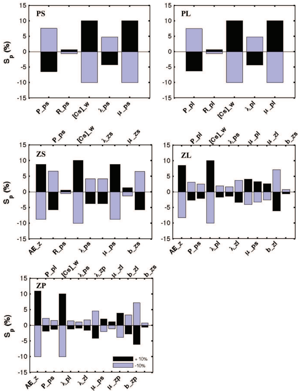
Figure 4. Sensitivity ( S_p ) of the estimated 137 Cs concentrations in different plankton groups (PS, PL, ZS, ZL, ZP) to a 10% change in the parameters of Eqs. (3) and (7). The S_p values are calculated using Eq. (8). Significance of parameters: P_ : primary production rate, R_ : phytoplankton respiration rate, [Cs]_w : 137 Cs concentration in seawater, \lambda_ : depuration rate, \mu_ : accumulation rate, AE_ : Assimilation efficiency, b : growth efficiency of zooplankton.
