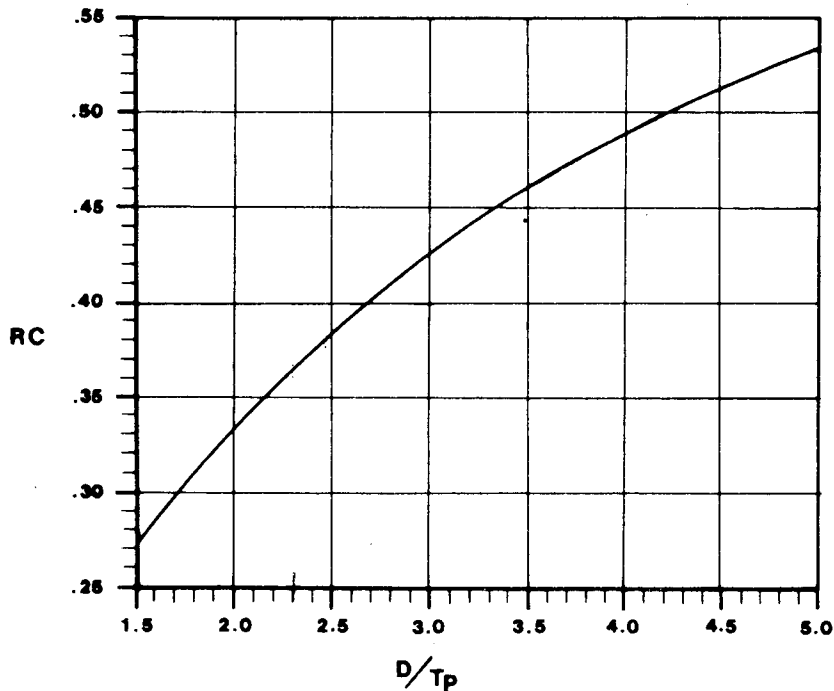
FIGURE 2 Graph of routing coefficient for use in "Rational" formula (based on triangular unit hydrograph and 75% winter rainfall profile)
