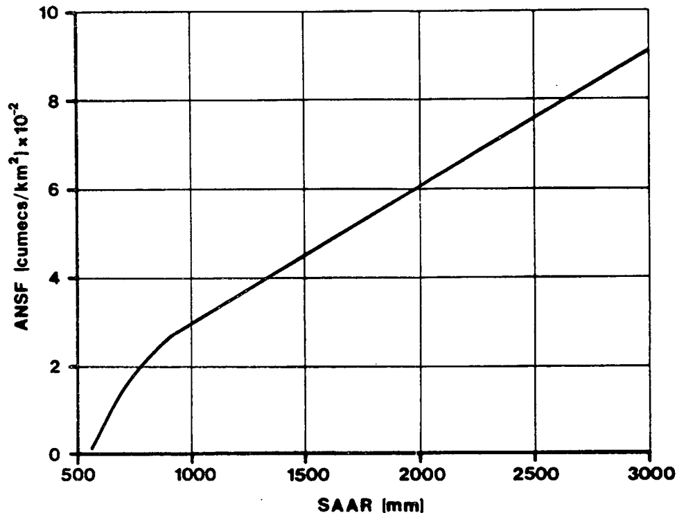
Figure 1. Graphical representation of ANSF-SAAR relationship for design use. (Applicable to T-year case but not PMF)
