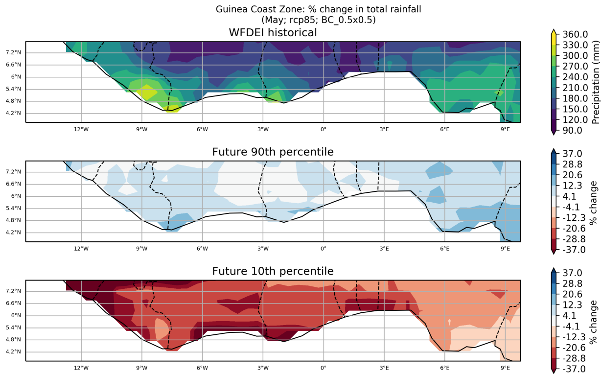
Figure 41: These maps show the ensemble spread in the percentage change in Total Rainfall for the period 2040 to 2059 (compared to a baseline period of 1950 - 2000) for the May season. They show the 90th and 10th percentiles of the distribution across the model ensemble, computed separately at each grid point, for the Guinea Coast Zone region. This particular plot shows the percentage change for the RCP8.5 scenario.
