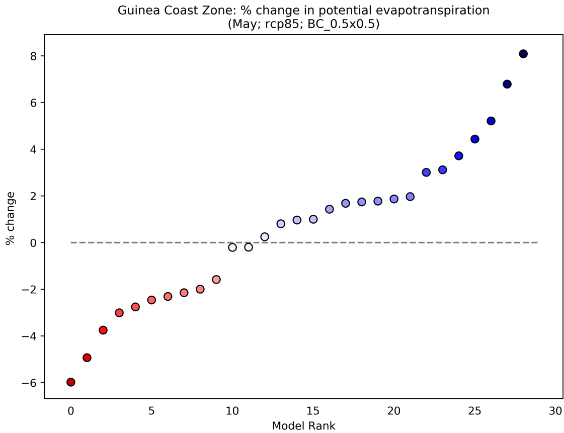
Figure 4: This scatterplot shows the percentage change in Potential Evapotranspiration for the period 2040 to 2059 (compared to a baseline period of 1950 - 2000) for the May season. Each data point shows an individual model averaged over Guinea Coast Zone, and ranked according to the magnitude of the value on the y-axis. This particular plot shows the percentage change for the RCP8.5 scenario.
