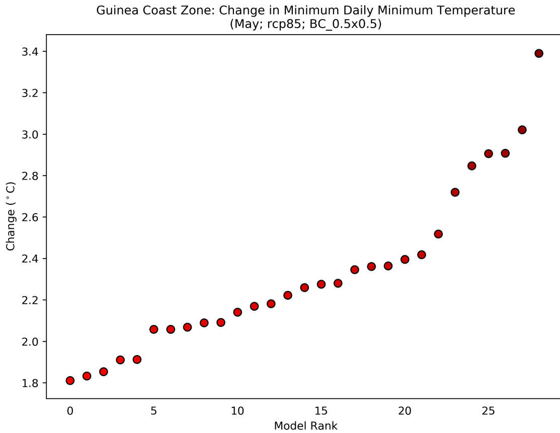
Figure 40: This scatterplot shows the absolute change in Minimum Daily Minimum Temperature for the period 2040 to 2059 (compared to a baseline period of 1950 - 2000) for the May season. Each data point shows an individual model averaged over Guinea Coast Zone, and ranked according to the magnitude of the value on the y-axis. This particular plot shows the absolute change for the RCP8.5 scenario.
