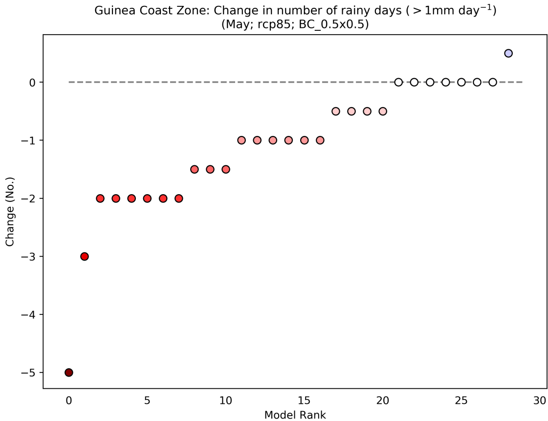
Figure 67: This scatterplot shows the absolute change in Number of Rainy Days ( >1\text{mm day}^{-1} ) for the period 2040 to 2059 (compared to a baseline period of 1950 - 2000) for the May season. Each data point shows an individual model averaged over Guinea Coast Zone, and ranked according to the magnitude of the value on the y-axis. This particular plot shows the absolute change for the RCP8.5 scenario.
