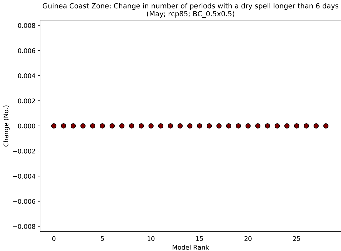
Figure 24: This scatterplot shows the absolute change in Number of Periods with a Dry Spell Longer Than 6 Days for the period 2040 to 2059 (compared to a baseline period of 1950 - 2000) for the May season. Each data point shows an individual model averaged over Guinea Coast Zone, and ranked according to the magnitude of the value on the y-axis. This particular plot shows the absolute change for the RCP8.5 scenario.
