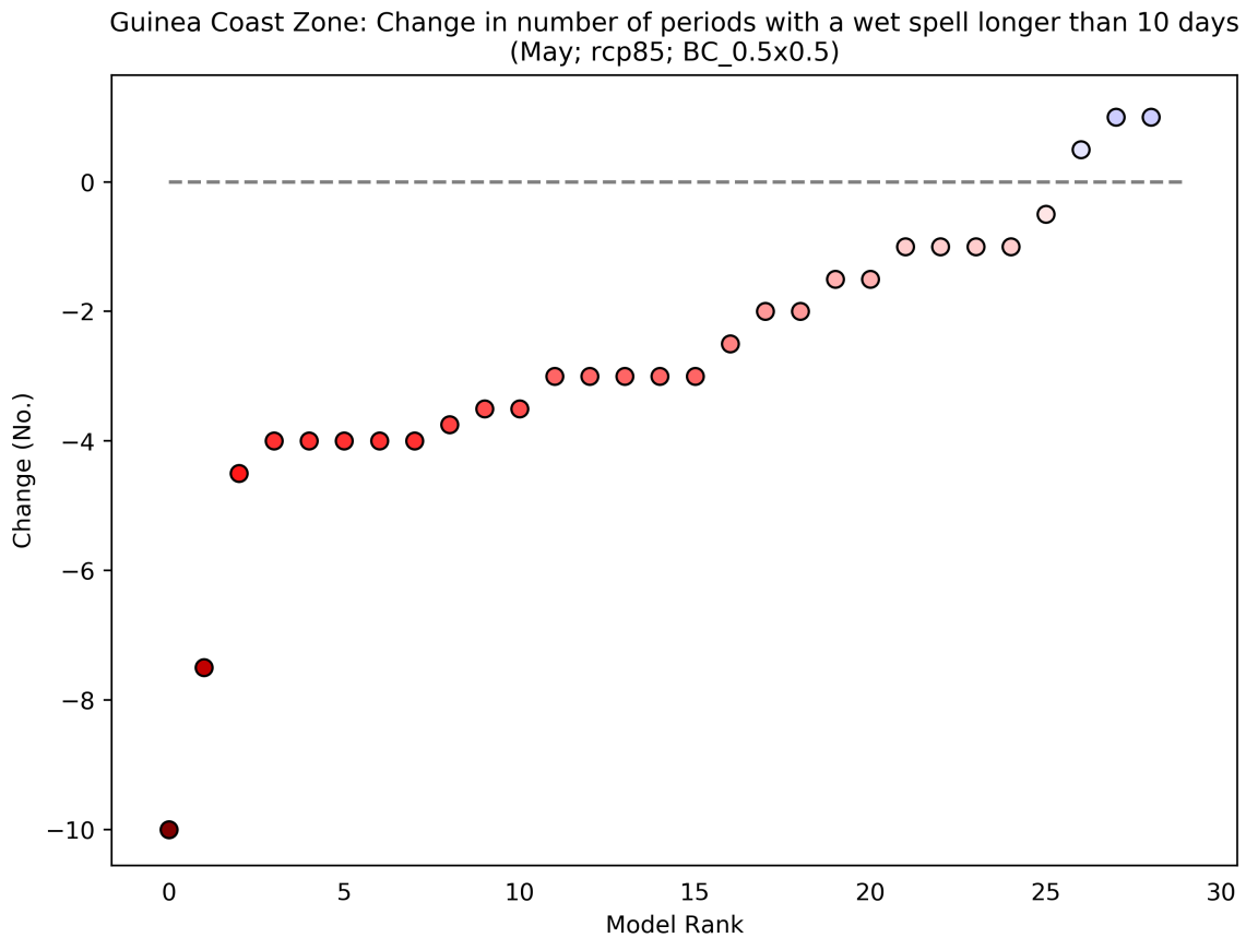
Figure 20: This scatterplot shows the absolute change in Number of Periods with a Wet Spell Longer Than 10 Days for the period 2040 to 2059 (compared to a baseline period of 1950 - 2000) for the May season. Each data point shows an individual model averaged over Guinea Coast Zone, and ranked according to the magnitude of the value on the y-axis. This particular plot shows the absolute change for the RCP8.5 scenario.
