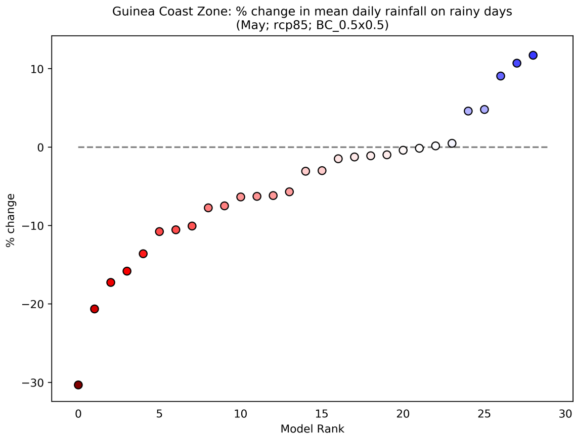
Figure 56: This scatterplot shows the percentage change in Mean Daily Rainfall on Rainy Days for the period 2040 to 2059 (compared to a baseline period of 1950 - 2000) for the May season. Each data point shows an individual model averaged over Guinea Coast Zone, and ranked according to the magnitude of the value on the y-axis. This particular plot shows the percentage change for the RCP8.5 scenario.
