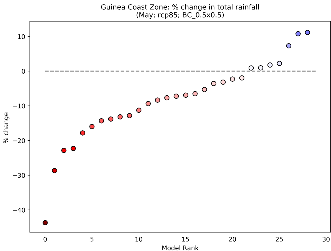
Figure 44: This scatterplot shows the percentage change in Total Rainfall for the period 2040 to 2059 (compared to a baseline period of 1950 - 2000) for the May season. Each data point shows an individual model averaged over Guinea Coast Zone, and ranked according to the magnitude of the value on the y-axis. This particular plot shows the percentage change for the RCP8.5 scenario.
