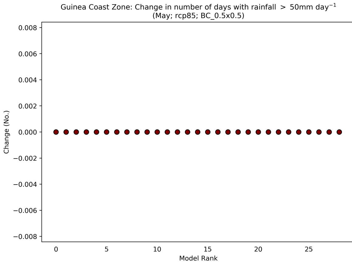
Figure 79: This scatterplot shows the absolute change in Number of Days with Rainfall > 50mm day -1 for the period 2040 to 2059 (compared to a baseline period of 1950 - 2000) for the May season. Each data point shows an individual model averaged over Guinea Coast Zone, and ranked according to the magnitude of the value on the y-axis. This particular plot shows the absolute change for the RCP8.5 scenario.
