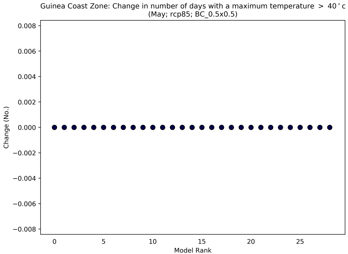
Figure 71: This scatterplot shows the absolute change in Number of Days with a Maximum Temperature > 40°C for the period 2040 to 2059 (compared to a baseline period of 1950 - 2000) for the May season. Each data point shows an individual model averaged over Guinea Coast Zone, and ranked according to the magnitude of the value on the y-axis. This particular plot shows the absolute change for the RCP8.5 scenario.
