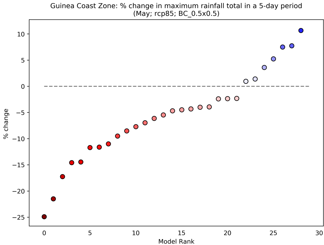
Figure 83: This scatterplot shows the percentage change in Maximum Rainfall Total in a 5-day Period for the period 2040 to 2059 (compared to a baseline period of 1950 - 2000) for the May season. Each data point shows an individual model averaged over Guinea Coast Zone, and ranked according to the magnitude of the value on the y-axis. This particular plot shows the percentage change for the RCP8.5 scenario.
