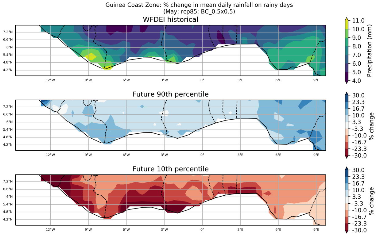
Figure 53: These maps show the ensemble spread in the percentage change in Mean Daily Rainfall on Rainy Days for the period 2040 to 2059 (compared to a baseline period of 1950 - 2000) for the May season. They show the 90th and 10th percentiles of the distribution across the model ensemble, computed separately at each grid point, for the Guinea Coast Zone region. This particular plot shows the percentage change for the RCP8.5 scenario.
