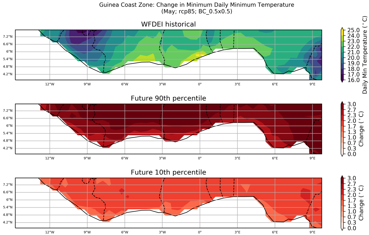
Figure 37: These maps show the ensemble spread in the absolute change in Minimum Daily Minimum Temperature for the period 2040 to 2059 (compared to a baseline period of 1950 - 2000) for the May season. They show the 90th and 10th percentiles of the distribution across the model ensemble, computed separately at each grid point, for the Guinea Coast Zone region. This particular plot shows the absolute change for the RCP8.5 scenario.
