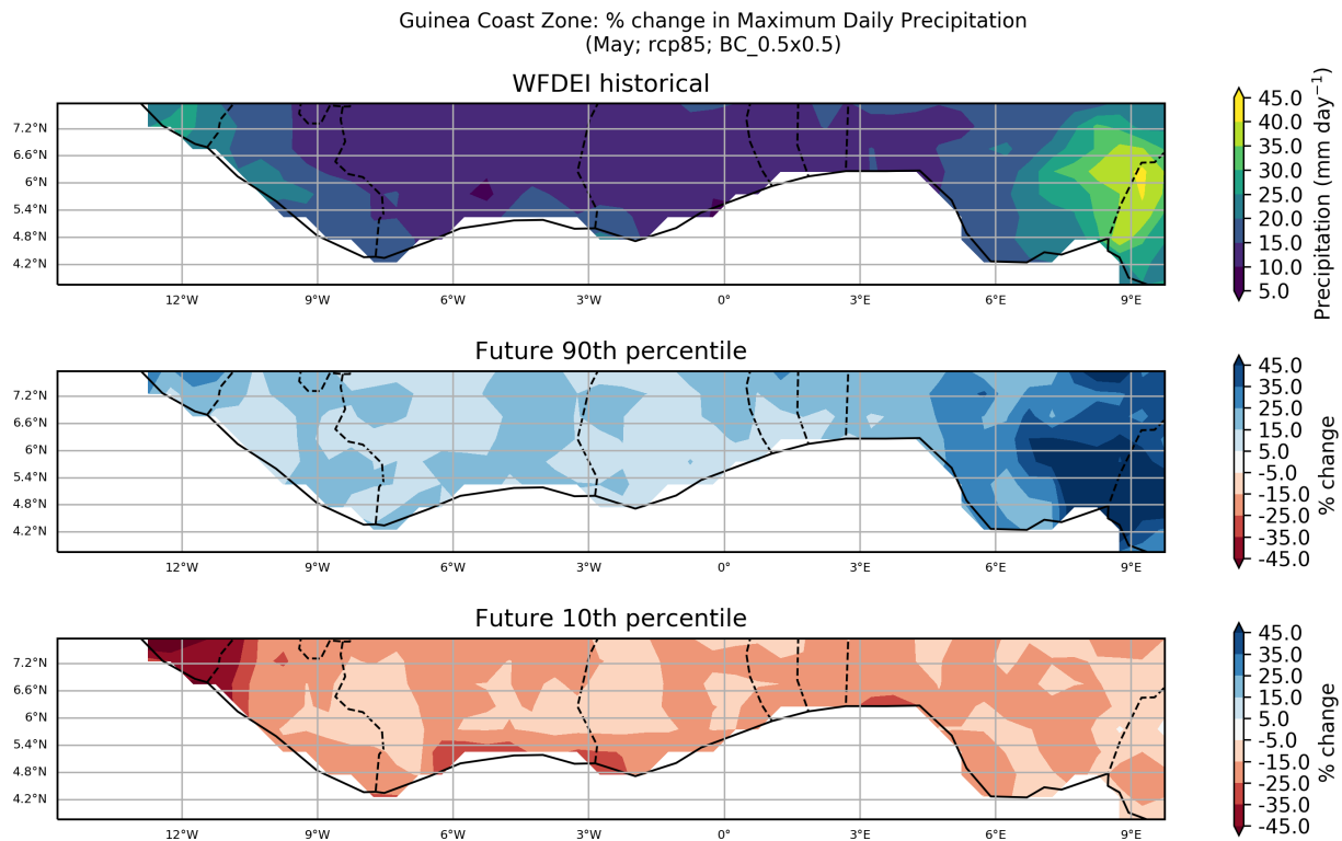
Figure 25: These maps show the ensemble spread in the percentage change in Maximum Daily Precipitation for the period 2040 to 2059 (compared to a baseline period of 1950 - 2000) for the May season. They show the 90th and 10th percentiles of the distribution across the model ensemble, computed separately at each grid point, for the Guinea Coast Zone region. This particular plot shows the percentage change for the RCP8.5 scenario.
