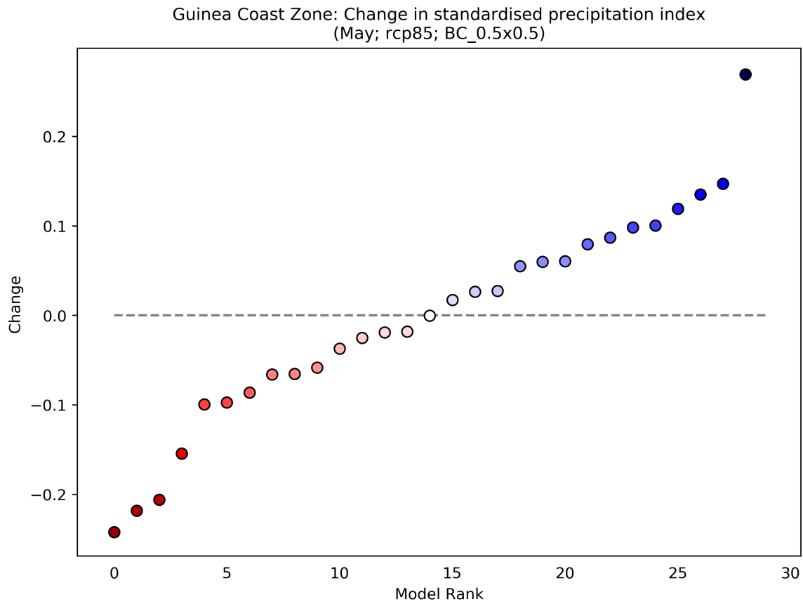
Figure 12: This scatterplot shows the absolute change in Standardised Precipitation Index for the period 2040 to 2059 (compared to a baseline period of 1950 - 2000) for the May season. Each data point shows an individual model averaged over Guinea Coast Zone, and ranked according to the magnitude of the value on the y-axis. This particular plot shows the absolute change for the RCP8.5 scenario.
