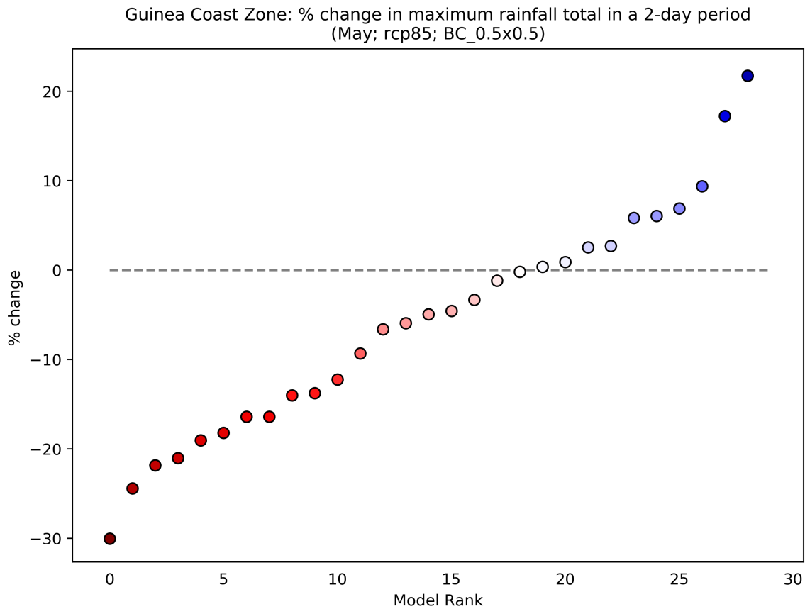
Figure 91: This scatterplot shows the percentage change in Maximum Rainfall Total in a 2-day Period for the period 2040 to 2059 (compared to a baseline period of 1950 - 2000) for the May season. Each data point shows an individual model averaged over Guinea Coast Zone, and ranked according to the magnitude of the value on the y-axis. This particular plot shows the percentage change for the RCP8.5 scenario.
