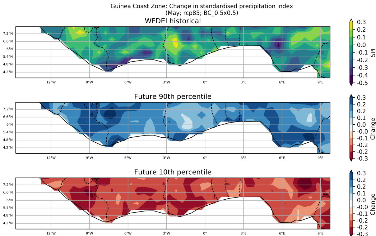
Figure 9: These maps show the ensemble spread in the absolute change in Standardised Precipitation Index for the period 2040 to 2059 (compared to a baseline period of 1950 - 2000) for the May season. They show the 90th and 10th percentiles of the distribution across the model ensemble, computed separately at each grid point, for the Guinea Coast Zone region. This particular plot shows the absolute change for the RCP8.5 scenario.
