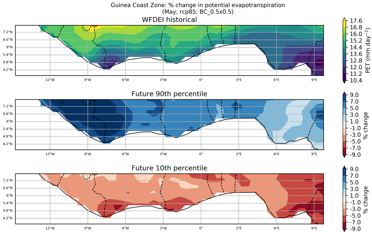
Figure 1: These maps show the ensemble spread in the percentage change in Potential Evapotranspiration for the period 2040 to 2059 (compared to a baseline period of 1950 - 2000) for the May season. They show the 90th and 10th percentiles of the distribution across the model ensemble, computed separately at each grid point, for the Guinea Coast Zone region. This particular plot shows the percentage change for the RCP8.5 scenario.
