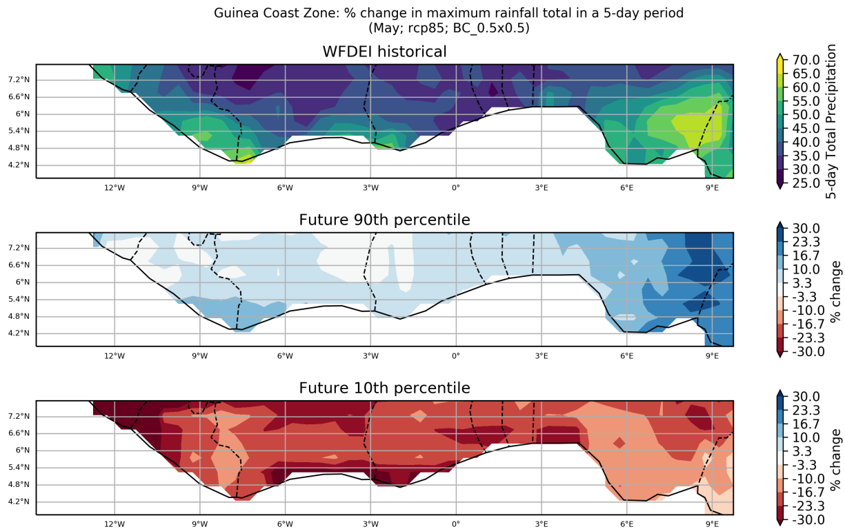
Figure 80: These maps show the ensemble spread in the percentage change in Maximum Rainfall Total in a 5-day Period for the period 2040 to 2059 (compared to a baseline period of 1950 - 2000) for the May season. They show the 90th and 10th percentiles of the distribution across the model ensemble, computed separately at each grid point, for the Guinea Coast Zone region. This particular plot shows the percentage change for the RCP8.5 scenario.
