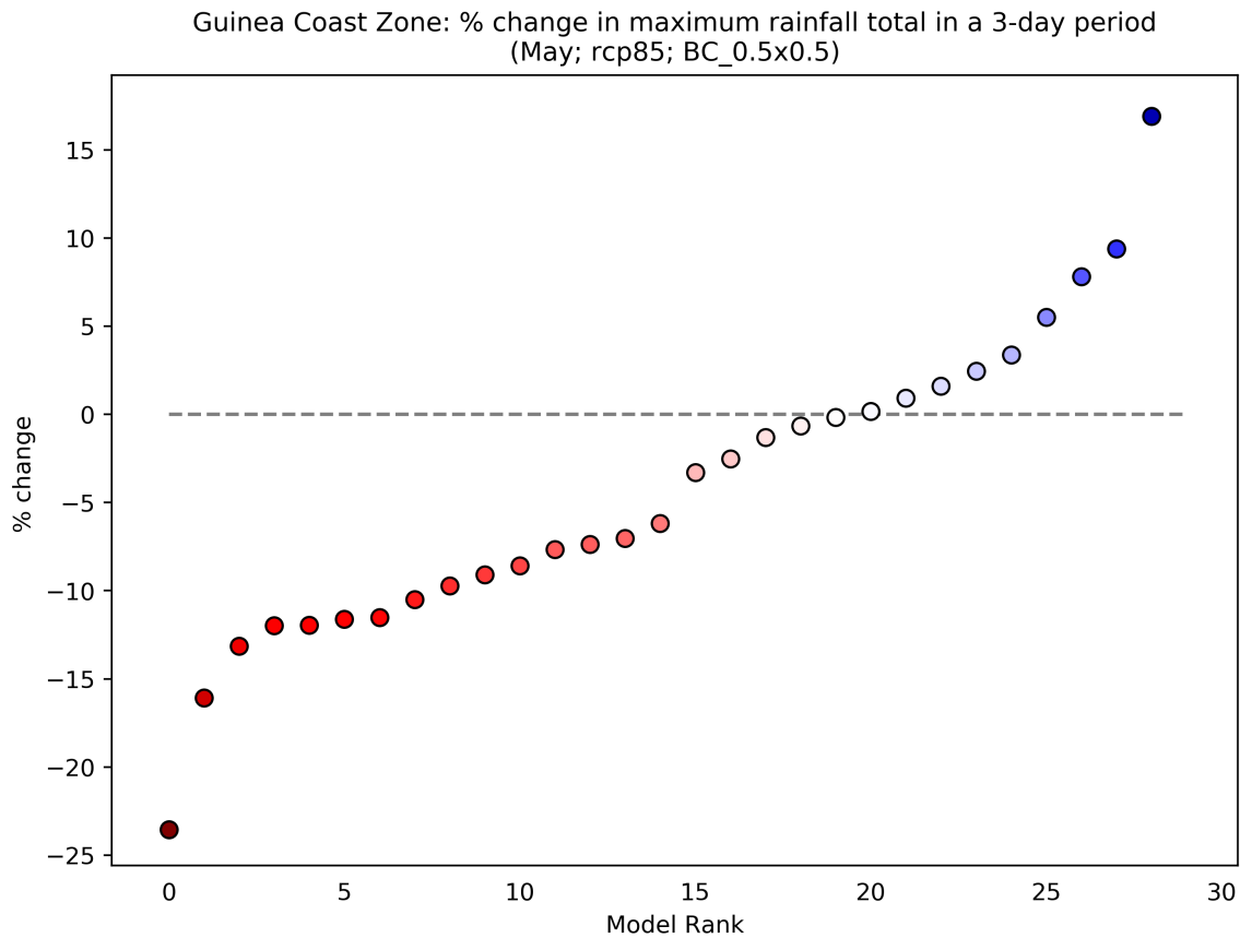
Figure 87: This scatterplot shows the percentage change in Maximum Rainfall Total in a 3-day Period for the period 2040 to 2059 (compared to a baseline period of 1950 - 2000) for the May season. Each data point shows an individual model averaged over Guinea Coast Zone, and ranked according to the magnitude of the value on the y-axis. This particular plot shows the percentage change for the RCP8.5 scenario.
