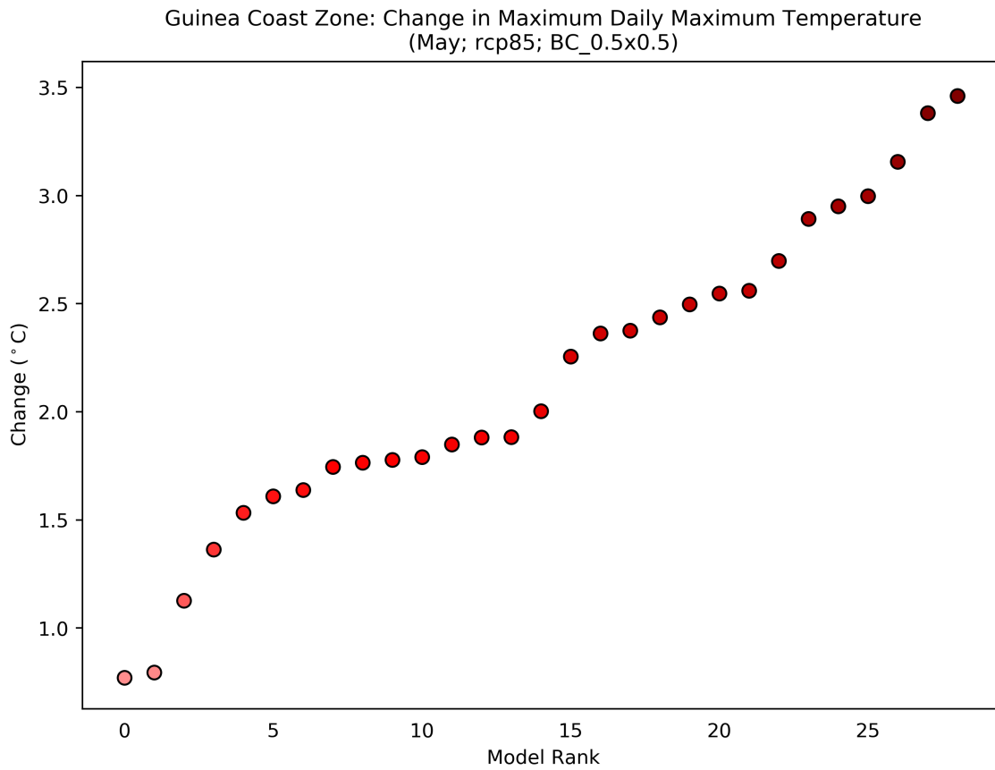
Figure 32: This scatterplot shows the absolute change in Maximum Daily Maximum Temperature for the period 2040 to 2059 (compared to a baseline period of 1950 - 2000) for the May season. Each data point shows an individual model averaged over Guinea Coast Zone, and ranked according to the magnitude of the value on the y-axis. This particular plot shows the absolute change for the RCP8.5 scenario.
