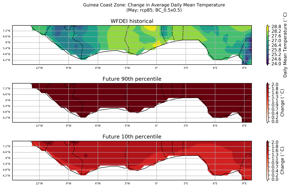
Figure 45: These maps show the ensemble spread in the absolute change in Average Daily Mean Temperature for the period 2040 to 2059 (compared to a baseline period of 1950 - 2000) for the May season. They show the 90th and 10th percentiles of the distribution across the model ensemble, computed separately at each grid point, for the Guinea Coast Zone region. This particular plot shows the absolute change for the RCP8.5 scenario.
