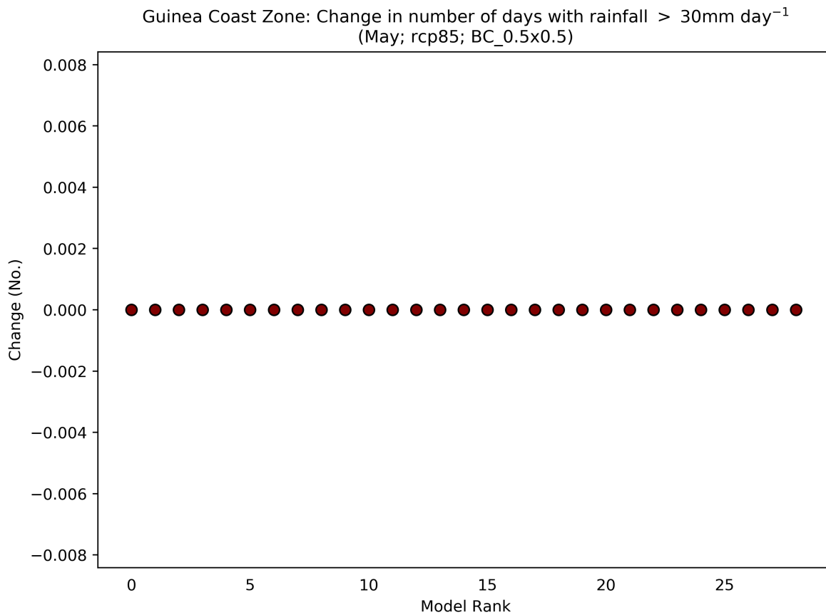
Figure 75: This scatterplot shows the absolute change in Number of Days with Rainfall > 30mm day -1 for the period 2040 to 2059 (compared to a baseline period of 1950 - 2000) for the May season. Each data point shows an individual model averaged over Guinea Coast Zone, and ranked according to the magnitude of the value on the y-axis. This particular plot shows the absolute change for the RCP8.5 scenario.
