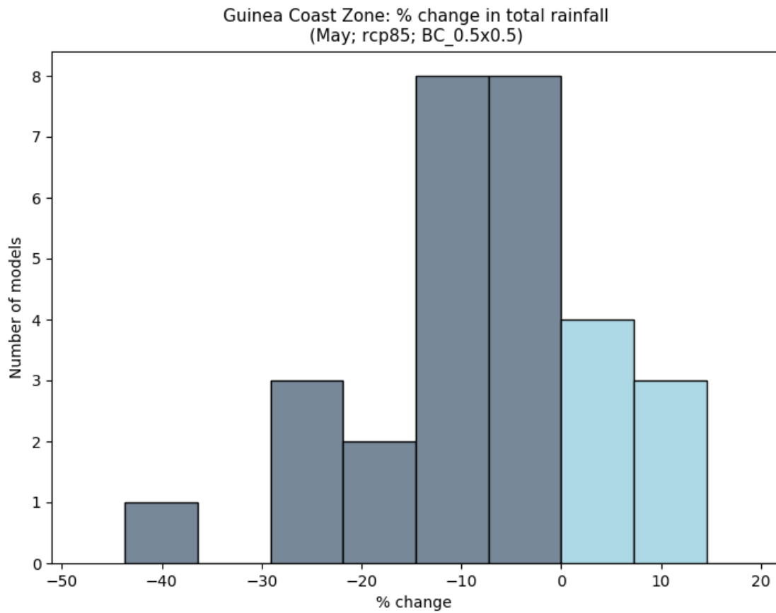
Figure 42: This histogram shows the number of models that agree on the percentage change in Total Rainfall for the period 2040 to 2059 (compared to a baseline period of 1950 - 2000) for the May season. Each vertical bar shows the number of models that agree on the range of values shown on the x-axis for the Guinea Coast Zone region. This particular plot shows the percentage change for the RCP8.5 scenario.
