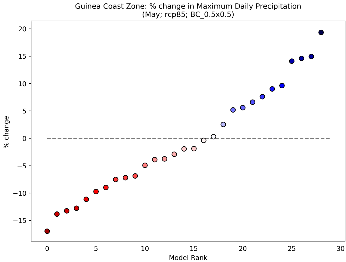
Figure 28: This scatterplot shows the percentage change in Maximum Daily Precipitation for the period 2040 to 2059 (compared to a baseline period of 1950 - 2000) for the May season. Each data point shows an individual model averaged over Guinea Coast Zone, and ranked according to the magnitude of the value on the y-axis. This particular plot shows the percentage change for the RCP8.5 scenario.
