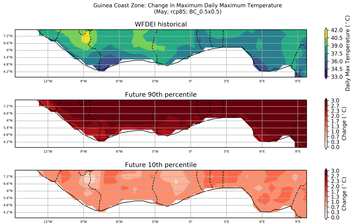
Figure 29: These maps show the ensemble spread in the absolute change in Maximum Daily Maximum Temperature for the period 2040 to 2059 (compared to a baseline period of 1950 - 2000) for the May season. They show the 90th and 10th percentiles of the distribution across the model ensemble, computed separately at each grid point, for the Guinea Coast Zone region. This particular plot shows the absolute change for the RCP8.5 scenario.
