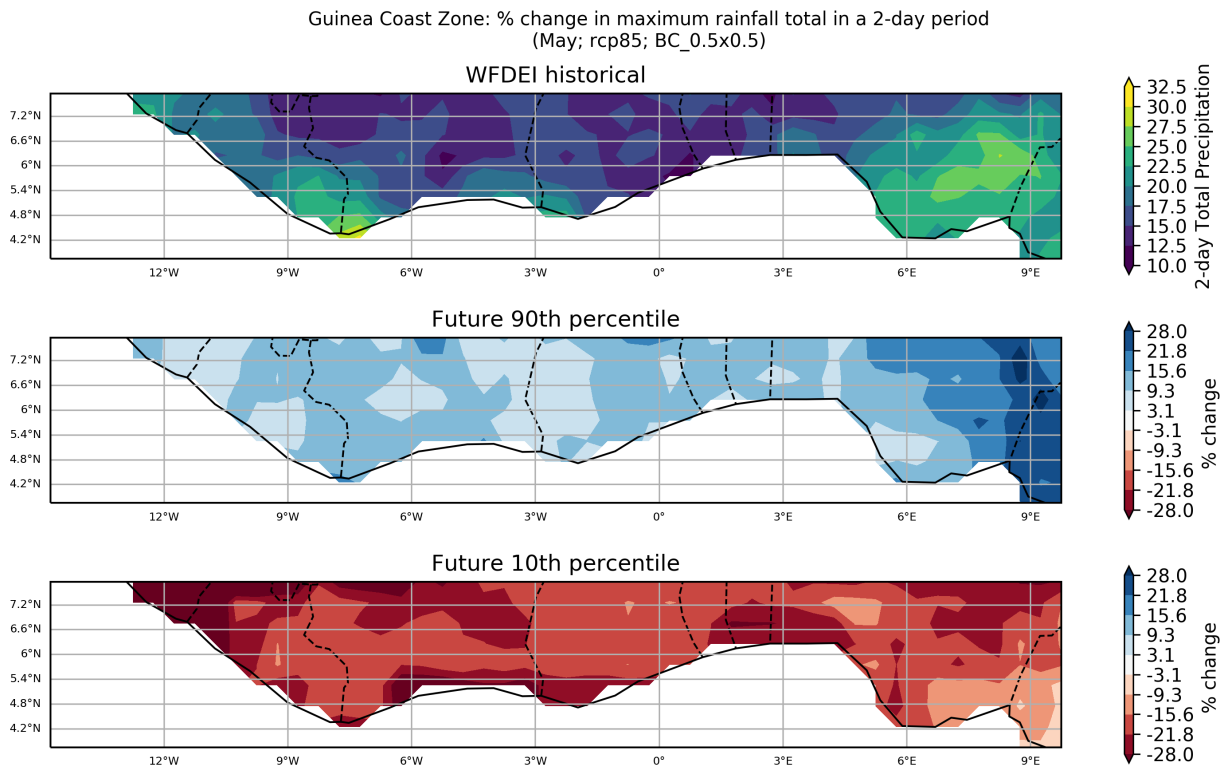
Figure 88: These maps show the ensemble spread in the percentage change in Maximum Rainfall Total in a 2-day Period for the period 2040 to 2059 (compared to a baseline period of 1950 - 2000) for the May season. They show the 90th and 10th percentiles of the distribution across the model ensemble, computed separately at each grid point, for the Guinea Coast Zone region. This particular plot shows the percentage change for the RCP8.5 scenario.
