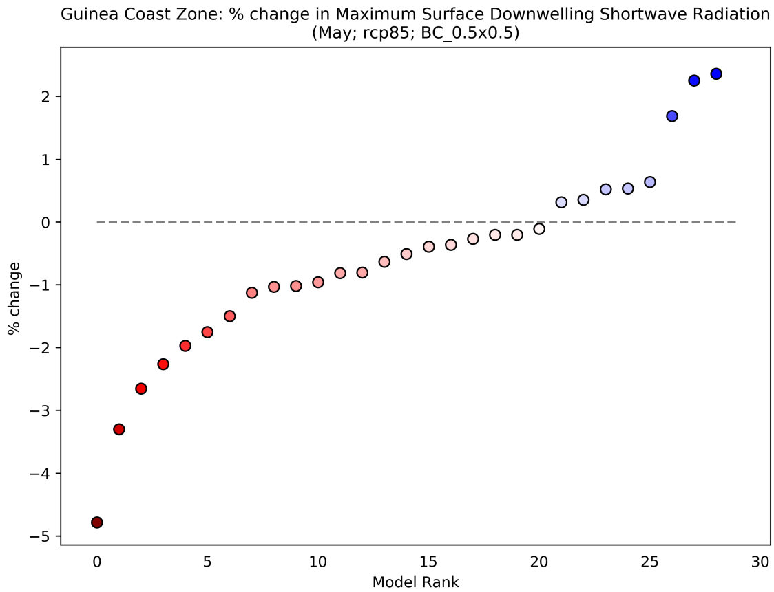
Figure 36: This scatterplot shows the percentage change in Maximum Surface Downwelling Shortwave Radiation for the period 2040 to 2059 (compared to a baseline period of 1950 - 2000) for the May season. Each data point shows an individual model averaged over Guinea Coast Zone, and ranked according to the magnitude of the value on the y-axis. This particular plot shows the percentage change for the RCP8.5 scenario.
