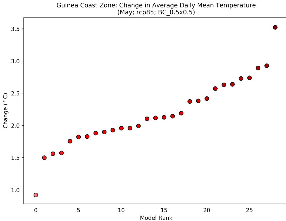
Figure 48: This scatterplot shows the absolute change in Average Daily Mean Temperature for the period 2040 to 2059 (compared to a baseline period of 1950 - 2000) for the May season. Each data point shows an individual model averaged over Guinea Coast Zone, and ranked according to the magnitude of the value on the y-axis. This particular plot shows the absolute change for the RCP8.5 scenario.
