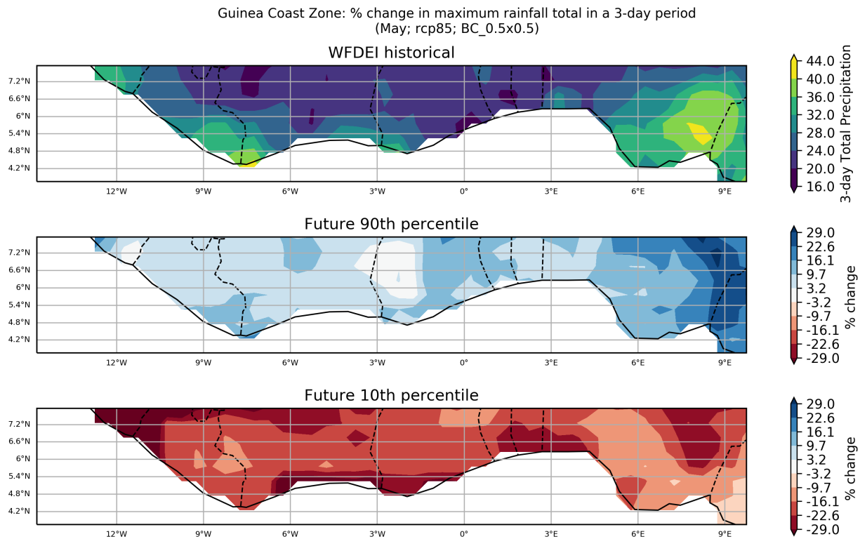
Figure 84: These maps show the ensemble spread in the percentage change in Maximum Rainfall Total in a 3-day Period for the period 2040 to 2059 (compared to a baseline period of 1950 - 2000) for the May season. They show the 90th and 10th percentiles of the distribution across the model ensemble, computed separately at each grid point, for the Guinea Coast Zone region. This particular plot shows the percentage change for the RCP8.5 scenario.
