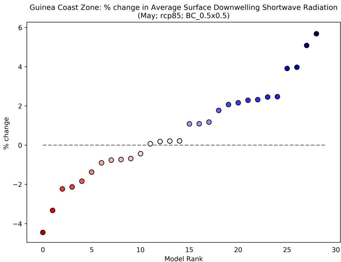
Figure 52: This scatterplot shows the percentage change in Average Surface Downwelling Shortwave Radiation for the period 2040 to 2059 (compared to a baseline period of 1950 - 2000) for the May season. Each data point shows an individual model averaged over Guinea Coast Zone, and ranked according to the magnitude of the value on the y-axis. This particular plot shows the percentage change for the RCP8.5 scenario.
