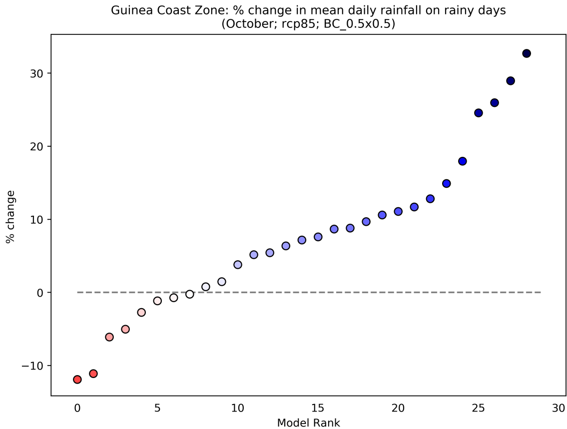
Figure 56: This scatterplot shows the percentage change in Mean Daily Rainfall on Rainy Days for the period 2040 to 2059 (compared to a baseline period of 1950 - 2000) for the October season. Each data point shows an individual model averaged over Guinea Coast Zone, and ranked according to the magnitude of the value on the y-axis. This particular plot shows the percentage change for the RCP8.5 scenario.
