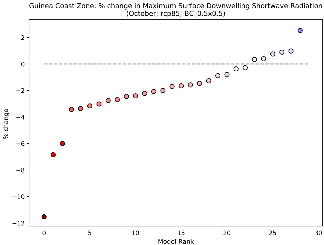
Figure 36: This scatterplot shows the percentage change in Maximum Surface Downwelling Shortwave Radiation for the period 2040 to 2059 (compared to a baseline period of 1950 - 2000) for the October season. Each data point shows an individual model averaged over Guinea Coast Zone, and ranked according to the magnitude of the value on the y-axis. This particular plot shows the percentage change for the RCP8.5 scenario.
