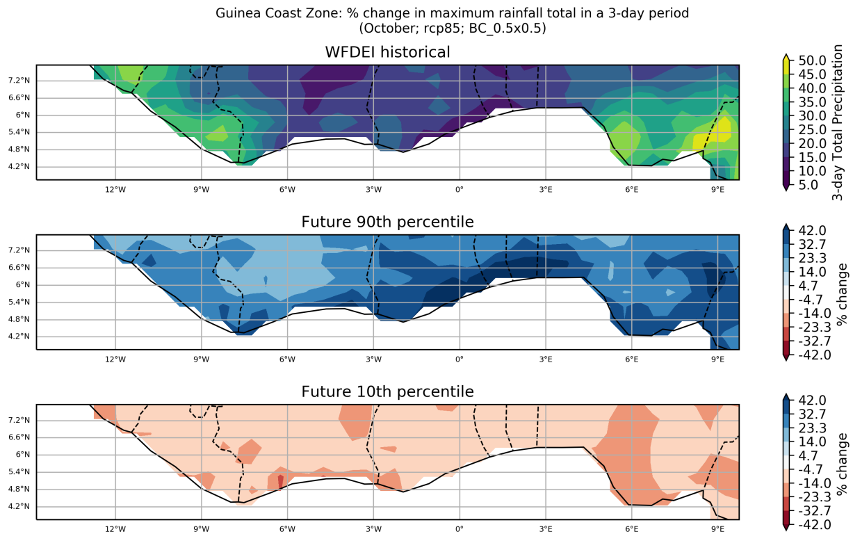
Figure 84: These maps show the ensemble spread in the percentage change in Maximum Rainfall Total in a 3-day Period for the period 2040 to 2059 (compared to a baseline period of 1950 - 2000) for the October season. They show the 90th and 10th percentiles of the distribution across the model ensemble, computed separately at each grid point, for the Guinea Coast Zone region. This particular plot shows the percentage change for the RCP8.5 scenario.
