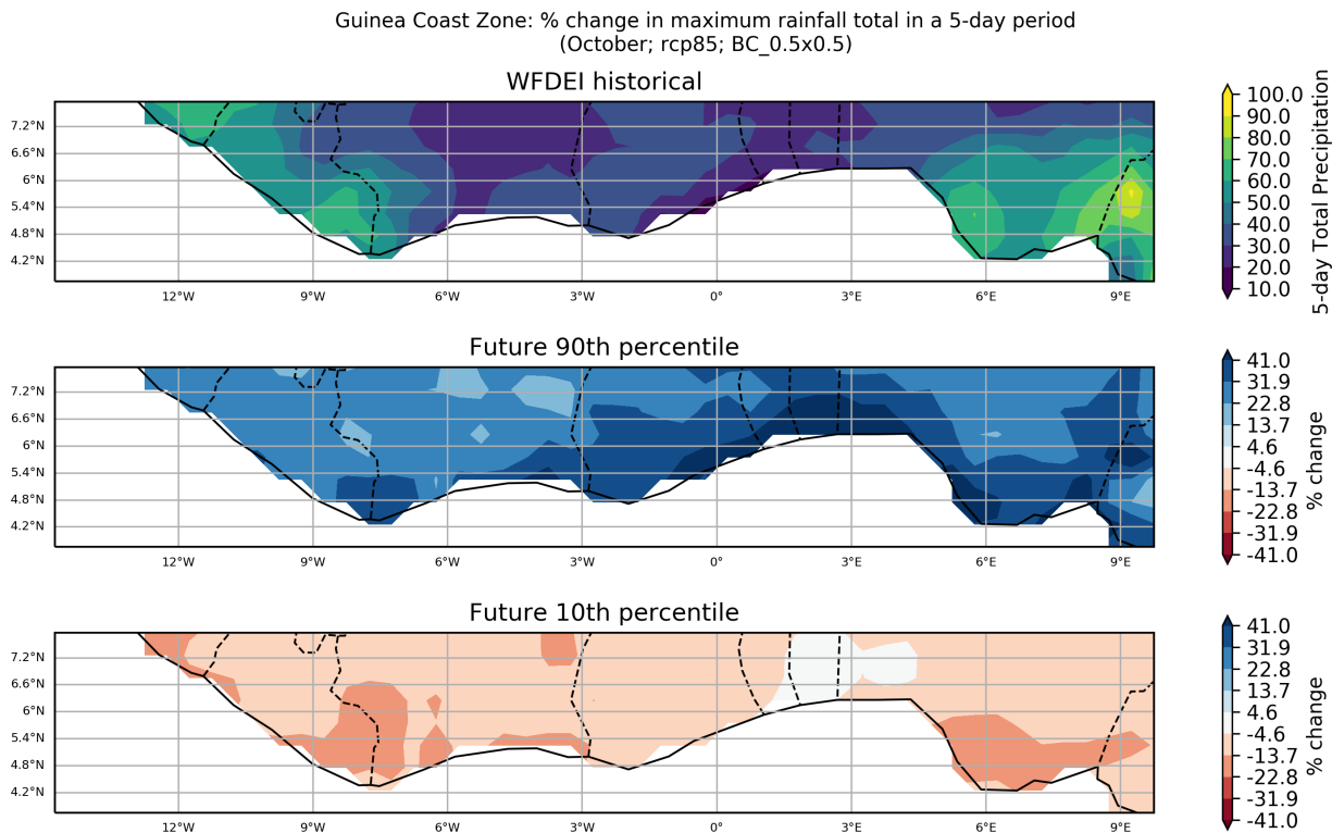
Figure 80: These maps show the ensemble spread in the percentage change in Maximum Rainfall Total in a 5-day Period for the period 2040 to 2059 (compared to a baseline period of 1950 - 2000) for the October season. They show the 90th and 10th percentiles of the distribution across the model ensemble, computed separately at each grid point, for the Guinea Coast Zone region. This particular plot shows the percentage change for the RCP8.5 scenario.
