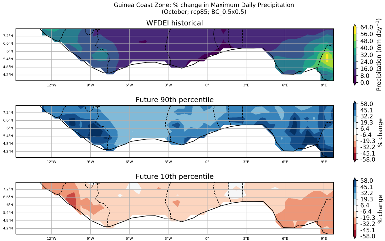
Figure 25: These maps show the ensemble spread in the percentage change in Maximum Daily Precipitation for the period 2040 to 2059 (compared to a baseline period of 1950 - 2000) for the October season. They show the 90th and 10th percentiles of the distribution across the model ensemble, computed separately at each grid point, for the Guinea Coast Zone region. This particular plot shows the percentage change for the RCP8.5 scenario.
