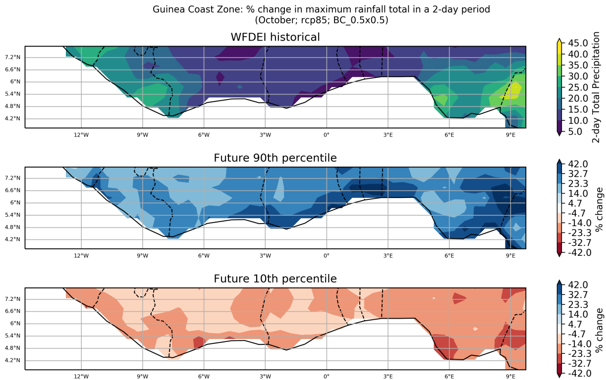
Figure 88: These maps show the ensemble spread in the percentage change in Maximum Rainfall Total in a 2-day Period for the period 2040 to 2059 (compared to a baseline period of 1950 - 2000) for the October season. They show the 90th and 10th percentiles of the distribution across the model ensemble, computed separately at each grid point, for the Guinea Coast Zone region. This particular plot shows the percentage change for the RCP8.5 scenario.
