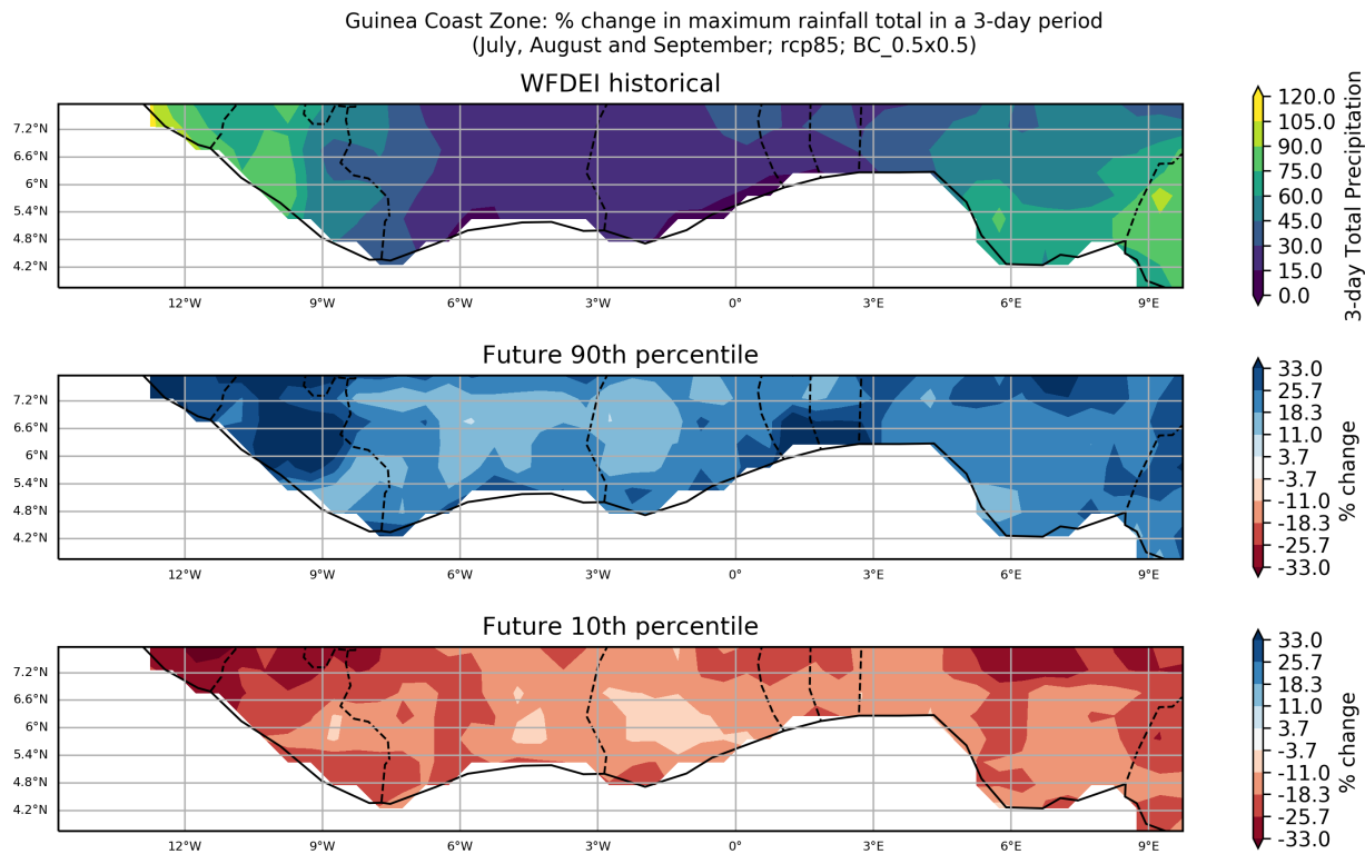
Figure 84: These maps show the ensemble spread in the percentage change in Maximum Rainfall Total in a 3-day Period for the period 2040 to 2059 (compared to a baseline period of 1950 - 2000) for the July, August and September season. They show the 90th and 10th percentiles of the distribution across the model ensemble, computed separately at each grid point, for the Guinea Coast Zone region. This particular plot shows the percentage change for the RCP8.5 scenario.
