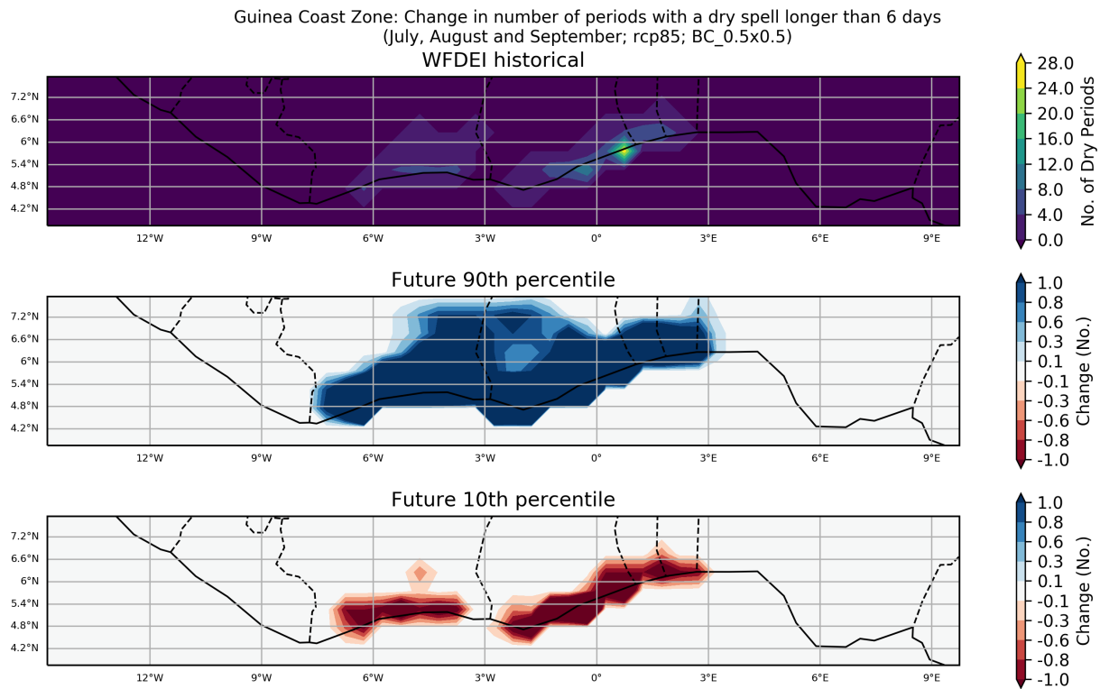
Figure 21: These maps show the ensemble spread in the absolute change in Number of Periods with a Dry Spell Longer Than 6 Days for the period 2040 to 2059 (compared to a baseline period of 1950 - 2000) for the July, August and September season. They show the 90th and 10th percentiles of the distribution across the model ensemble, computed separately at each grid point, for the Guinea Coast Zone region. This particular plot shows the absolute change for the RCP8.5 scenario.
