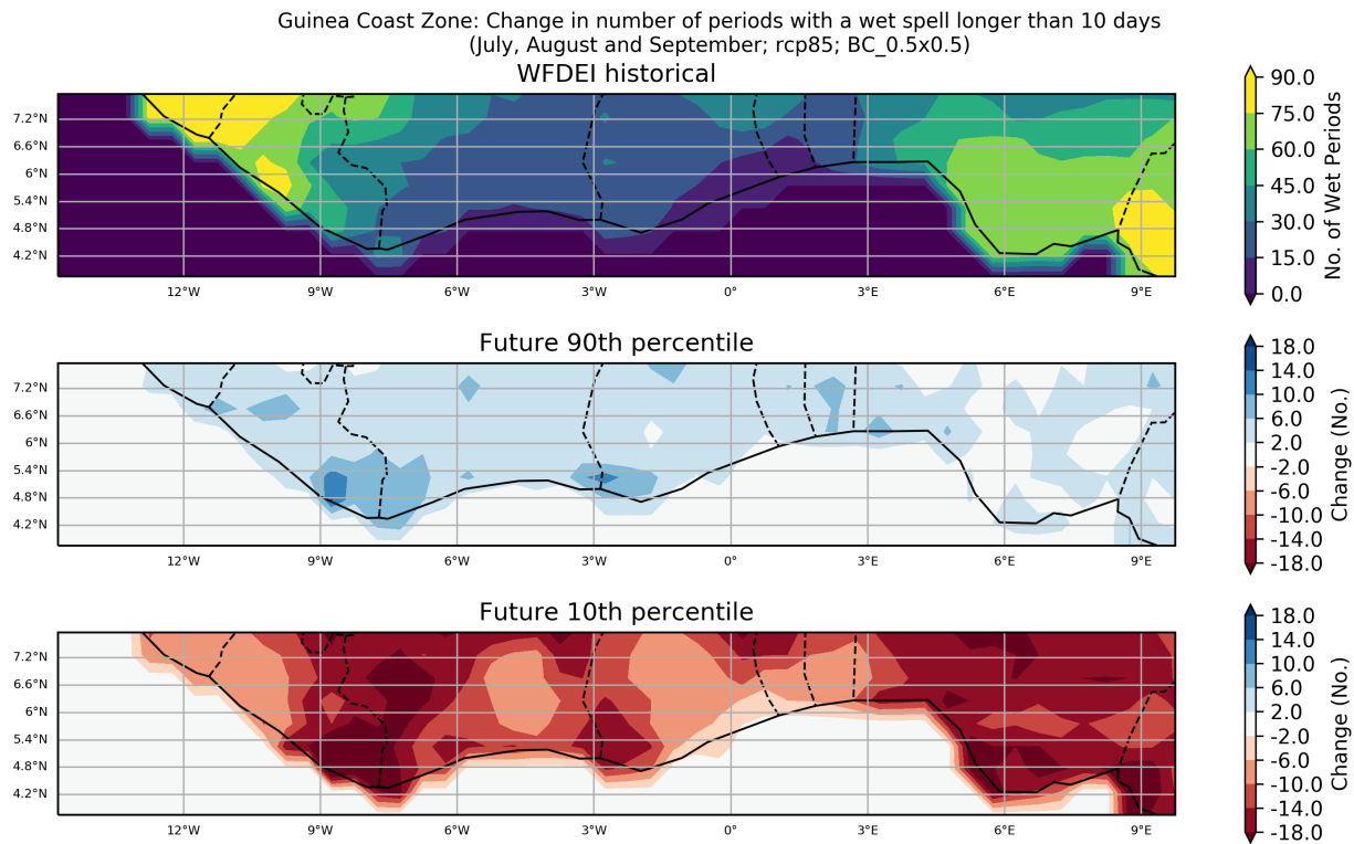
Figure 17: These maps show the ensemble spread in the absolute change in Number of Periods with a Wet Spell Longer Than 10 Days for the period 2040 to 2059 (compared to a baseline period of 1950 - 2000) for the July, August and September season. They show the 90th and 10th percentiles of the distribution across the model ensemble, computed separately at each grid point, for the Guinea Coast Zone region. This particular plot shows the absolute change for the RCP8.5 scenario.
