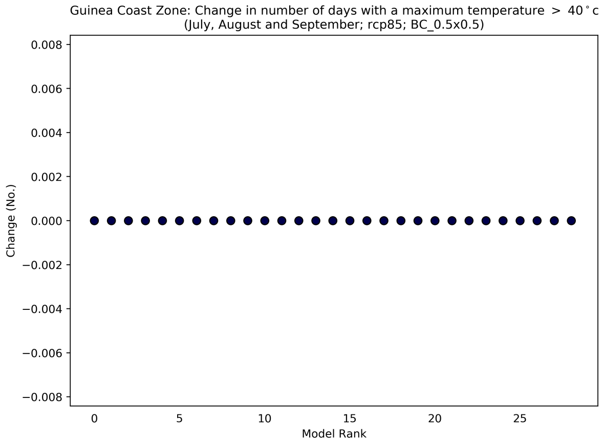
Figure 71: This scatterplot shows the absolute change in Number of Days with a Maximum Temperature > 40°C for the period 2040 to 2059 (compared to a baseline period of 1950 - 2000) for the July, August and September season. Each data point shows an individual model averaged over Guinea Coast Zone, and ranked according to the magnitude of the value on the y-axis. This particular plot shows the absolute change for the RCP8.5 scenario.
