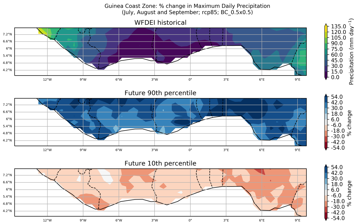
Figure 25: These maps show the ensemble spread in the percentage change in Maximum Daily Precipitation for the period 2040 to 2059 (compared to a baseline period of 1950 - 2000) for the July, August and September season. They show the 90th and 10th percentiles of the distribution across the model ensemble, computed separately at each grid point, for the Guinea Coast Zone region. This particular plot shows the percentage change for the RCP8.5 scenario.
