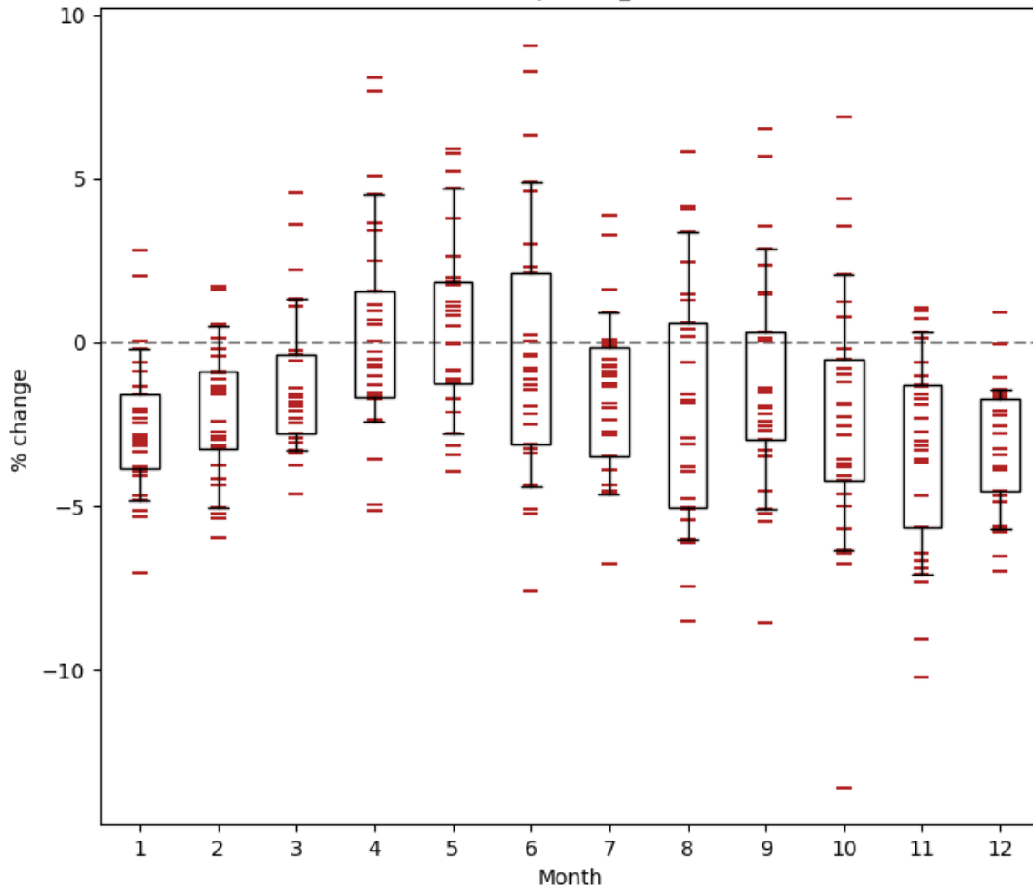
Guinea Coast Zone: % change in Monthly Climatological Mean Surface Downwelling Shortwave Radiation (Annual; rcp85; BC_0.5x0.5)
