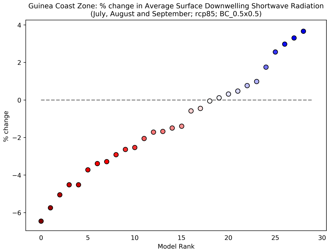
Figure 52: This scatterplot shows the percentage change in Average Surface Downwelling Shortwave Radiation for the period 2040 to 2059 (compared to a baseline period of 1950 - 2000) for the July, August and September season. Each data point shows an individual model averaged over Guinea Coast Zone, and ranked according to the magnitude of the value on the y-axis. This particular plot shows the percentage change for the RCP8.5 scenario.
