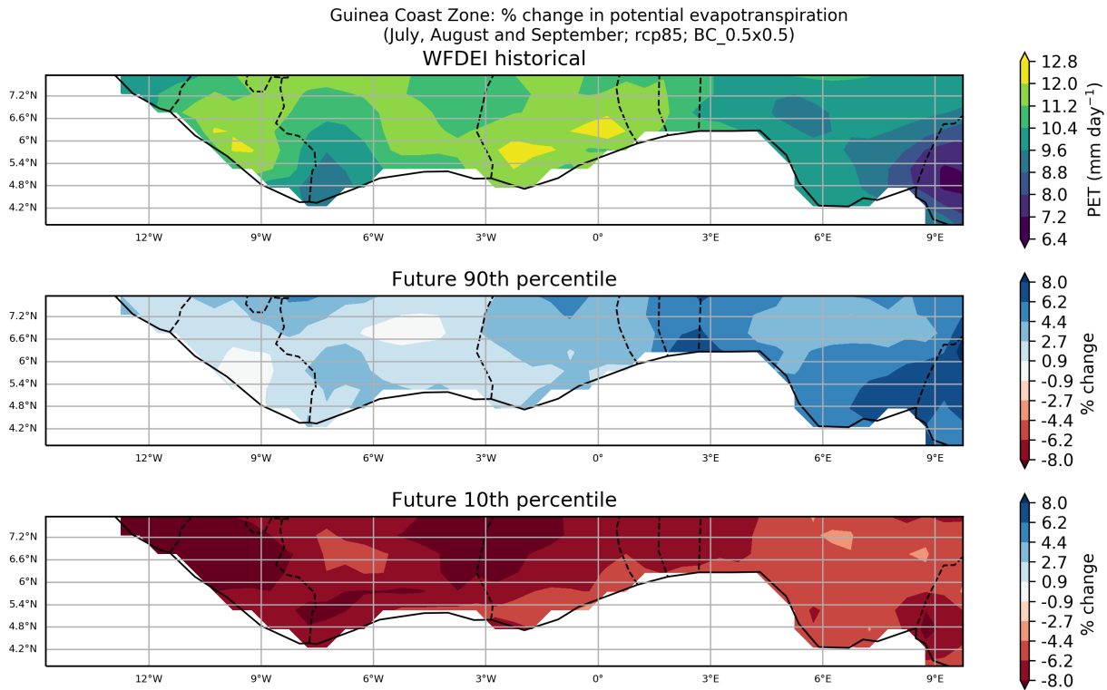
Figure 1: These maps show the ensemble spread in the percentage change in Potential Evapotranspiration for the period 2040 to 2059 (compared to a baseline period of 1950 - 2000) for the July, August and September season. They show the 90th and 10th percentiles of the distribution across the model ensemble, computed separately at each grid point, for the Guinea Coast Zone region. This particular plot shows the percentage change for the RCP8.5 scenario.
