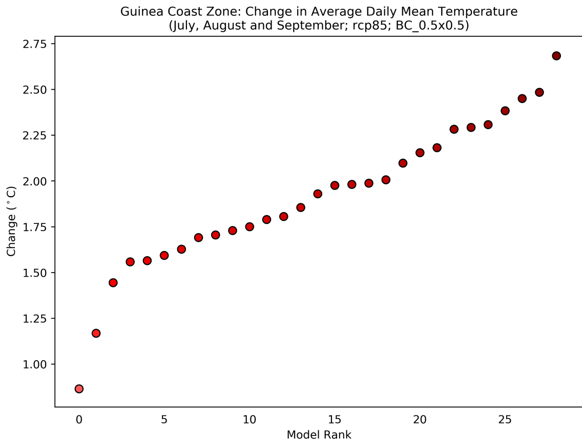
Figure 48: This scatterplot shows the absolute change in Average Daily Mean Temperature for the period 2040 to 2059 (compared to a baseline period of 1950 - 2000) for the July, August and September season. Each data point shows an individual model averaged over Guinea Coast Zone, and ranked according to the magnitude of the value on the y-axis. This particular plot shows the absolute change for the RCP8.5 scenario.
