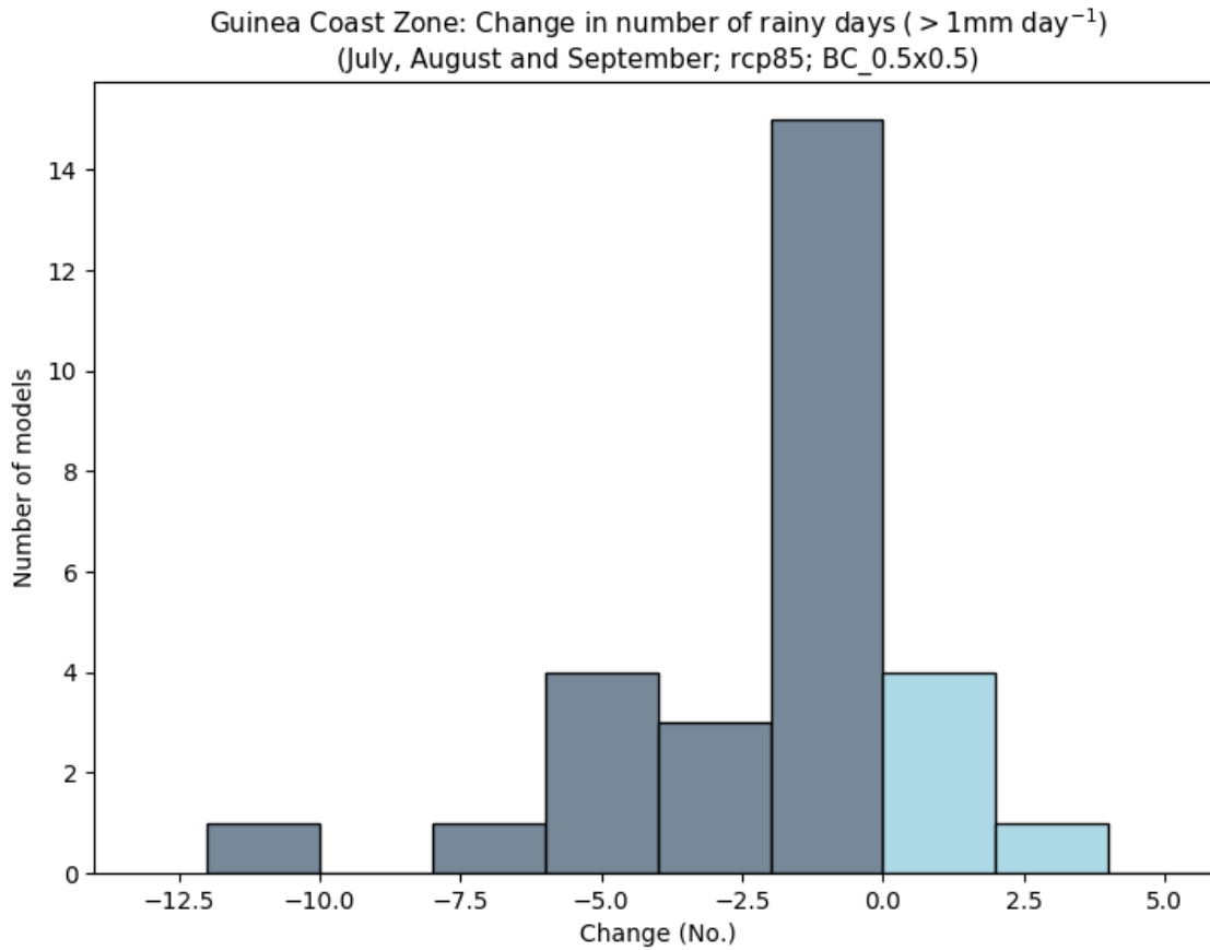
Figure 65: This histogram shows the number of models that agree on the absolute change in Number of Rainy Days ( > 1\text{mm day}^{-1} ) for the period 2040 to 2059 (compared to a baseline period of 1950 - 2000) for the July, August and September season. Each vertical bar shows the number of models that agree on the range of values shown on the x-axis for the Guinea Coast Zone region. This particular plot shows the absolute change for the RCP8.5 scenario.
