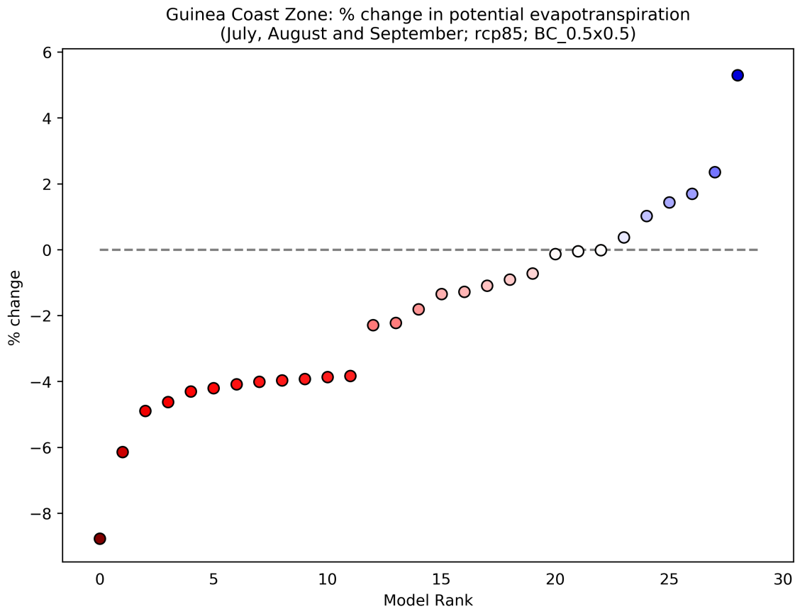
Figure 4: This scatterplot shows the percentage change in Potential Evapotranspiration for the period 2040 to 2059 (compared to a baseline period of 1950 - 2000) for the July, August and September season. Each data point shows an individual model averaged over Guinea Coast Zone, and ranked according to the magnitude of the value on the y-axis. This particular plot shows the percentage change for the RCP8.5 scenario.
