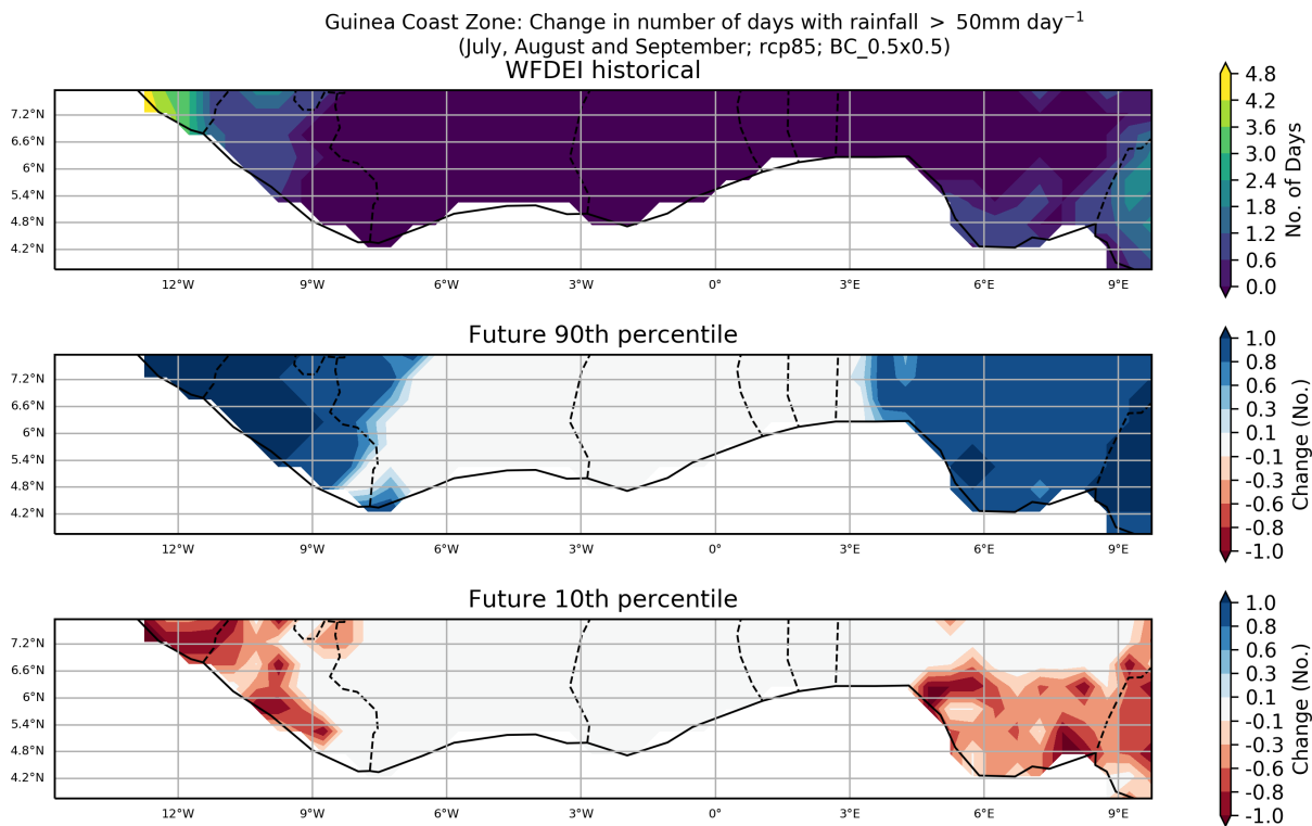
Figure 76: These maps show the ensemble spread in the absolute change in Number of Days with Rainfall > 50\text{mm day}^{-1} for the period 2040 to 2059 (compared to a baseline period of 1950 - 2000) for the July, August and September season. They show the 90th and 10th percentiles of the distribution across the model ensemble, computed separately at each grid point, for the Guinea Coast Zone region. This particular plot shows the absolute change for the RCP8.5 scenario.
