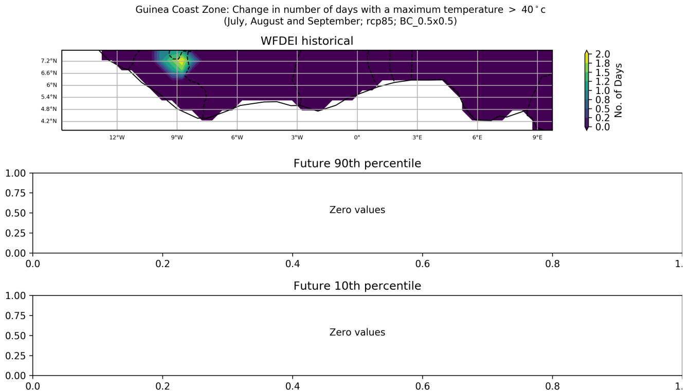
Figure 68: These maps show the ensemble spread in the absolute change in Number of Days with a Maximum Temperature > 40°C for the period 2040 to 2059 (compared to a baseline period of 1950 - 2000) for the July, August and September season. They show the 90th and 10th percentiles of the distribution across the model ensemble, computed separately at each grid point, for the Guinea Coast Zone region. This particular plot shows the absolute change for the RCP8.5 scenario.
