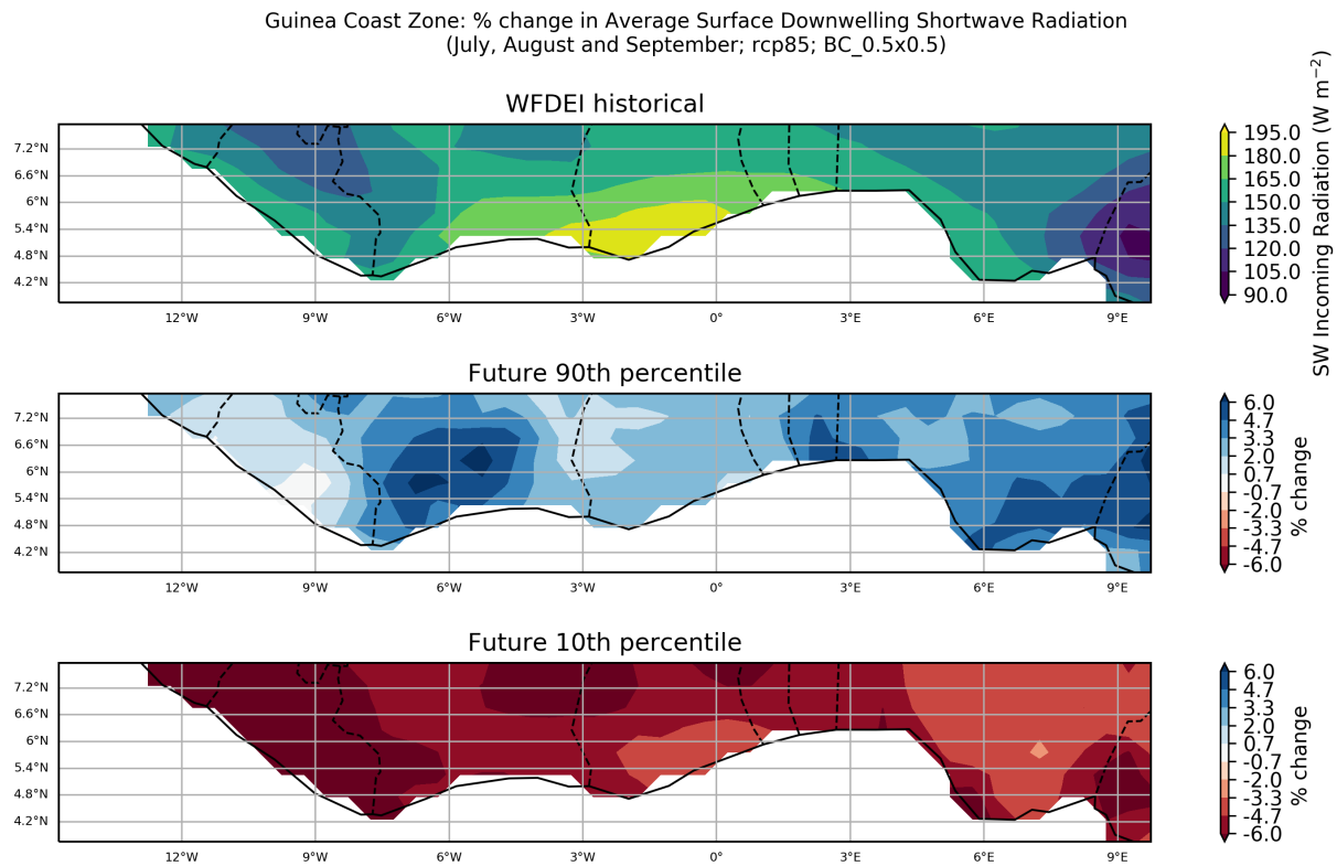
Figure 49: These maps show the ensemble spread in the percentage change in Average Surface Downwelling Shortwave Radiation for the period 2040 to 2059 (compared to a baseline period of 1950 - 2000) for the July, August and September season. They show the 90th and 10th percentiles of the distribution across the model ensemble, computed separately at each grid point, for the Guinea Coast Zone region. This particular plot shows the percentage change for the RCP8.5 scenario.
