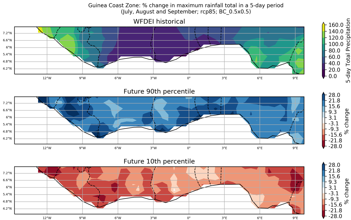
Figure 80: These maps show the ensemble spread in the percentage change in Maximum Rainfall Total in a 5-day Period for the period 2040 to 2059 (compared to a baseline period of 1950 - 2000) for the July, August and September season. They show the 90th and 10th percentiles of the distribution across the model ensemble, computed separately at each grid point, for the Guinea Coast Zone region. This particular plot shows the percentage change for the RCP8.5 scenario.
