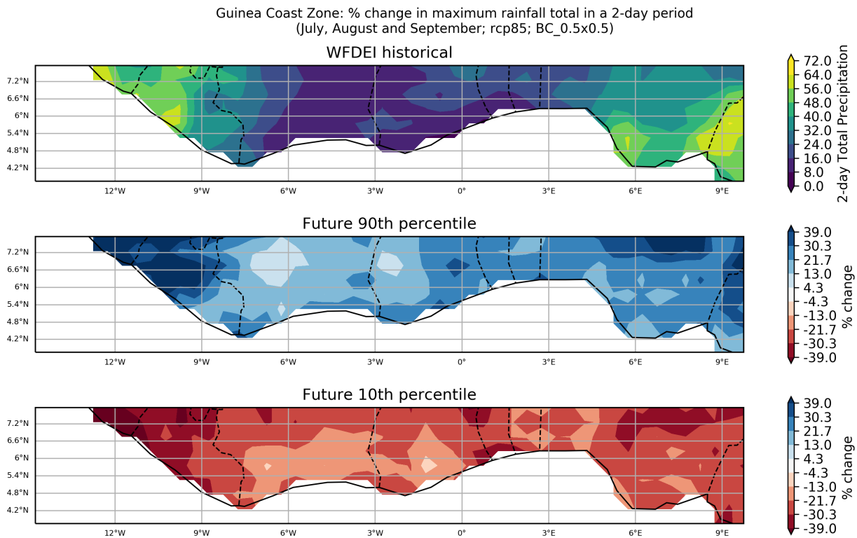
Figure 88: These maps show the ensemble spread in the percentage change in Maximum Rainfall Total in a 2-day Period for the period 2040 to 2059 (compared to a baseline period of 1950 - 2000) for the July, August and September season. They show the 90th and 10th percentiles of the distribution across the model ensemble, computed separately at each grid point, for the Guinea Coast Zone region. This particular plot shows the percentage change for the RCP8.5 scenario.
