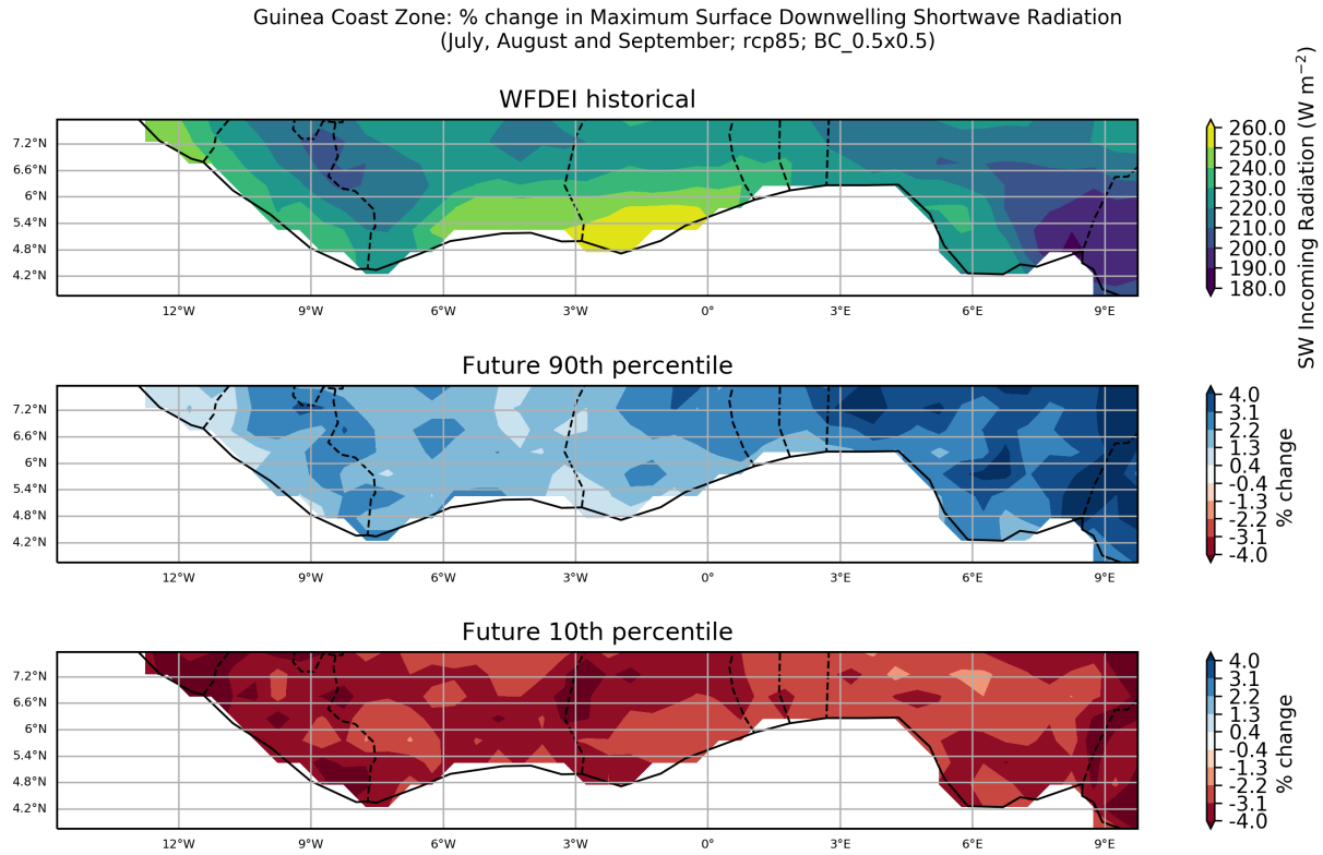
Figure 33: These maps show the ensemble spread in the percentage change in Maximum Surface Downwelling Shortwave Radiation for the period 2040 to 2059 (compared to a baseline period of 1950 - 2000) for the July, August and September season. They show the 90th and 10th percentiles of the distribution across the model ensemble, computed separately at each grid point, for the Guinea Coast Zone region. This particular plot shows the percentage change for the RCP8.5 scenario.
