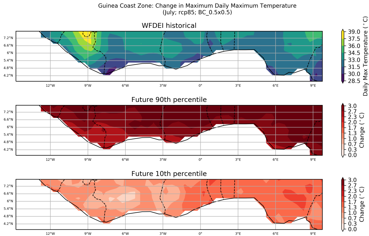
Figure 29: These maps show the ensemble spread in the absolute change in Maximum Daily Maximum Temperature for the period 2040 to 2059 (compared to a baseline period of 1950 - 2000) for the July season. They show the 90th and 10th percentiles of the distribution across the model ensemble, computed separately at each grid point, for the Guinea Coast Zone region. This particular plot shows the absolute change for the RCP8.5 scenario.
