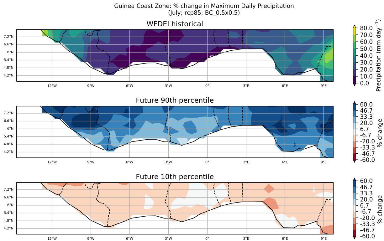
Figure 25: These maps show the ensemble spread in the percentage change in Maximum Daily Precipitation for the period 2040 to 2059 (compared to a baseline period of 1950 - 2000) for the July season. They show the 90th and 10th percentiles of the distribution across the model ensemble, computed separately at each grid point, for the Guinea Coast Zone region. This particular plot shows the percentage change for the RCP8.5 scenario.
