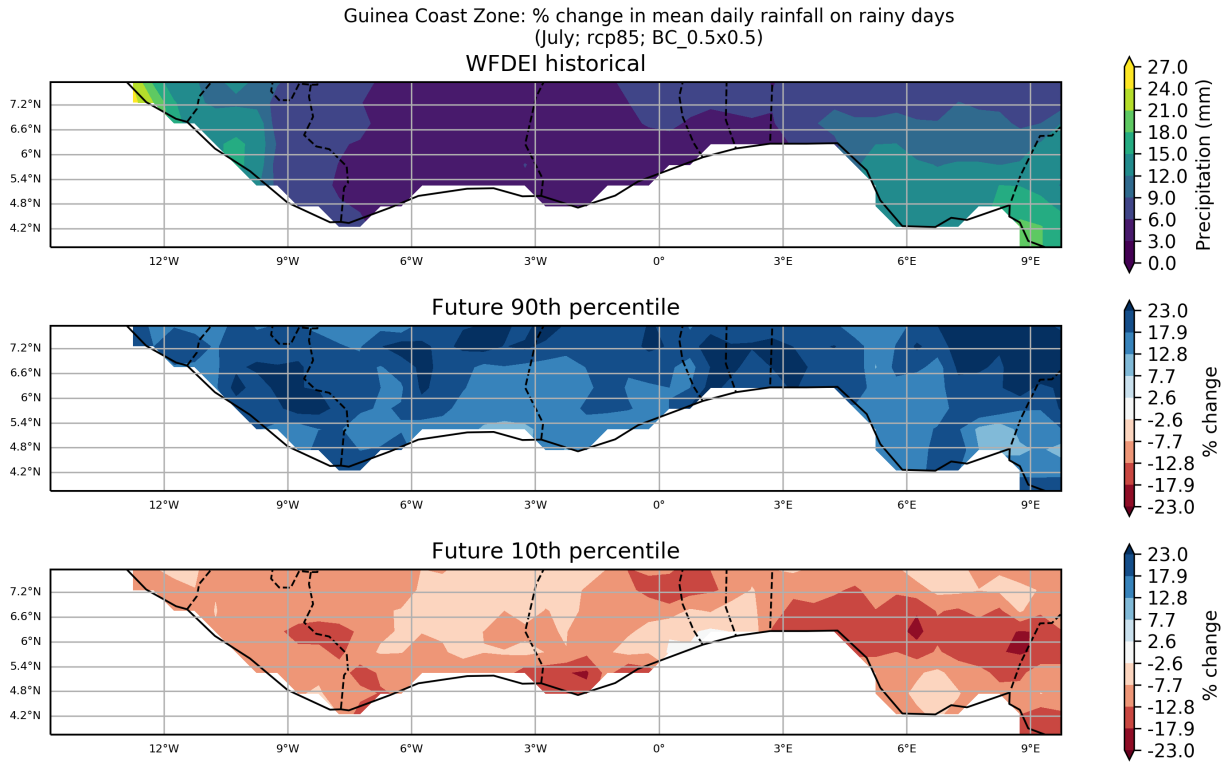
Figure 53: These maps show the ensemble spread in the percentage change in Mean Daily Rainfall on Rainy Days for the period 2040 to 2059 (compared to a baseline period of 1950 - 2000) for the July season. They show the 90th and 10th percentiles of the distribution across the model ensemble, computed separately at each grid point, for the Guinea Coast Zone region. This particular plot shows the percentage change for the RCP8.5 scenario.
