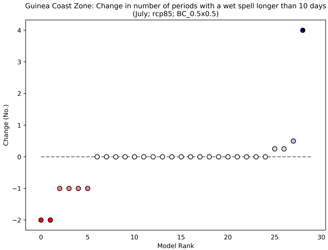
Figure 20: This scatterplot shows the absolute change in Number of Periods with a Wet Spell Longer Than 10 Days for the period 2040 to 2059 (compared to a baseline period of 1950 - 2000) for the July season. Each data point shows an individual model averaged over Guinea Coast Zone, and ranked according to the magnitude of the value on the y-axis. This particular plot shows the absolute change for the RCP8.5 scenario.
