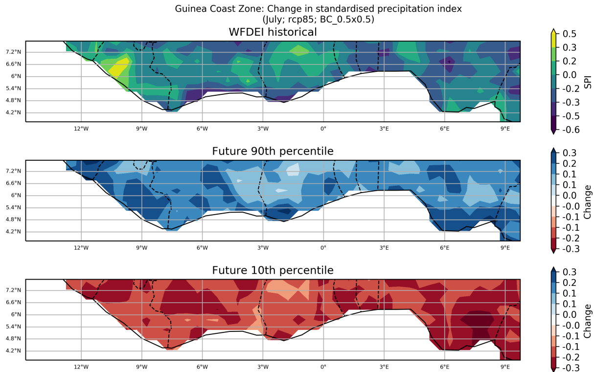
Figure 9: These maps show the ensemble spread in the absolute change in Standardised Precipitation Index for the period 2040 to 2059 (compared to a baseline period of 1950 - 2000) for the July season. They show the 90th and 10th percentiles of the distribution across the model ensemble, computed separately at each grid point, for the Guinea Coast Zone region. This particular plot shows the absolute change for the RCP8.5 scenario.
