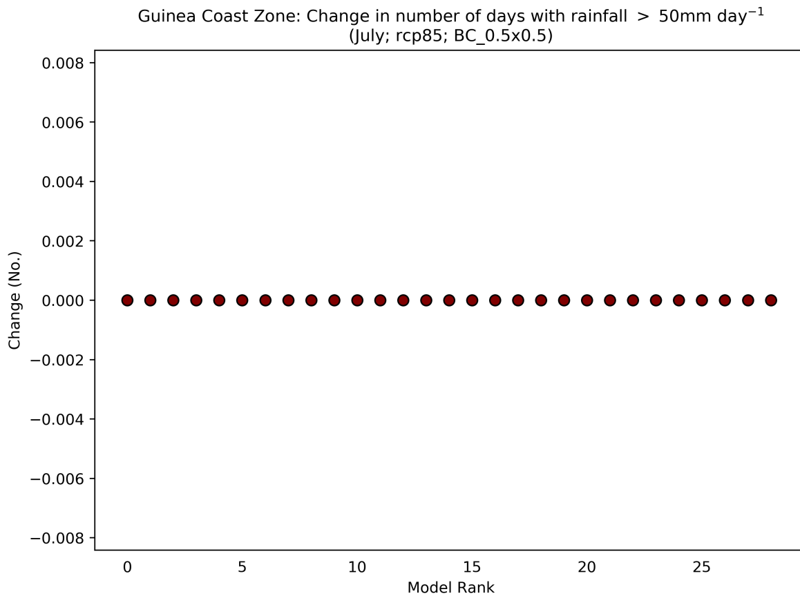
Figure 79: This scatterplot shows the absolute change in Number of Days with Rainfall > 50mm day -1 for the period 2040 to 2059 (compared to a baseline period of 1950 - 2000) for the July season. Each data point shows an individual model averaged over Guinea Coast Zone, and ranked according to the magnitude of the value on the y-axis. This particular plot shows the absolute change for the RCP8.5 scenario.
