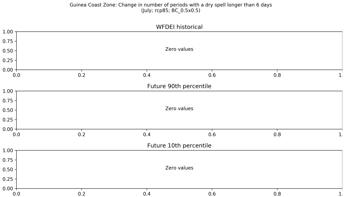
Figure 21: These maps show the ensemble spread in the absolute change in Number of Periods with a Dry Spell Longer Than 6 Days for the period 2040 to 2059 (compared to a baseline period of 1950 - 2000) for the July season. They show the 90th and 10th percentiles of the distribution across the model ensemble, computed separately at each grid point, for the Guinea Coast Zone region. This particular plot shows the absolute change for the RCP8.5 scenario.
