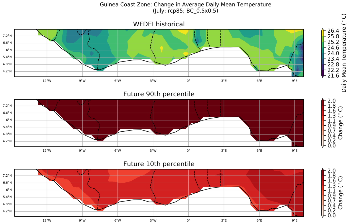
Figure 45: These maps show the ensemble spread in the absolute change in Average Daily Mean Temperature for the period 2040 to 2059 (compared to a baseline period of 1950 - 2000) for the July season. They show the 90th and 10th percentiles of the distribution across the model ensemble, computed separately at each grid point, for the Guinea Coast Zone region. This particular plot shows the absolute change for the RCP8.5 scenario.
