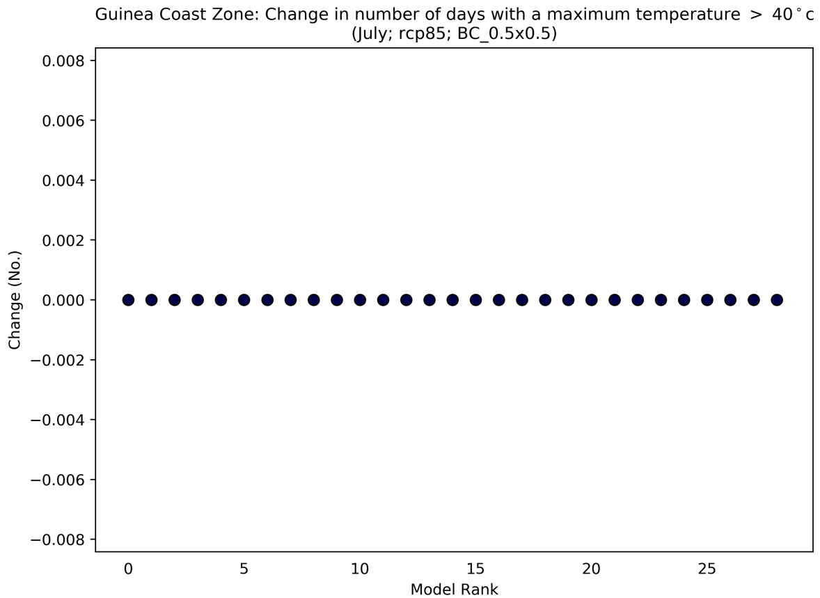
Figure 71: This scatterplot shows the absolute change in Number of Days with a Maximum Temperature > 40°C for the period 2040 to 2059 (compared to a baseline period of 1950 - 2000) for the July season. Each data point shows an individual model averaged over Guinea Coast Zone, and ranked according to the magnitude of the value on the y-axis. This particular plot shows the absolute change for the RCP8.5 scenario.
