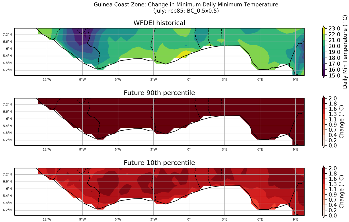
Figure 37: These maps show the ensemble spread in the absolute change in Minimum Daily Minimum Temperature for the period 2040 to 2059 (compared to a baseline period of 1950 - 2000) for the July season. They show the 90th and 10th percentiles of the distribution across the model ensemble, computed separately at each grid point, for the Guinea Coast Zone region. This particular plot shows the absolute change for the RCP8.5 scenario.
