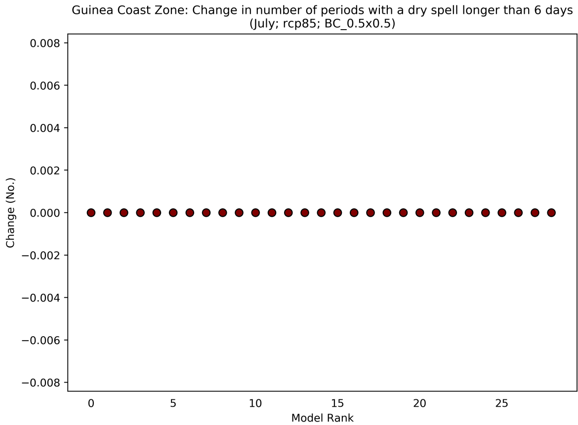
Figure 24: This scatterplot shows the absolute change in Number of Periods with a Dry Spell Longer Than 6 Days for the period 2040 to 2059 (compared to a baseline period of 1950 - 2000) for the July season. Each data point shows an individual model averaged over Guinea Coast Zone, and ranked according to the magnitude of the value on the y-axis. This particular plot shows the absolute change for the RCP8.5 scenario.
