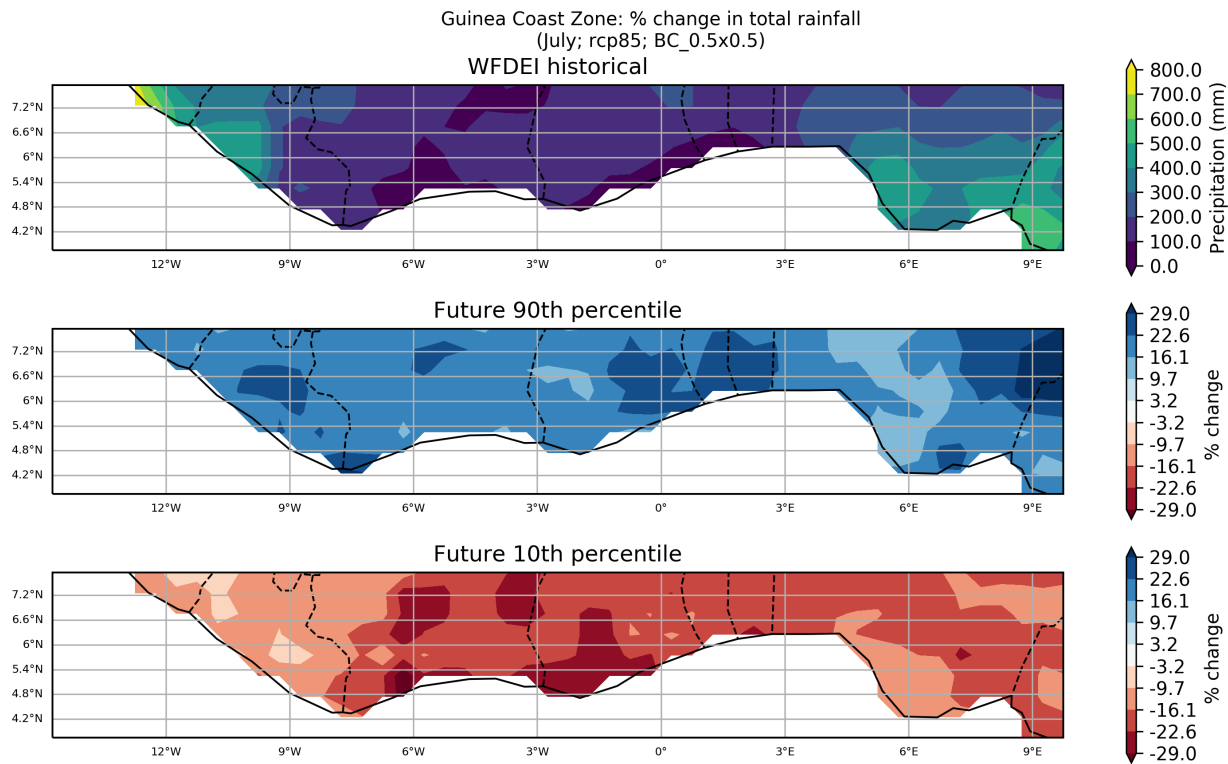
Figure 41: These maps show the ensemble spread in the percentage change in Total Rainfall for the period 2040 to 2059 (compared to a baseline period of 1950 - 2000) for the July season. They show the 90th and 10th percentiles of the distribution across the model ensemble, computed separately at each grid point, for the Guinea Coast Zone region. This particular plot shows the percentage change for the RCP8.5 scenario.
