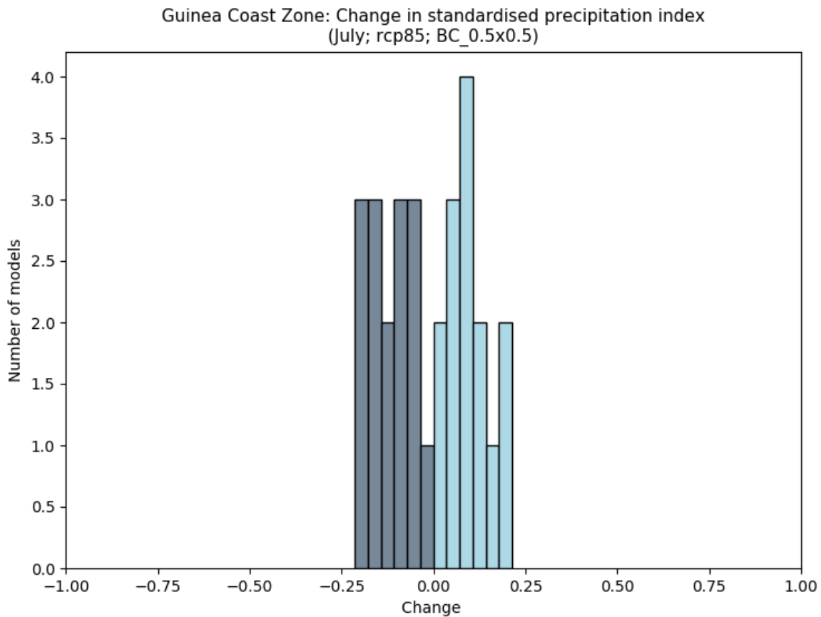
Figure 10: This histogram shows the number of models that agree on the absolute change in Standardised Precipitation Index for the period 2040 to 2059 (compared to a baseline period of 1950 - 2000) for the July season. Each vertical bar shows the number of models that agree on the range of values shown on the x-axis for the Guinea Coast Zone region. This particular plot shows the absolute change for the RCP8.5 scenario.
