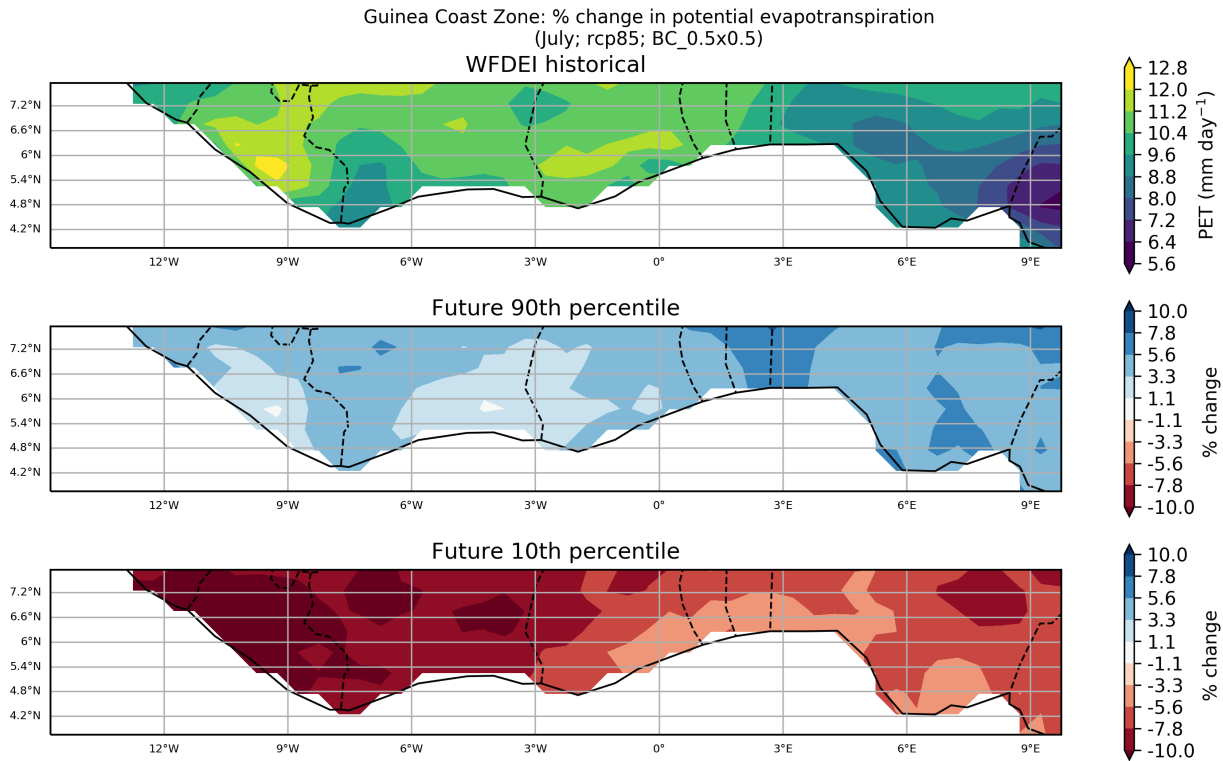
Figure 1: These maps show the ensemble spread in the percentage change in Potential Evapotranspiration for the period 2040 to 2059 (compared to a baseline period of 1950 - 2000) for the July season. They show the 90th and 10th percentiles of the distribution across the model ensemble, computed separately at each grid point, for the Guinea Coast Zone region. This particular plot shows the percentage change for the RCP8.5 scenario.
