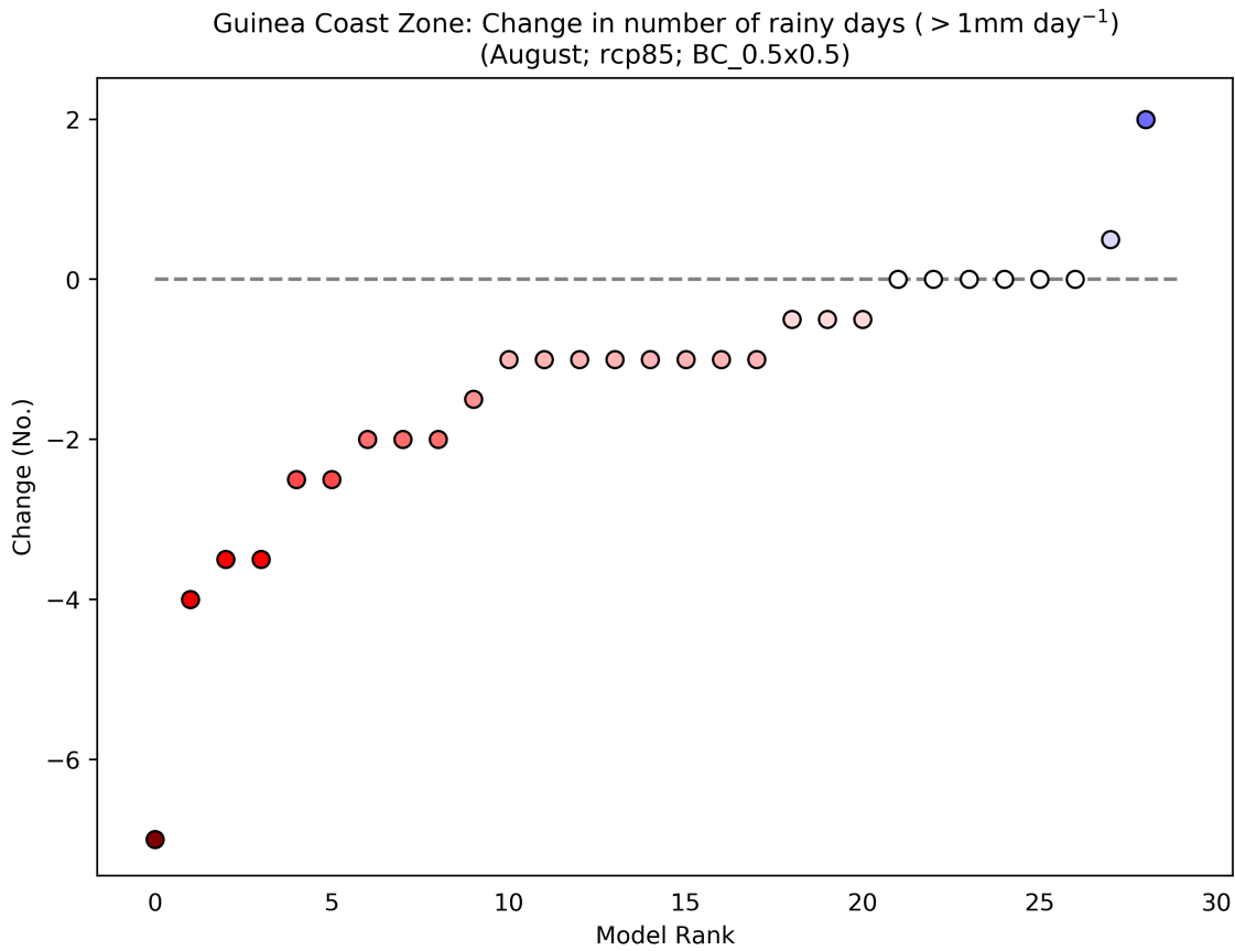
Figure 67: This scatterplot shows the absolute change in Number of Rainy Days ( >1\text{mm day}^{-1} ) for the period 2040 to 2059 (compared to a baseline period of 1950 - 2000) for the August season. Each data point shows an individual model averaged over Guinea Coast Zone, and ranked according to the magnitude of the value on the y-axis. This particular plot shows the absolute change for the RCP8.5 scenario.
