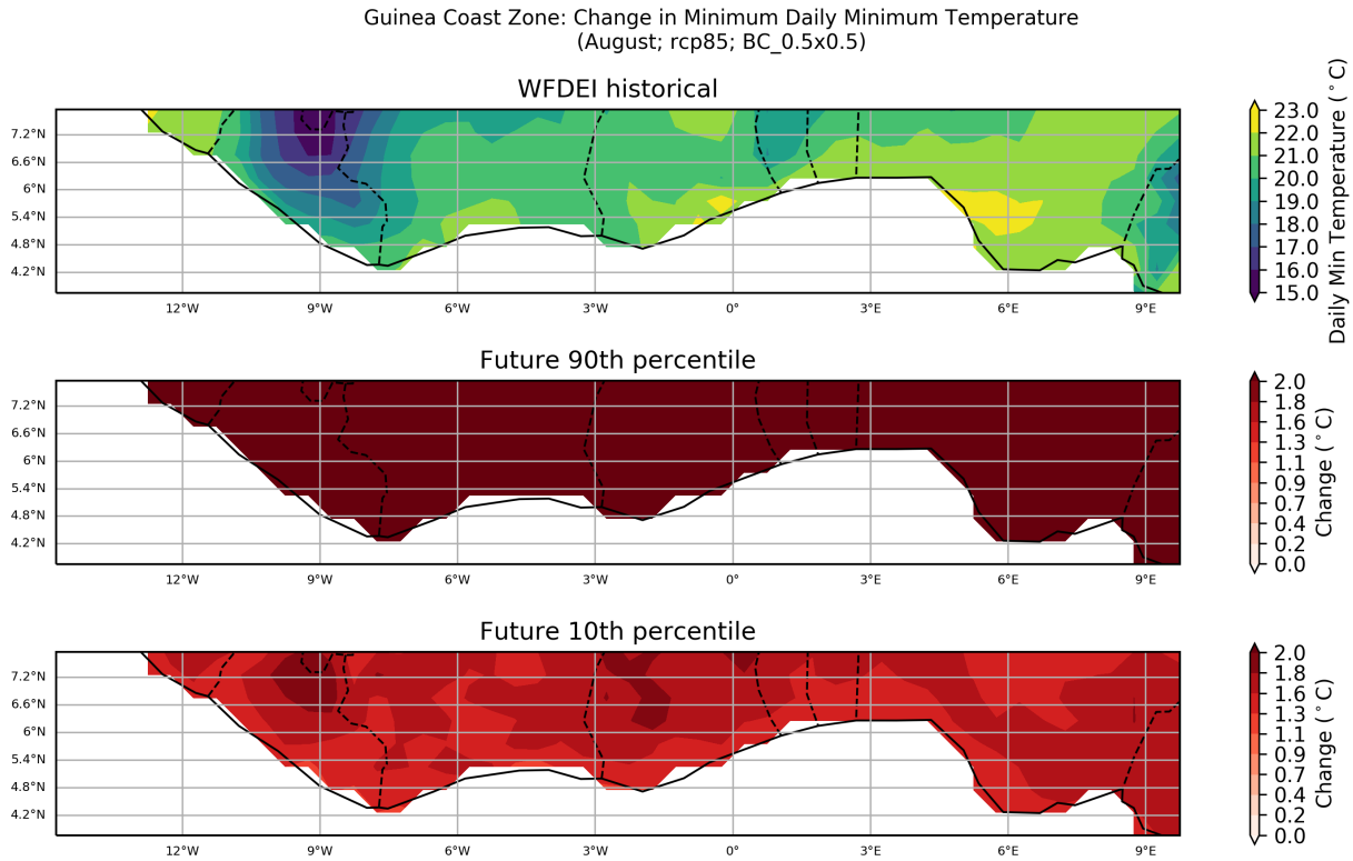
Figure 37: These maps show the ensemble spread in the absolute change in Minimum Daily Minimum Temperature for the period 2040 to 2059 (compared to a baseline period of 1950 - 2000) for the August season. They show the 90th and 10th percentiles of the distribution across the model ensemble, computed separately at each grid point, for the Guinea Coast Zone region. This particular plot shows the absolute change for the RCP8.5 scenario.
