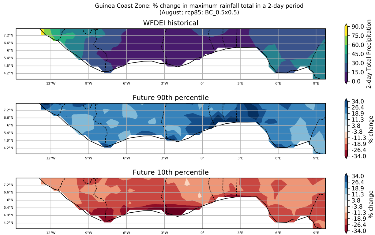
Figure 88: These maps show the ensemble spread in the percentage change in Maximum Rainfall Total in a 2-day Period for the period 2040 to 2059 (compared to a baseline period of 1950 - 2000) for the August season. They show the 90th and 10th percentiles of the distribution across the model ensemble, computed separately at each grid point, for the Guinea Coast Zone region. This particular plot shows the percentage change for the RCP8.5 scenario.
