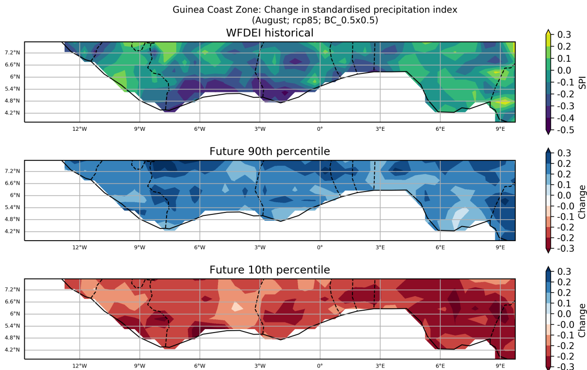
Figure 9: These maps show the ensemble spread in the absolute change in Standardised Precipitation Index for the period 2040 to 2059 (compared to a baseline period of 1950 - 2000) for the August season. They show the 90th and 10th percentiles of the distribution across the model ensemble, computed separately at each grid point, for the Guinea Coast Zone region. This particular plot shows the absolute change for the RCP8.5 scenario.
