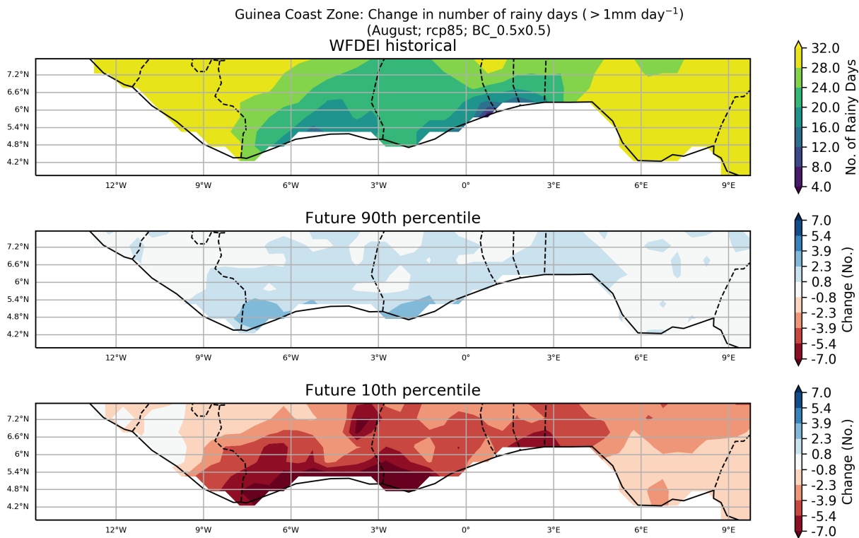
Figure 64: These maps show the ensemble spread in the absolute change in Number of Rainy Days ( >1\text{mm day}^{-1} ) for the period 2040 to 2059 (compared to a baseline period of 1950 - 2000) for the August season. They show the 90th and 10th percentiles of the distribution across the model ensemble, computed separately at each grid point, for the Guinea Coast Zone region. This particular plot shows the absolute change for the RCP8.5 scenario.
