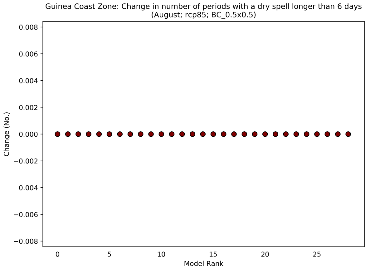
Figure 24: This scatterplot shows the absolute change in Number of Periods with a Dry Spell Longer Than 6 Days for the period 2040 to 2059 (compared to a baseline period of 1950 - 2000) for the August season. Each data point shows an individual model averaged over Guinea Coast Zone, and ranked according to the magnitude of the value on the y-axis. This particular plot shows the absolute change for the RCP8.5 scenario.
