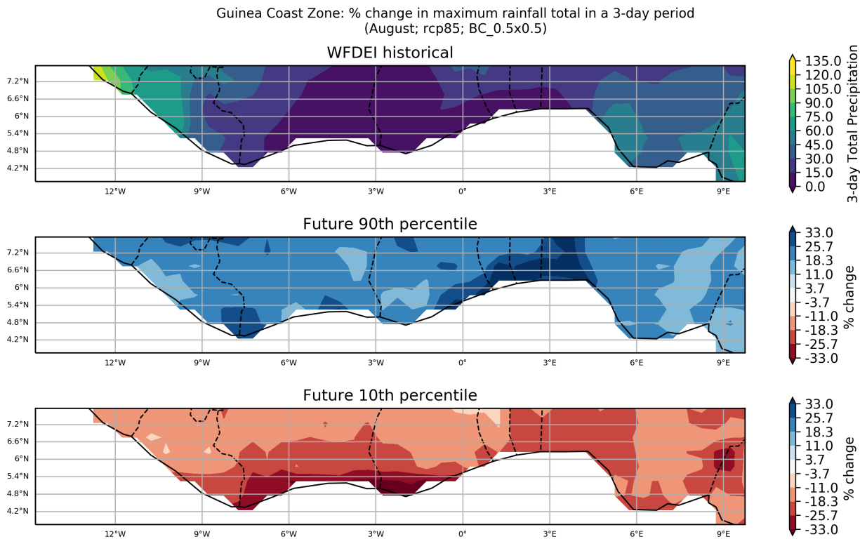
Figure 84: These maps show the ensemble spread in the percentage change in Maximum Rainfall Total in a 3-day Period for the period 2040 to 2059 (compared to a baseline period of 1950 - 2000) for the August season. They show the 90th and 10th percentiles of the distribution across the model ensemble, computed separately at each grid point, for the Guinea Coast Zone region. This particular plot shows the percentage change for the RCP8.5 scenario.
