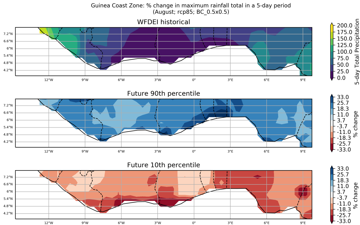
Figure 80: These maps show the ensemble spread in the percentage change in Maximum Rainfall Total in a 5-day Period for the period 2040 to 2059 (compared to a baseline period of 1950 - 2000) for the August season. They show the 90th and 10th percentiles of the distribution across the model ensemble, computed separately at each grid point, for the Guinea Coast Zone region. This particular plot shows the percentage change for the RCP8.5 scenario.
