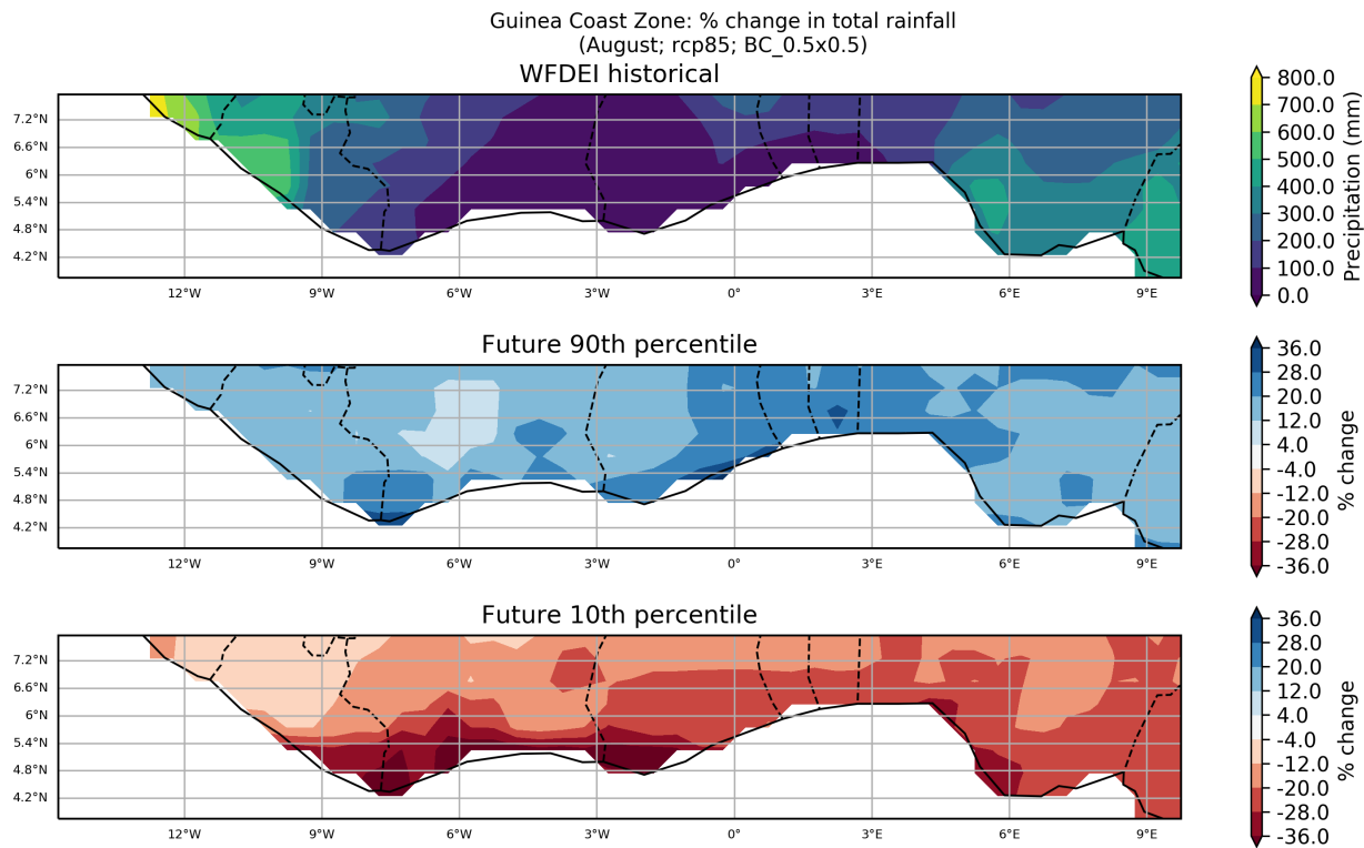
Figure 41: These maps show the ensemble spread in the percentage change in Total Rainfall for the period 2040 to 2059 (compared to a baseline period of 1950 - 2000) for the August season. They show the 90th and 10th percentiles of the distribution across the model ensemble, computed separately at each grid point, for the Guinea Coast Zone region. This particular plot shows the percentage change for the RCP8.5 scenario.
