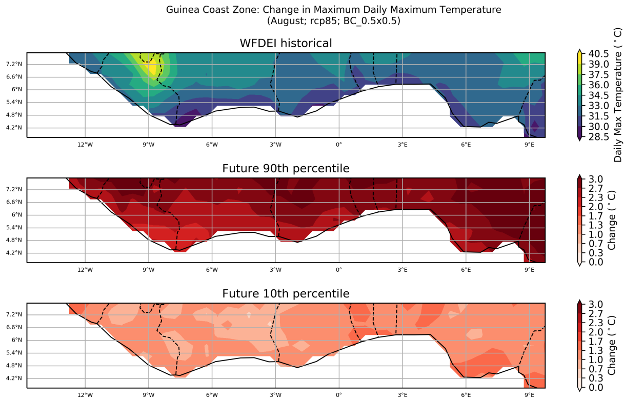
Figure 29: These maps show the ensemble spread in the absolute change in Maximum Daily Maximum Temperature for the period 2040 to 2059 (compared to a baseline period of 1950 - 2000) for the August season. They show the 90th and 10th percentiles of the distribution across the model ensemble, computed separately at each grid point, for the Guinea Coast Zone region. This particular plot shows the absolute change for the RCP8.5 scenario.
