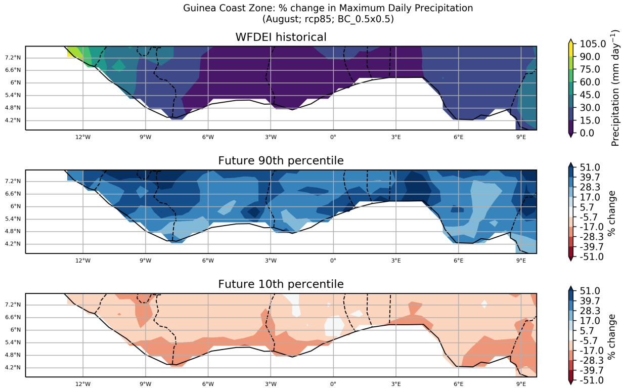
Figure 25: These maps show the ensemble spread in the percentage change in Maximum Daily Precipitation for the period 2040 to 2059 (compared to a baseline period of 1950 - 2000) for the August season. They show the 90th and 10th percentiles of the distribution across the model ensemble, computed separately at each grid point, for the Guinea Coast Zone region. This particular plot shows the percentage change for the RCP8.5 scenario.
