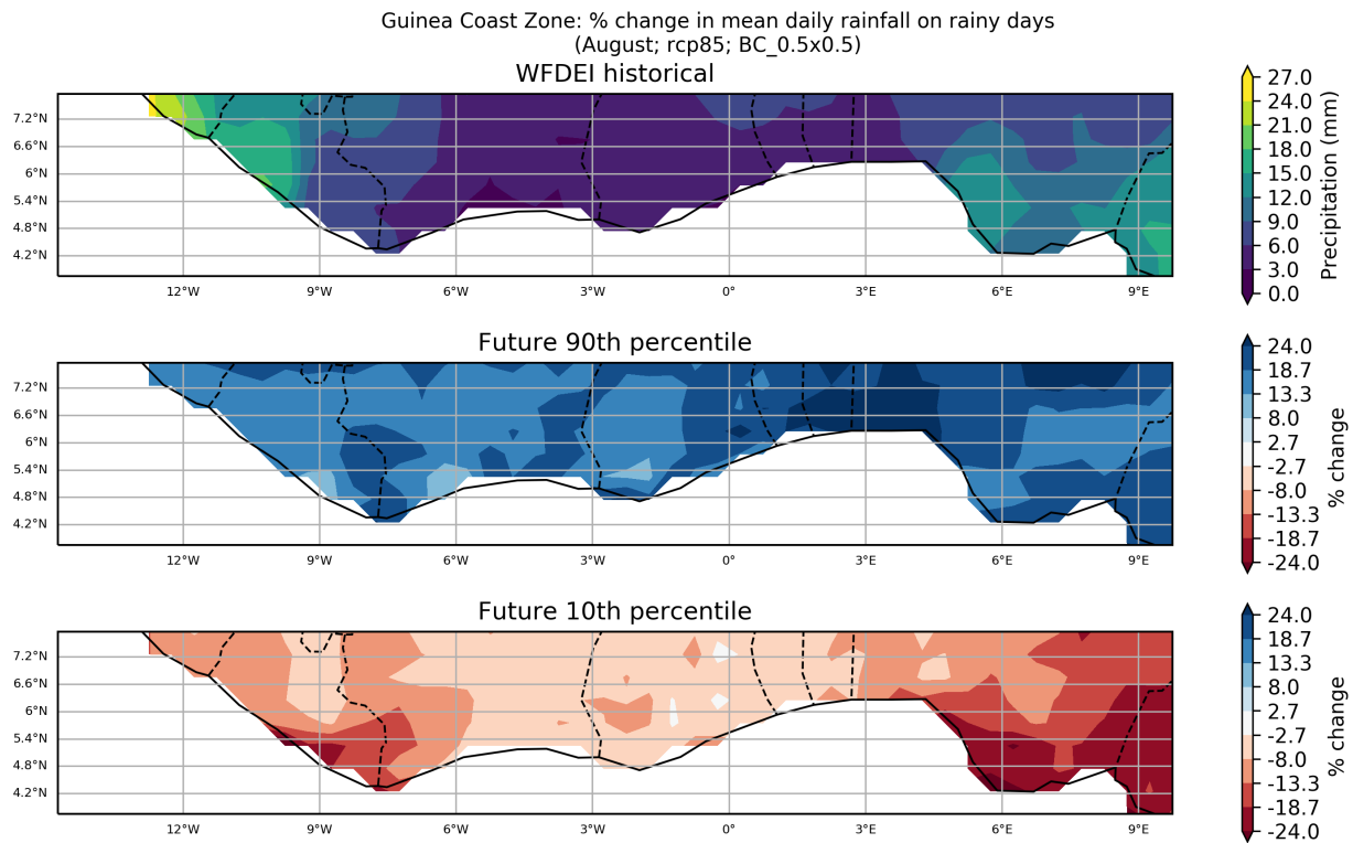
Figure 53: These maps show the ensemble spread in the percentage change in Mean Daily Rainfall on Rainy Days for the period 2040 to 2059 (compared to a baseline period of 1950 - 2000) for the August season. They show the 90th and 10th percentiles of the distribution across the model ensemble, computed separately at each grid point, for the Guinea Coast Zone region. This particular plot shows the percentage change for the RCP8.5 scenario.
