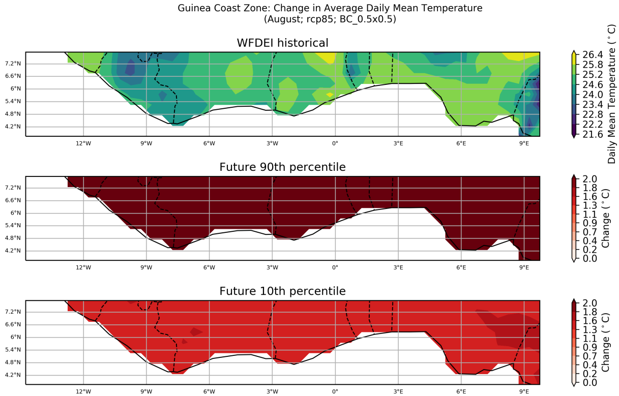
Figure 45: These maps show the ensemble spread in the absolute change in Average Daily Mean Temperature for the period 2040 to 2059 (compared to a baseline period of 1950 - 2000) for the August season. They show the 90th and 10th percentiles of the distribution across the model ensemble, computed separately at each grid point, for the Guinea Coast Zone region. This particular plot shows the absolute change for the RCP8.5 scenario.
