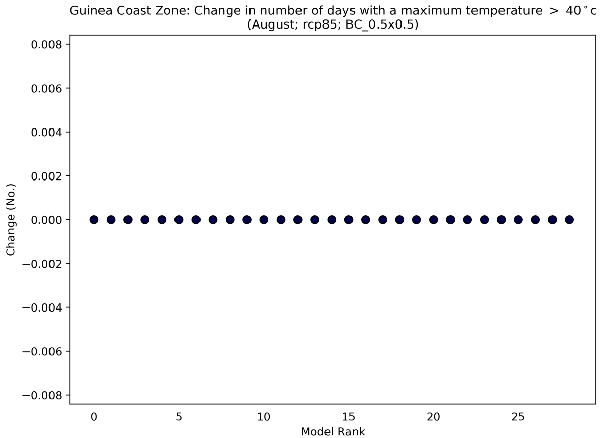
Figure 71: This scatterplot shows the absolute change in Number of Days with a Maximum Temperature > 40°C for the period 2040 to 2059 (compared to a baseline period of 1950 - 2000) for the August season. Each data point shows an individual model averaged over Guinea Coast Zone, and ranked according to the magnitude of the value on the y-axis. This particular plot shows the absolute change for the RCP8.5 scenario.
