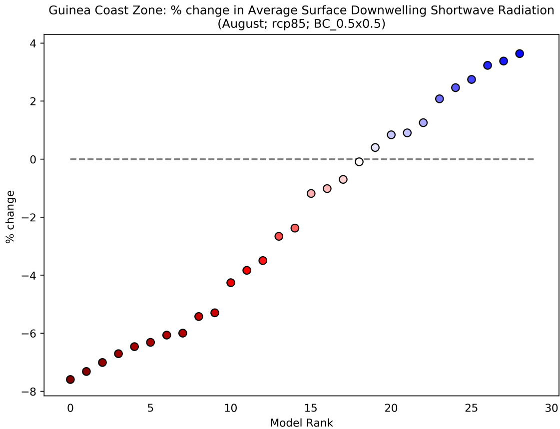
Figure 52: This scatterplot shows the percentage change in Average Surface Downwelling Shortwave Radiation for the period 2040 to 2059 (compared to a baseline period of 1950 - 2000) for the August season. Each data point shows an individual model averaged over Guinea Coast Zone, and ranked according to the magnitude of the value on the y-axis. This particular plot shows the percentage change for the RCP8.5 scenario.
