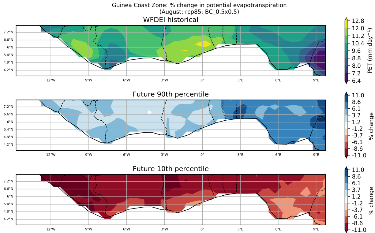
Figure 1: These maps show the ensemble spread in the percentage change in Potential Evapotranspiration for the period 2040 to 2059 (compared to a baseline period of 1950 - 2000) for the August season. They show the 90th and 10th percentiles of the distribution across the model ensemble, computed separately at each grid point, for the Guinea Coast Zone region. This particular plot shows the percentage change for the RCP8.5 scenario.
