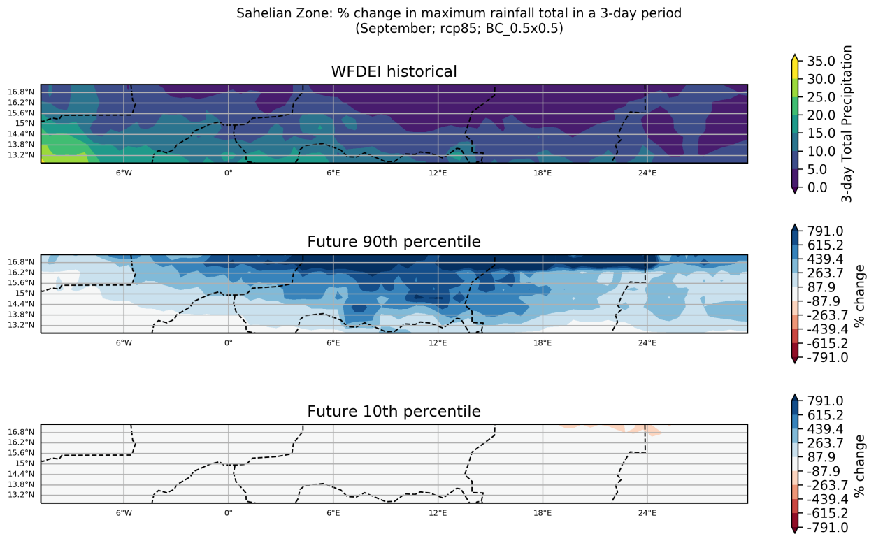
Figure 84: These maps show the ensemble spread in the percentage change in Maximum Rainfall Total in a 3-day Period for the period 2040 to 2059 (compared to a baseline period of 1950 - 2000) for the September season. They show the 90th and 10th percentiles of the distribution across the model ensemble, computed separately at each grid point, for the Sahelian Zone region. This particular plot shows the percentage change for the RCP8.5 scenario.
