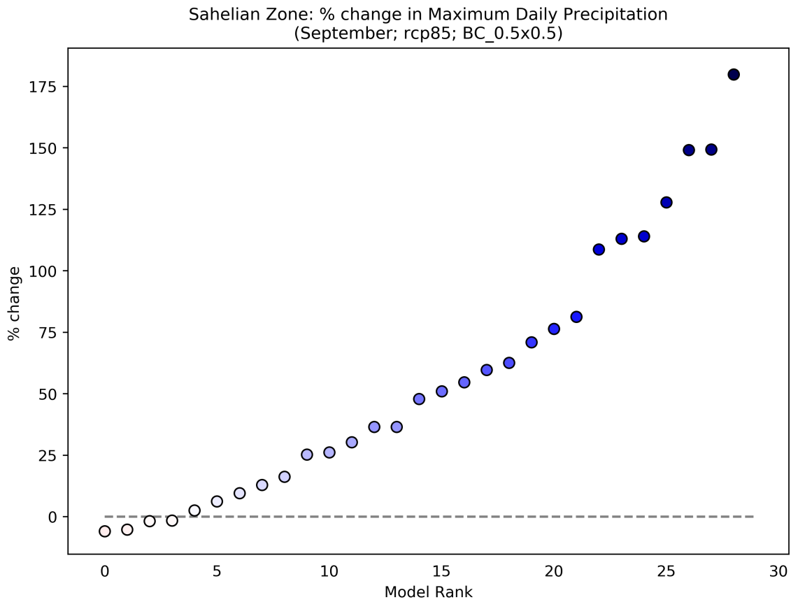
Figure 28: This scatterplot shows the percentage change in Maximum Daily Precipitation for the period 2040 to 2059 (compared to a baseline period of 1950 - 2000) for the September season. Each data point shows an individual model averaged over Sahelian Zone, and ranked according to the magnitude of the value on the y-axis. This particular plot shows the percentage change for the RCP8.5 scenario.
