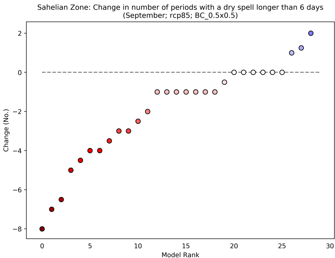
Figure 24: This scatterplot shows the absolute change in Number of Periods with a Dry Spell Longer Than 6 Days for the period 2040 to 2059 (compared to a baseline period of 1950 - 2000) for the September season. Each data point shows an individual model averaged over Sahelian Zone, and ranked according to the magnitude of the value on the y-axis. This particular plot shows the absolute change for the RCP8.5 scenario.
