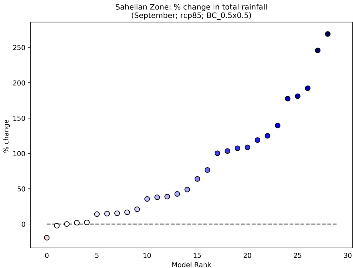
Figure 44: This scatterplot shows the percentage change in Total Rainfall for the period 2040 to 2059 (compared to a baseline period of 1950 - 2000) for the September season. Each data point shows an individual model averaged over Sahelian Zone, and ranked according to the magnitude of the value on the y-axis. This particular plot shows the percentage change for the RCP8.5 scenario.
