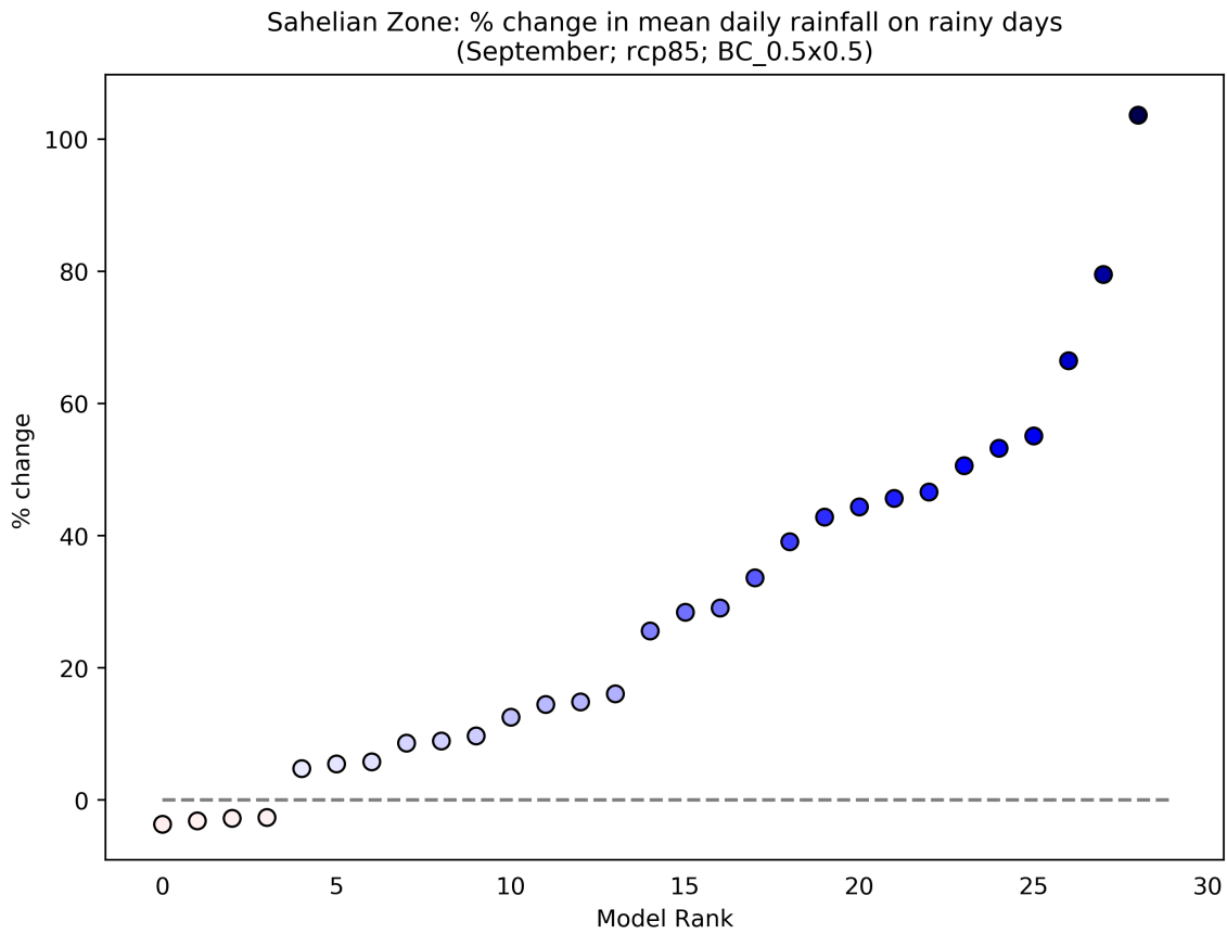
Figure 56: This scatterplot shows the percentage change in Mean Daily Rainfall on Rainy Days for the period 2040 to 2059 (compared to a baseline period of 1950 - 2000) for the September season. Each data point shows an individual model averaged over Sahelian Zone, and ranked according to the magnitude of the value on the y-axis. This particular plot shows the percentage change for the RCP8.5 scenario.
