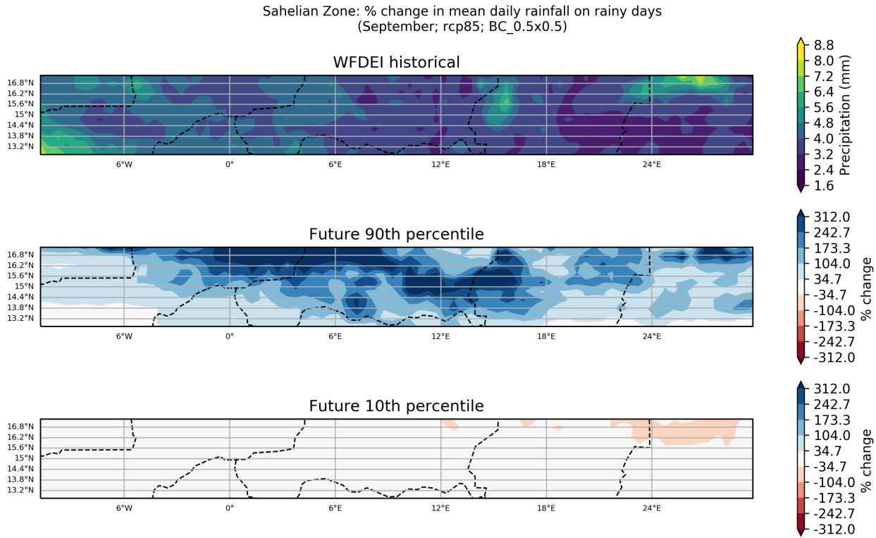
Figure 53: These maps show the ensemble spread in the percentage change in Mean Daily Rainfall on Rainy Days for the period 2040 to 2059 (compared to a baseline period of 1950 - 2000) for the September season. They show the 90th and 10th percentiles of the distribution across the model ensemble, computed separately at each grid point, for the Sahelian Zone region. This particular plot shows the percentage change for the RCP8.5 scenario.
