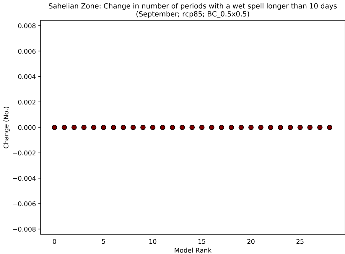
Figure 20: This scatterplot shows the absolute change in Number of Periods with a Wet Spell Longer Than 10 Days for the period 2040 to 2059 (compared to a baseline period of 1950 - 2000) for the September season. Each data point shows an individual model averaged over Sahelian Zone, and ranked according to the magnitude of the value on the y-axis. This particular plot shows the absolute change for the RCP8.5 scenario.
