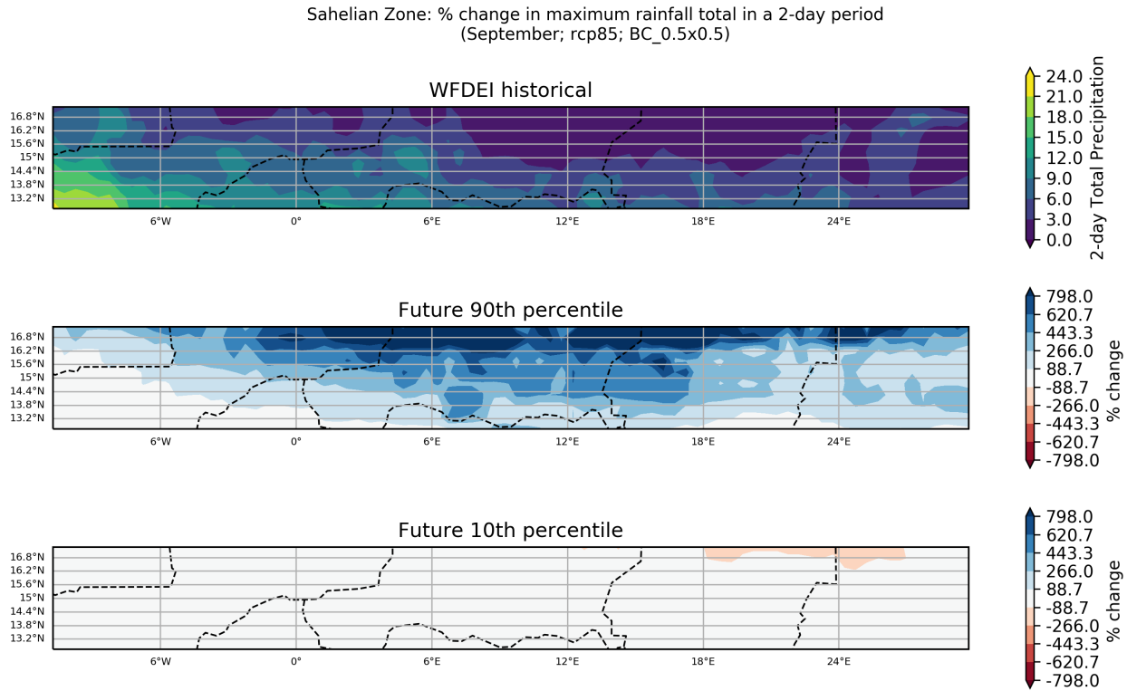
Figure 88: These maps show the ensemble spread in the percentage change in Maximum Rainfall Total in a 2-day Period for the period 2040 to 2059 (compared to a baseline period of 1950 - 2000) for the September season. They show the 90th and 10th percentiles of the distribution across the model ensemble, computed separately at each grid point, for the Sahelian Zone region. This particular plot shows the percentage change for the RCP8.5 scenario.
