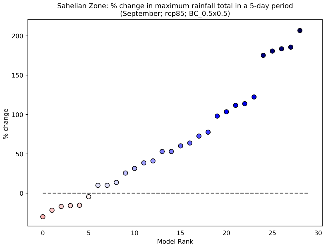
Figure 83: This scatterplot shows the percentage change in Maximum Rainfall Total in a 5-day Period for the period 2040 to 2059 (compared to a baseline period of 1950 - 2000) for the September season. Each data point shows an individual model averaged over Sahelian Zone, and ranked according to the magnitude of the value on the y-axis. This particular plot shows the percentage change for the RCP8.5 scenario.
