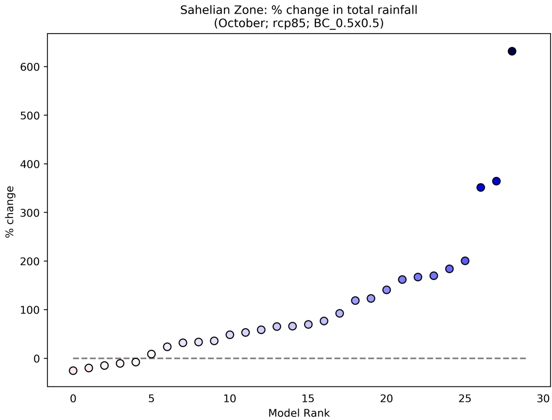
Figure 44: This scatterplot shows the percentage change in Total Rainfall for the period 2040 to 2059 (compared to a baseline period of 1950 - 2000) for the October season. Each data point shows an individual model averaged over Sahelian Zone, and ranked according to the magnitude of the value on the y-axis. This particular plot shows the percentage change for the RCP8.5 scenario.
