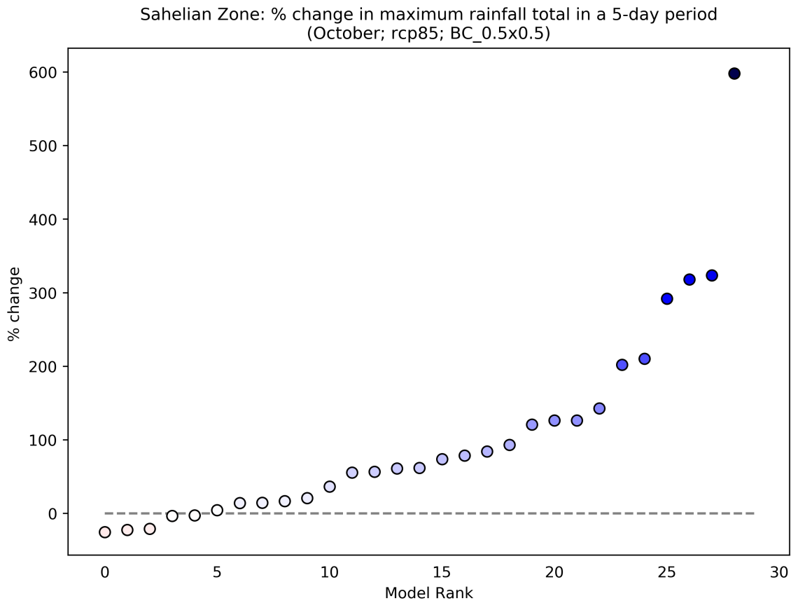
Figure 83: This scatterplot shows the percentage change in Maximum Rainfall Total in a 5-day Period for the period 2040 to 2059 (compared to a baseline period of 1950 - 2000) for the October season. Each data point shows an individual model averaged over Sahelian Zone, and ranked according to the magnitude of the value on the y-axis. This particular plot shows the percentage change for the RCP8.5 scenario.
