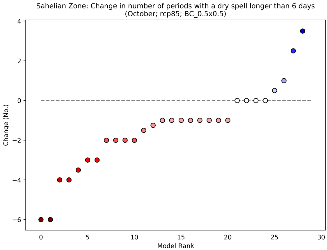
Figure 24: This scatterplot shows the absolute change in Number of Periods with a Dry Spell Longer Than 6 Days for the period 2040 to 2059 (compared to a baseline period of 1950 - 2000) for the October season. Each data point shows an individual model averaged over Sahelian Zone, and ranked according to the magnitude of the value on the y-axis. This particular plot shows the absolute change for the RCP8.5 scenario.
