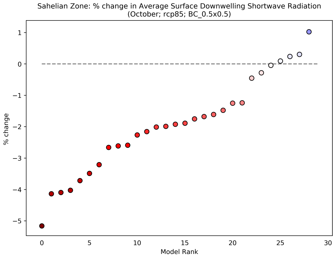
Figure 52: This scatterplot shows the percentage change in Average Surface Downwelling Shortwave Radiation for the period 2040 to 2059 (compared to a baseline period of 1950 - 2000) for the October season. Each data point shows an individual model averaged over Sahelian Zone, and ranked according to the magnitude of the value on the y-axis. This particular plot shows the percentage change for the RCP8.5 scenario.
