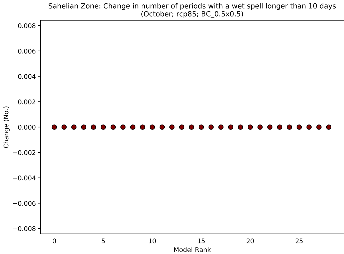
Figure 20: This scatterplot shows the absolute change in Number of Periods with a Wet Spell Longer Than 10 Days for the period 2040 to 2059 (compared to a baseline period of 1950 - 2000) for the October season. Each data point shows an individual model averaged over Sahelian Zone, and ranked according to the magnitude of the value on the y-axis. This particular plot shows the absolute change for the RCP8.5 scenario.
