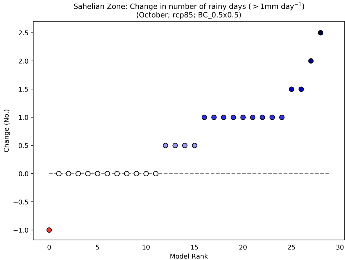
Figure 67: This scatterplot shows the absolute change in Number of Rainy Days ( >1\text{mm day}^{-1} ) for the period 2040 to 2059 (compared to a baseline period of 1950 - 2000) for the October season. Each data point shows an individual model averaged over Sahelian Zone, and ranked according to the magnitude of the value on the y-axis. This particular plot shows the absolute change for the RCP8.5 scenario.
