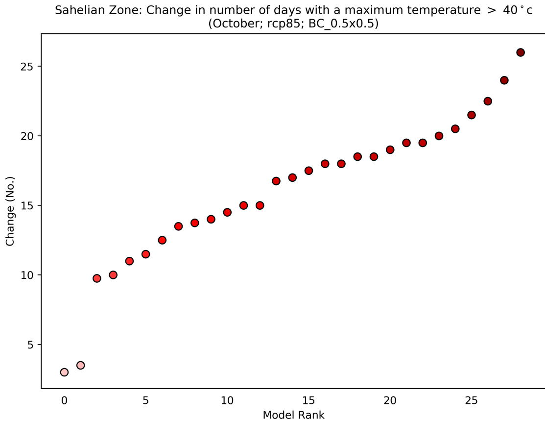
Figure 71: This scatterplot shows the absolute change in Number of Days with a Maximum Temperature > 40°C for the period 2040 to 2059 (compared to a baseline period of 1950 - 2000) for the October season. Each data point shows an individual model averaged over Sahelian Zone, and ranked according to the magnitude of the value on the y-axis. This particular plot shows the absolute change for the RCP8.5 scenario.
