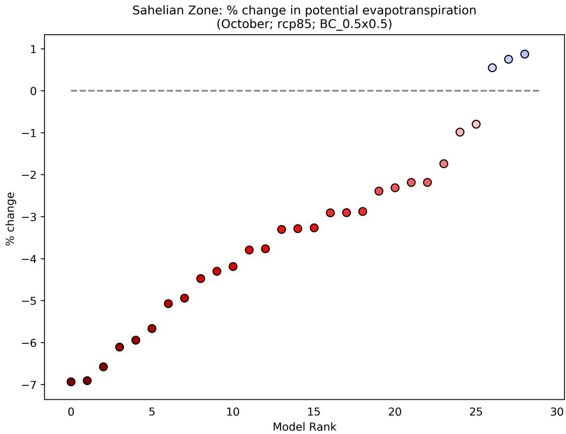
Figure 4: This scatterplot shows the percentage change in Potential Evapotranspiration for the period 2040 to 2059 (compared to a baseline period of 1950 - 2000) for the October season. Each data point shows an individual model averaged over Sahelian Zone, and ranked according to the magnitude of the value on the y-axis. This particular plot shows the percentage change for the RCP8.5 scenario.
