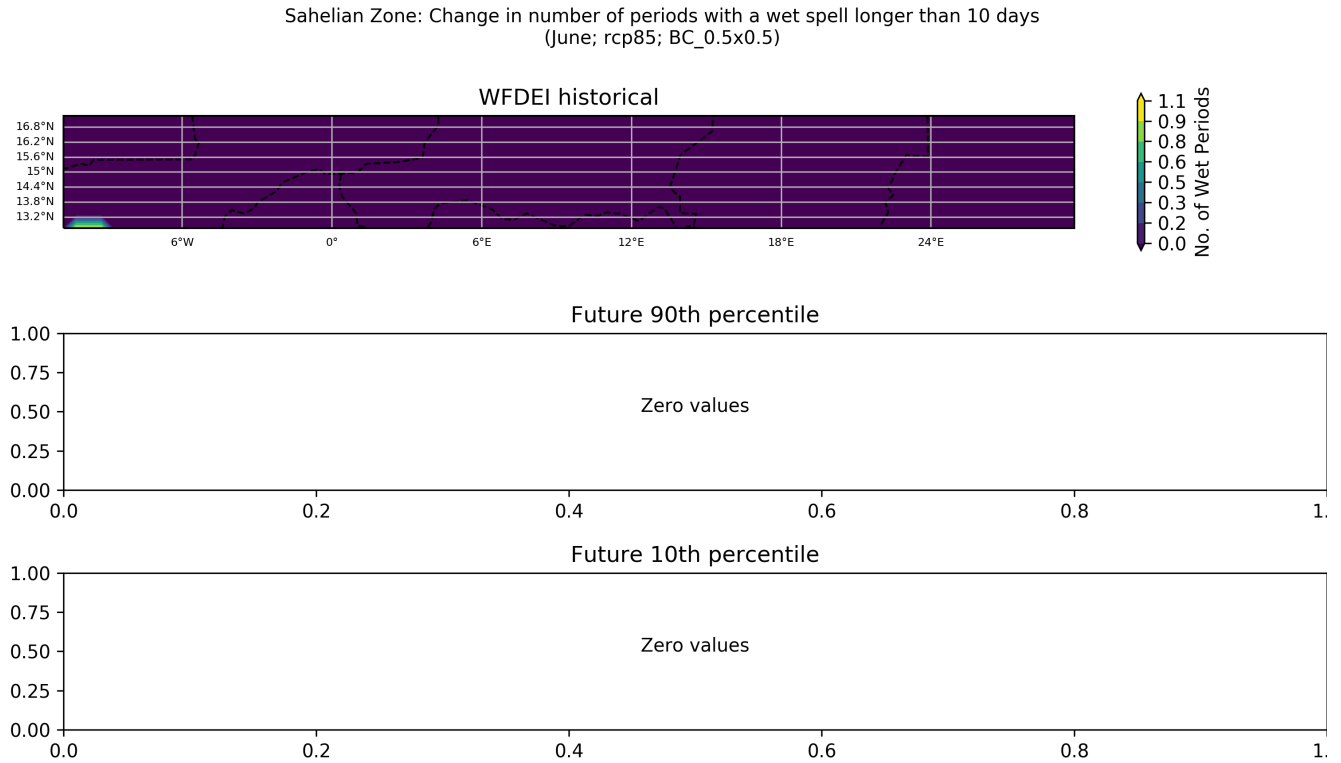
Figure 17: These maps show the ensemble spread in the absolute change in Number of Periods with a Wet Spell Longer Than 10 Days for the period 2040 to 2059 (compared to a baseline period of 1950 - 2000) for the June season. They show the 90th and 10th percentiles of the distribution across the model ensemble, computed separately at each grid point, for the Sahelian Zone region. This particular plot shows the absolute change for the RCP8.5 scenario.
