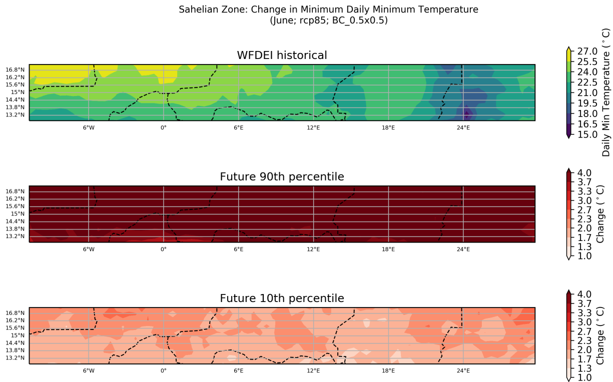
Figure 37: These maps show the ensemble spread in the absolute change in Minimum Daily Minimum Temperature for the period 2040 to 2059 (compared to a baseline period of 1950 - 2000) for the June season. They show the 90th and 10th percentiles of the distribution across the model ensemble, computed separately at each grid point, for the Sahelian Zone region. This particular plot shows the absolute change for the RCP8.5 scenario.
