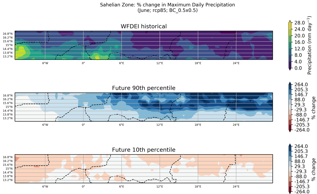
Figure 25: These maps show the ensemble spread in the percentage change in Maximum Daily Precipitation for the period 2040 to 2059 (compared to a baseline period of 1950 - 2000) for the June season. They show the 90th and 10th percentiles of the distribution across the model ensemble, computed separately at each grid point, for the Sahelian Zone region. This particular plot shows the percentage change for the RCP8.5 scenario.
