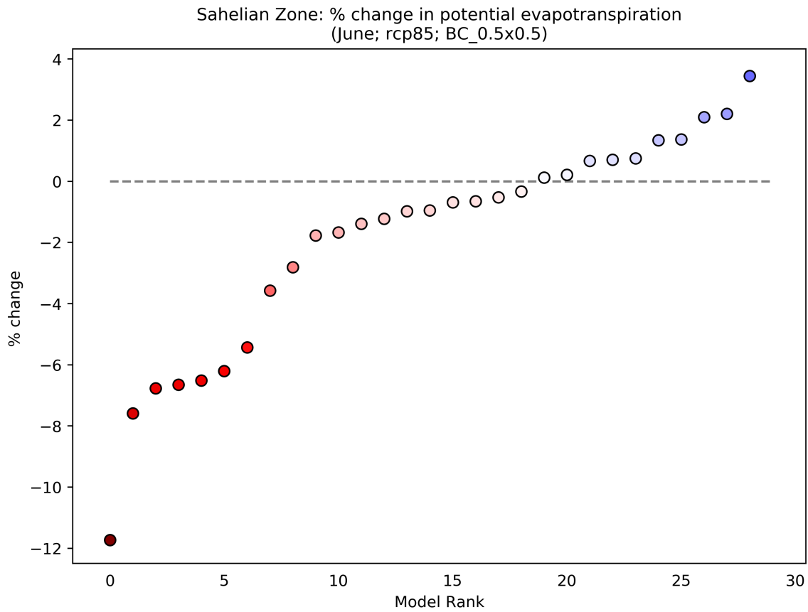
Figure 4: This scatterplot shows the percentage change in Potential Evapotranspiration for the period 2040 to 2059 (compared to a baseline period of 1950 - 2000) for the June season. Each data point shows an individual model averaged over Sahelian Zone, and ranked according to the magnitude of the value on the y-axis. This particular plot shows the percentage change for the RCP8.5 scenario.
