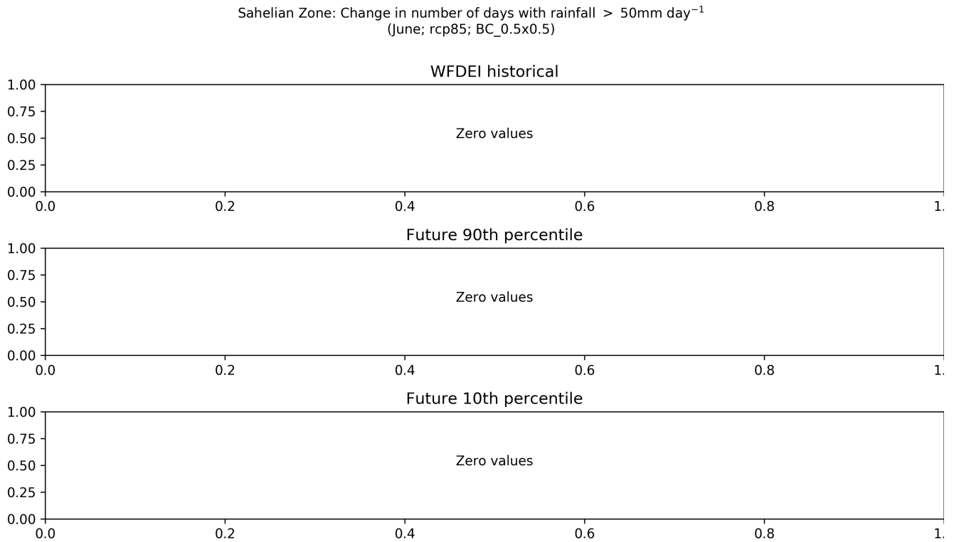
Figure 76: These maps show the ensemble spread in the absolute change in Number of Days with Rainfall > 50\text{mm day}^{-1} for the period 2040 to 2059 (compared to a baseline period of 1950 - 2000) for the June season. They show the 90th and 10th percentiles of the distribution across the model ensemble, computed separately at each grid point, for the Sahelian Zone region. This particular plot shows the absolute change for the RCP8.5 scenario.
