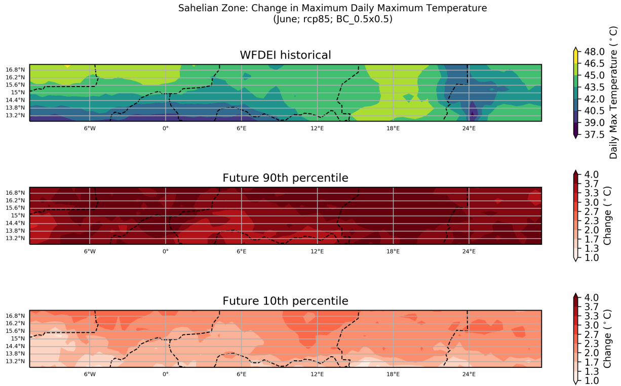
Figure 29: These maps show the ensemble spread in the absolute change in Maximum Daily Maximum Temperature for the period 2040 to 2059 (compared to a baseline period of 1950 - 2000) for the June season. They show the 90th and 10th percentiles of the distribution across the model ensemble, computed separately at each grid point, for the Sahelian Zone region. This particular plot shows the absolute change for the RCP8.5 scenario.
