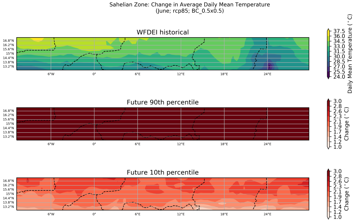
Figure 45: These maps show the ensemble spread in the absolute change in Average Daily Mean Temperature for the period 2040 to 2059 (compared to a baseline period of 1950 - 2000) for the June season. They show the 90th and 10th percentiles of the distribution across the model ensemble, computed separately at each grid point, for the Sahelian Zone region. This particular plot shows the absolute change for the RCP8.5 scenario.
