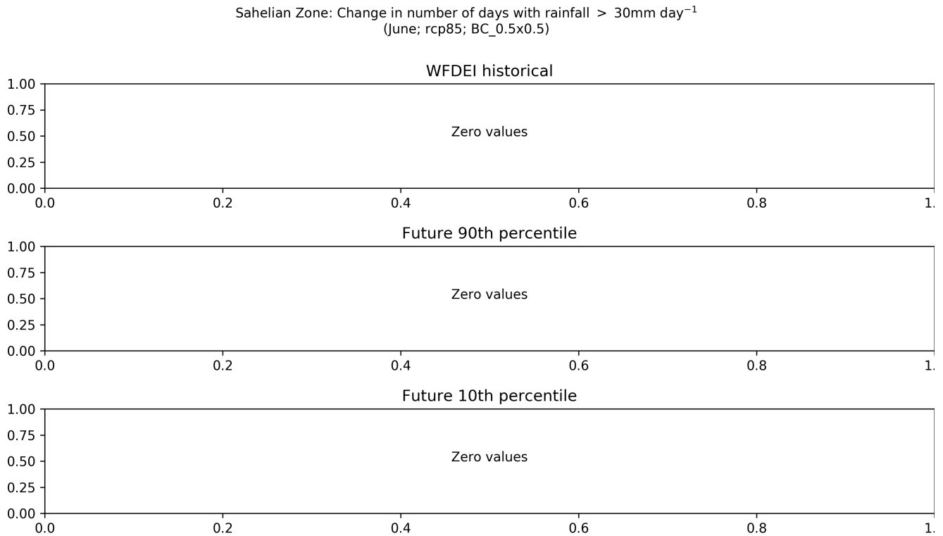
Figure 72: These maps show the ensemble spread in the absolute change in Number of Days with Rainfall > 30\text{mm day}^{-1} for the period 2040 to 2059 (compared to a baseline period of 1950 - 2000) for the June season. They show the 90th and 10th percentiles of the distribution across the model ensemble, computed separately at each grid point, for the Sahelian Zone region. This particular plot shows the absolute change for the RCP8.5 scenario.
