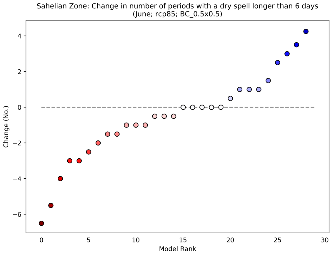
Figure 24: This scatterplot shows the absolute change in Number of Periods with a Dry Spell Longer Than 6 Days for the period 2040 to 2059 (compared to a baseline period of 1950 - 2000) for the June season. Each data point shows an individual model averaged over Sahelian Zone, and ranked according to the magnitude of the value on the y-axis. This particular plot shows the absolute change for the RCP8.5 scenario.
