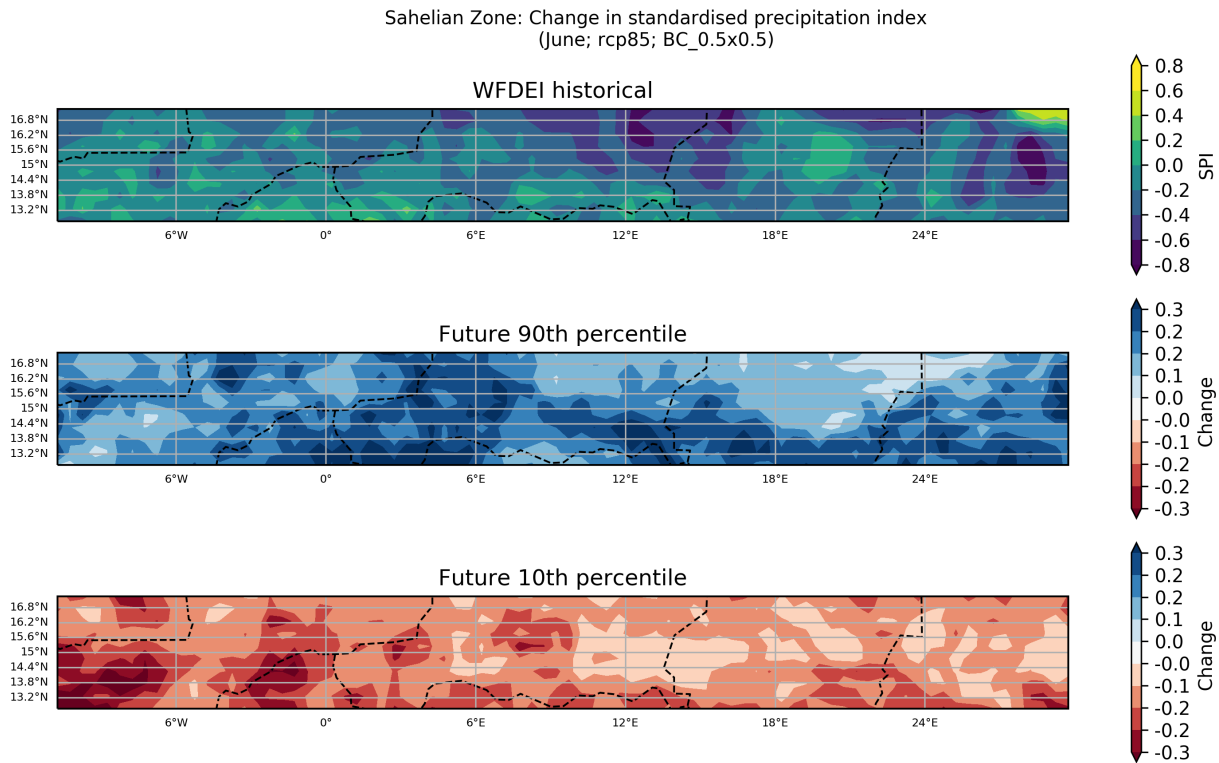
Figure 9: These maps show the ensemble spread in the absolute change in Standardised Precipitation Index for the period 2040 to 2059 (compared to a baseline period of 1950 - 2000) for the June season. They show the 90th and 10th percentiles of the distribution across the model ensemble, computed separately at each grid point, for the Sahelian Zone region. This particular plot shows the absolute change for the RCP8.5 scenario.
