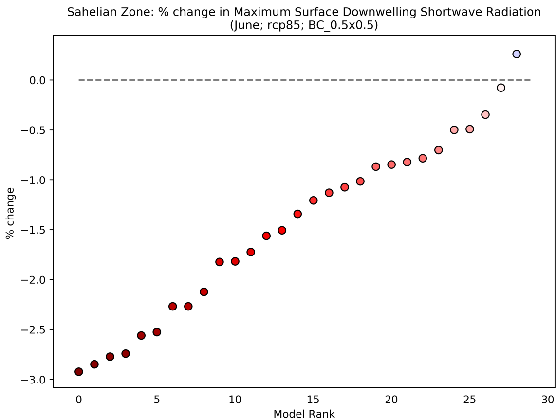
Figure 36: This scatterplot shows the percentage change in Maximum Surface Downwelling Shortwave Radiation for the period 2040 to 2059 (compared to a baseline period of 1950 - 2000) for the June season. Each data point shows an individual model averaged over Sahelian Zone, and ranked according to the magnitude of the value on the y-axis. This particular plot shows the percentage change for the RCP8.5 scenario.
