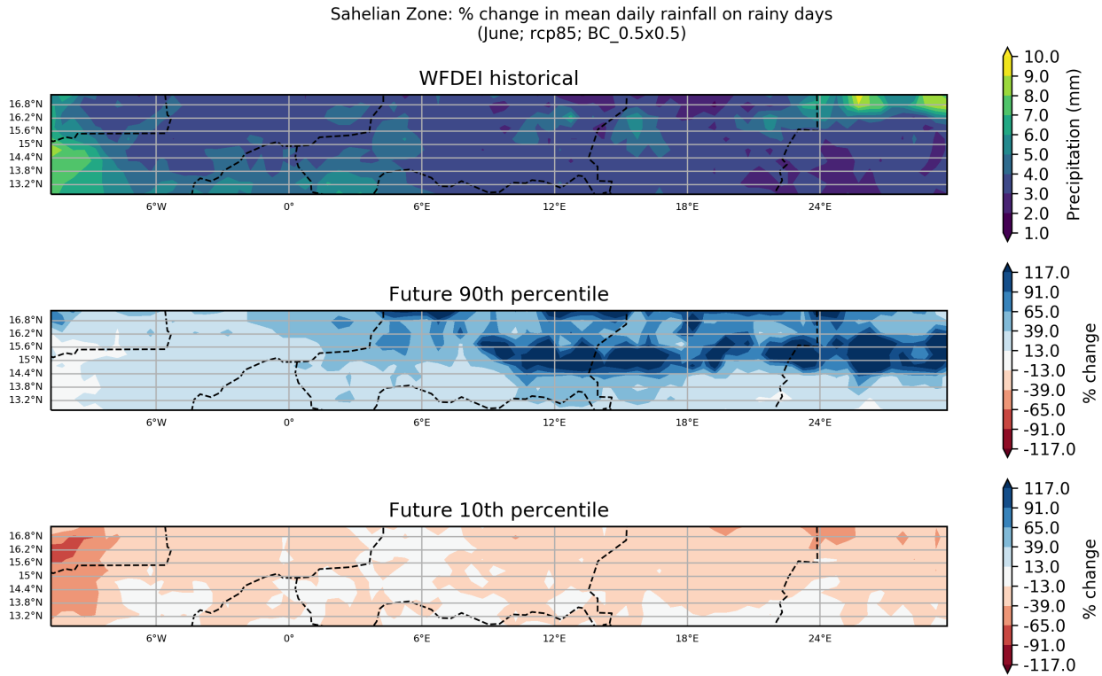
Figure 53: These maps show the ensemble spread in the percentage change in Mean Daily Rainfall on Rainy Days for the period 2040 to 2059 (compared to a baseline period of 1950 - 2000) for the June season. They show the 90th and 10th percentiles of the distribution across the model ensemble, computed separately at each grid point, for the Sahelian Zone region. This particular plot shows the percentage change for the RCP8.5 scenario.
