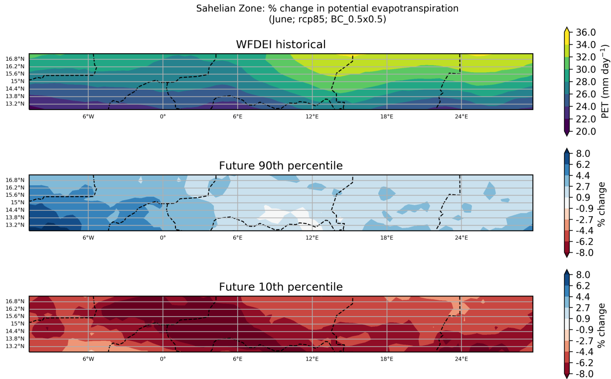
Figure 1: These maps show the ensemble spread in the percentage change in Potential Evapotranspiration for the period 2040 to 2059 (compared to a baseline period of 1950 - 2000) for the June season. They show the 90th and 10th percentiles of the distribution across the model ensemble, computed separately at each grid point, for the Sahelian Zone region. This particular plot shows the percentage change for the RCP8.5 scenario.
