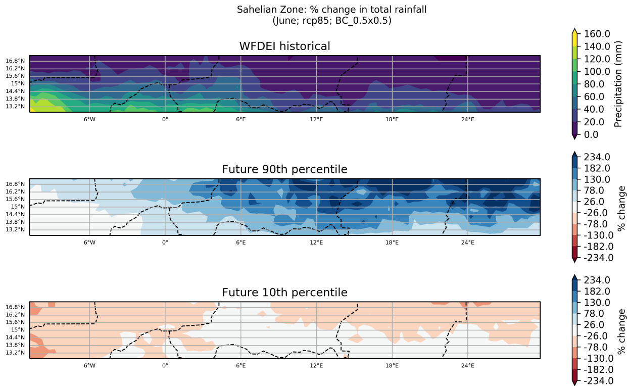
Figure 41: These maps show the ensemble spread in the percentage change in Total Rainfall for the period 2040 to 2059 (compared to a baseline period of 1950 - 2000) for the June season. They show the 90th and 10th percentiles of the distribution across the model ensemble, computed separately at each grid point, for the Sahelian Zone region. This particular plot shows the percentage change for the RCP8.5 scenario.
