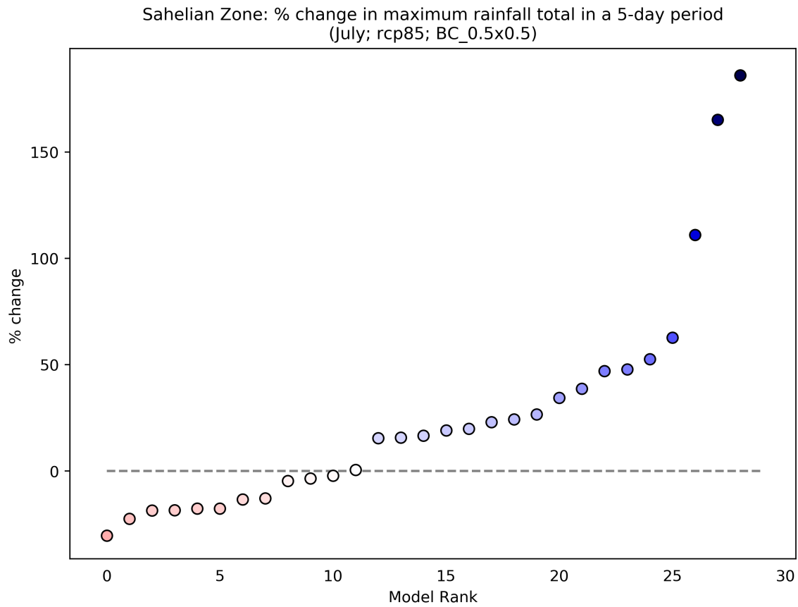
Figure 83: This scatterplot shows the percentage change in Maximum Rainfall Total in a 5-day Period for the period 2040 to 2059 (compared to a baseline period of 1950 - 2000) for the July season. Each data point shows an individual model averaged over Sahelian Zone, and ranked according to the magnitude of the value on the y-axis. This particular plot shows the percentage change for the RCP8.5 scenario.
