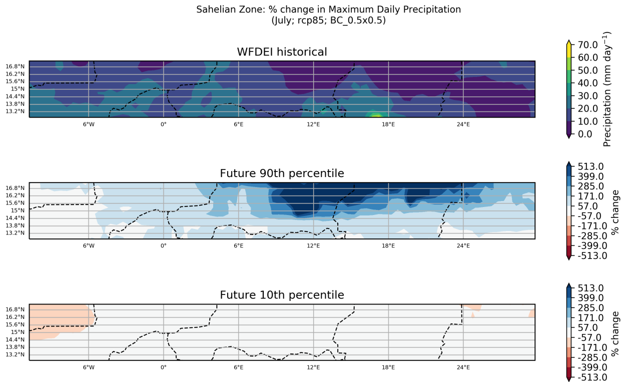
Figure 25: These maps show the ensemble spread in the percentage change in Maximum Daily Precipitation for the period 2040 to 2059 (compared to a baseline period of 1950 - 2000) for the July season. They show the 90th and 10th percentiles of the distribution across the model ensemble, computed separately at each grid point, for the Sahelian Zone region. This particular plot shows the percentage change for the RCP8.5 scenario.
