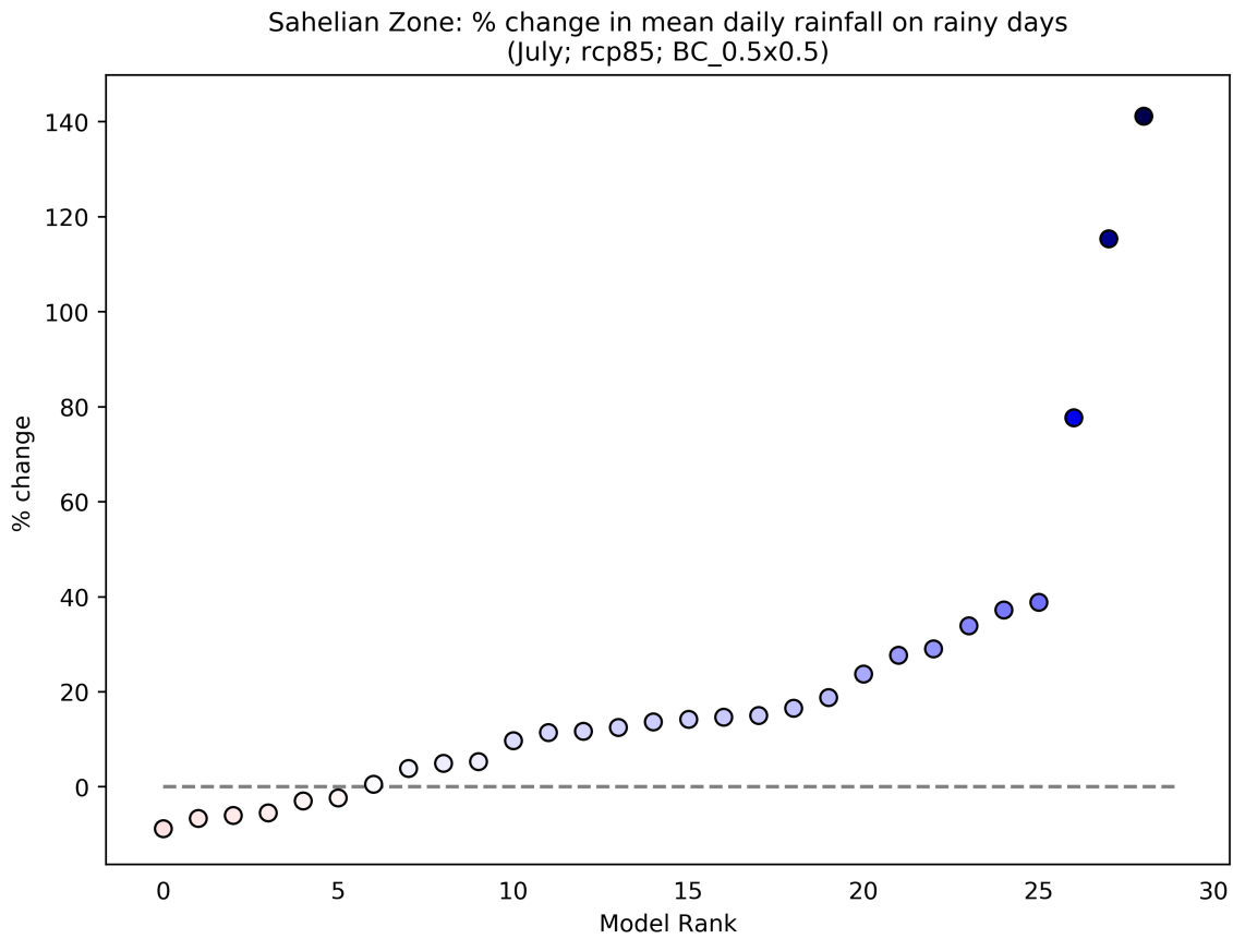
Figure 56: This scatterplot shows the percentage change in Mean Daily Rainfall on Rainy Days for the period 2040 to 2059 (compared to a baseline period of 1950 - 2000) for the July season. Each data point shows an individual model averaged over Sahelian Zone, and ranked according to the magnitude of the value on the y-axis. This particular plot shows the percentage change for the RCP8.5 scenario.
