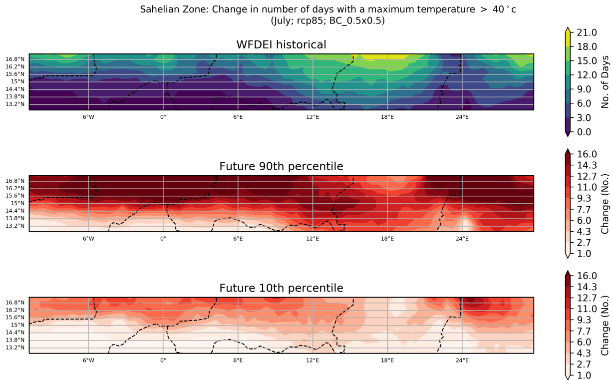
Figure 68: These maps show the ensemble spread in the absolute change in Number of Days with a Maximum Temperature > 40^{\circ}\text{C} for the period 2040 to 2059 (compared to a baseline period of 1950 - 2000) for the July season. They show the 90th and 10th percentiles of the distribution across the model ensemble, computed separately at each grid point, for the Sahelian Zone region. This particular plot shows the absolute change for the RCP8.5 scenario.
