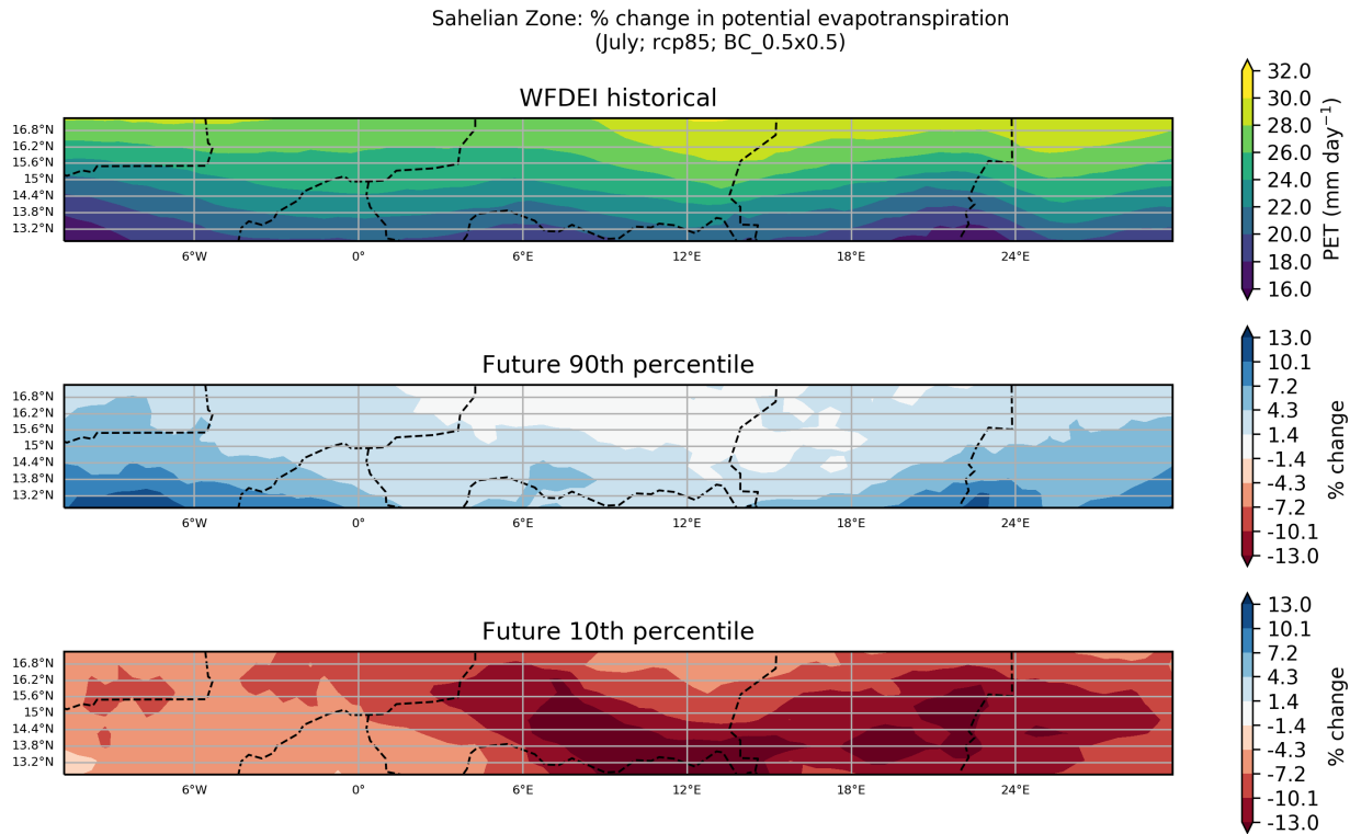
Figure 1: These maps show the ensemble spread in the percentage change in Potential Evapotranspiration for the period 2040 to 2059 (compared to a baseline period of 1950 - 2000) for the July season. They show the 90th and 10th percentiles of the distribution across the model ensemble, computed separately at each grid point, for the Sahelian Zone region. This particular plot shows the percentage change for the RCP8.5 scenario.
