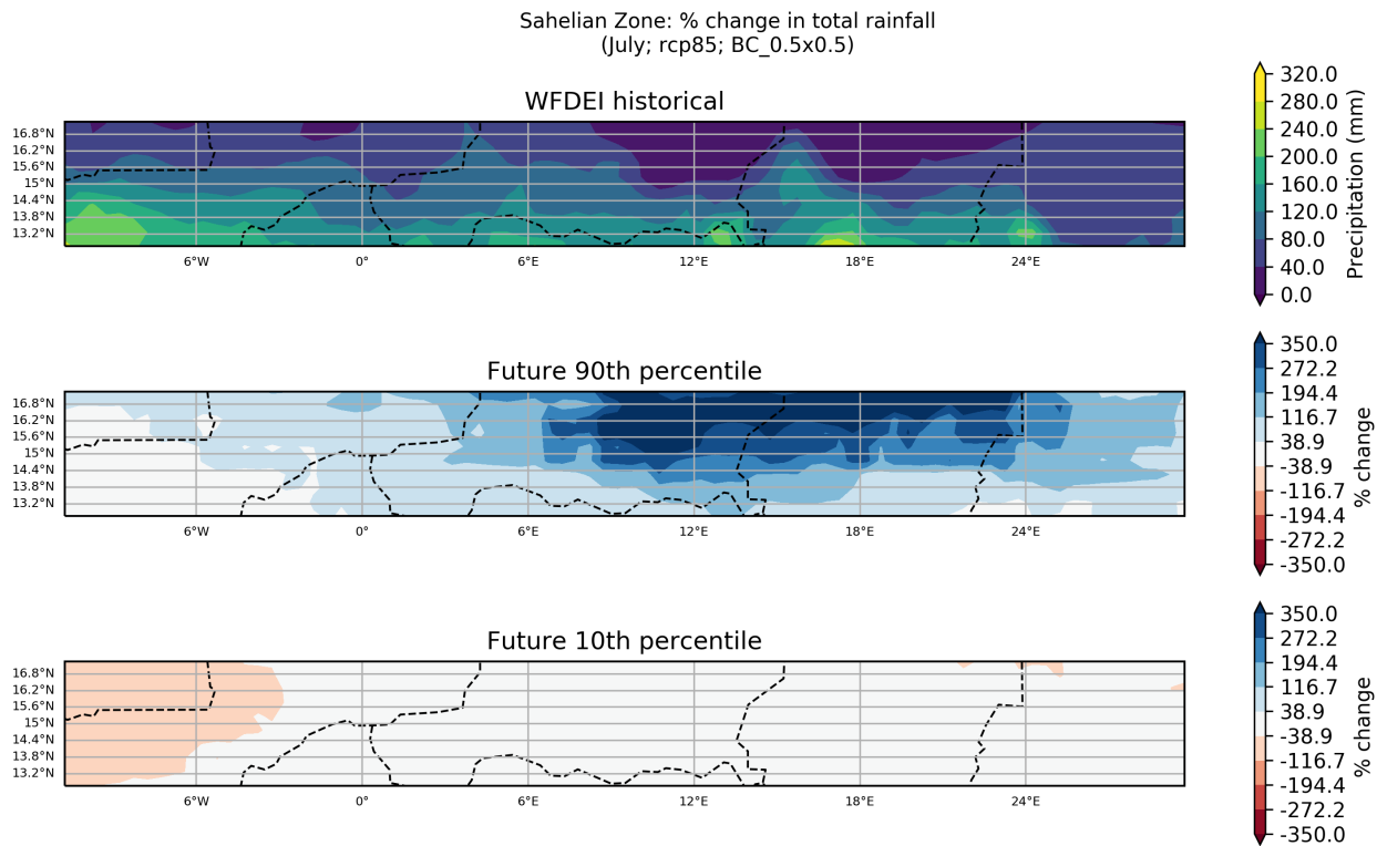
Figure 41: These maps show the ensemble spread in the percentage change in Total Rainfall for the period 2040 to 2059 (compared to a baseline period of 1950 - 2000) for the July season. They show the 90th and 10th percentiles of the distribution across the model ensemble, computed separately at each grid point, for the Sahelian Zone region. This particular plot shows the percentage change for the RCP8.5 scenario.
