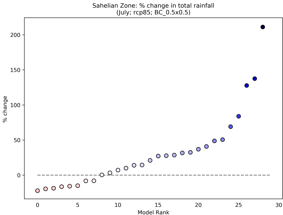
Figure 44: This scatterplot shows the percentage change in Total Rainfall for the period 2040 to 2059 (compared to a baseline period of 1950 - 2000) for the July season. Each data point shows an individual model averaged over Sahelian Zone, and ranked according to the magnitude of the value on the y-axis. This particular plot shows the percentage change for the RCP8.5 scenario.
