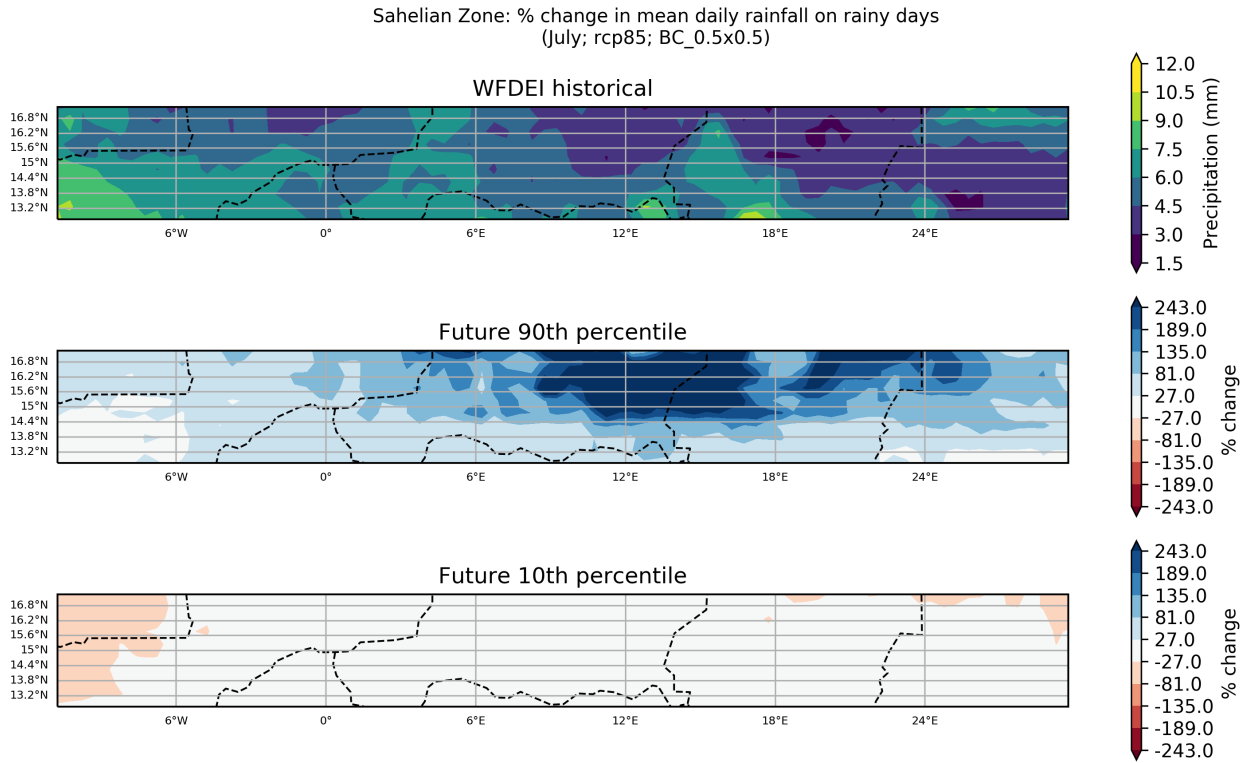
Figure 53: These maps show the ensemble spread in the percentage change in Mean Daily Rainfall on Rainy Days for the period 2040 to 2059 (compared to a baseline period of 1950 - 2000) for the July season. They show the 90th and 10th percentiles of the distribution across the model ensemble, computed separately at each grid point, for the Sahelian Zone region. This particular plot shows the percentage change for the RCP8.5 scenario.
