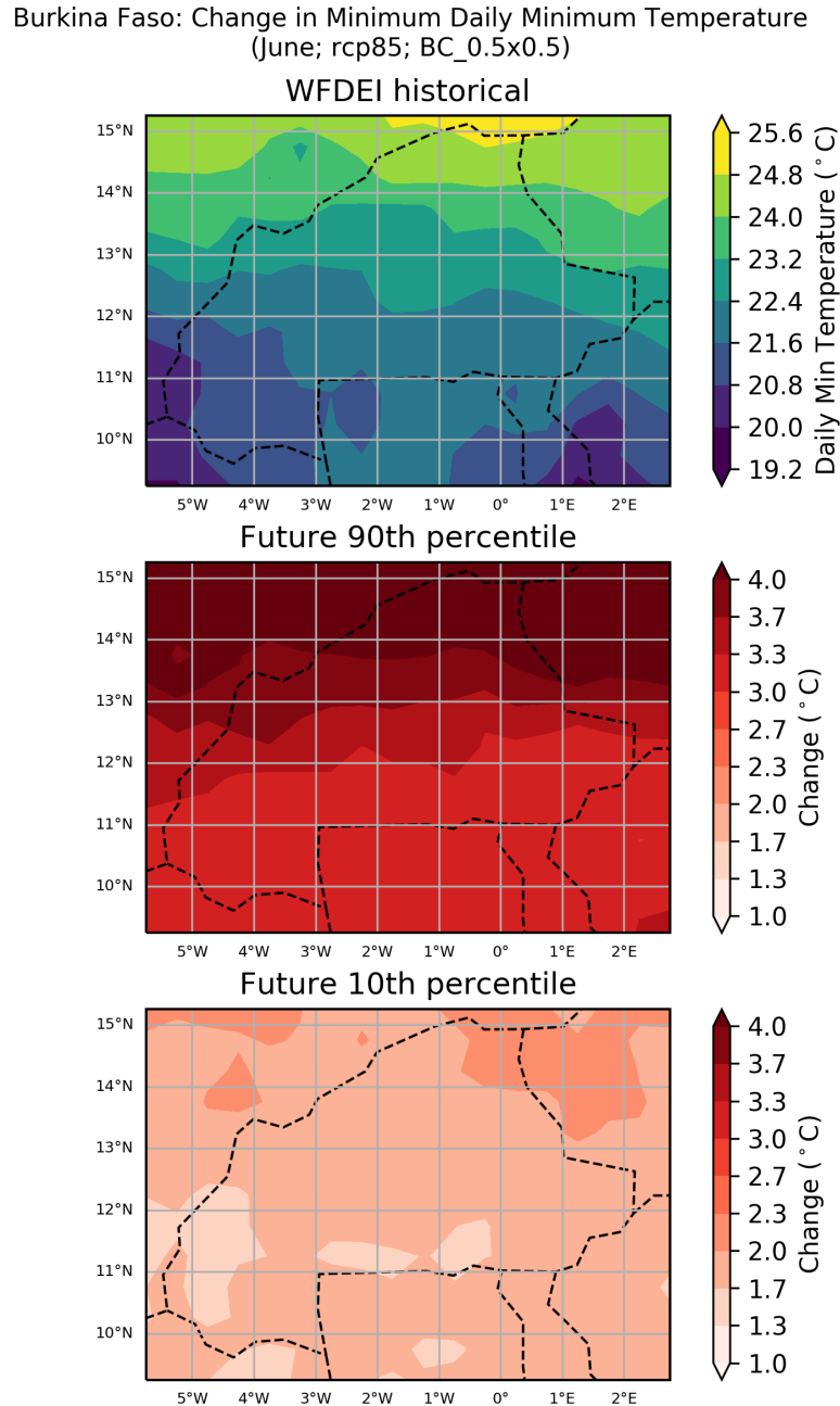
Figure 37: These maps show the ensemble spread in the absolute change in Minimum Daily Minimum Temperature for the period 2040 to 2059 (compared to a baseline period of 1950 - 2000) for the June season. They show the 90th and 10th percentiles of the distribution across the model ensemble, computed separately at each grid point, for the Burkina Faso region. This particular plot shows the absolute change for the RCP8.5 scenario.
