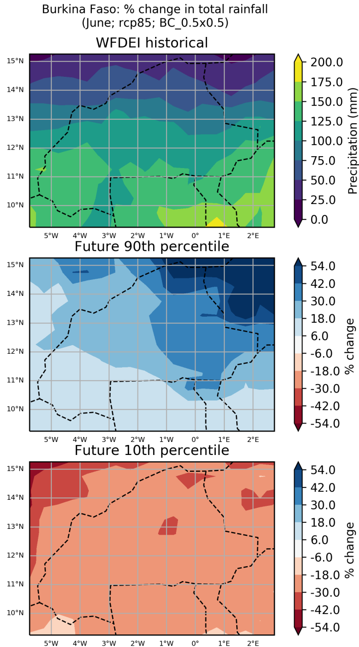
Figure 41: These maps show the ensemble spread in the percentage change in Total Rainfall for the period 2040 to 2059 (compared to a baseline period of 1950 - 2000) for the June season. They show the 90th and 10th percentiles of the distribution across the model ensemble, computed separately at each grid point, for the Burkina Faso region. This particular plot shows the percentage change for the RCP8.5 scenario.
