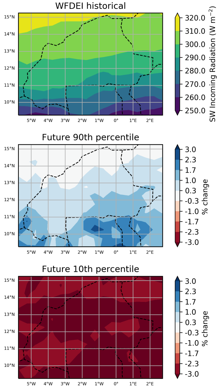
Burkina Faso: % change in Maximum Surface Downwelling Shortwave Radiation (June; rcp85; BC_0.5x0.5)
