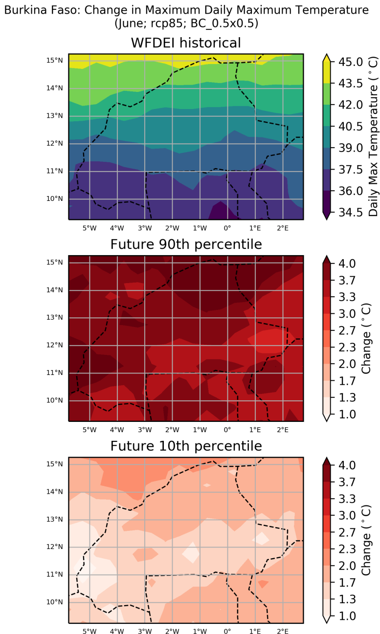
Figure 29: These maps show the ensemble spread in the absolute change in Maximum Daily Maximum Temperature for the period 2040 to 2059 (compared to a baseline period of 1950 - 2000) for the June season. They show the 90th and 10th percentiles of the distribution across the model ensemble, computed separately at each grid point, for the Burkina Faso region. This particular plot shows the absolute change for the RCP8.5 scenario.
