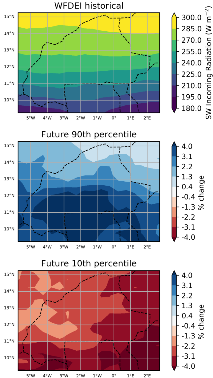
Burkina Faso: % change in Average Surface Downwelling Shortwave Radiation (June; rcp85; BC_0.5x0.5)
