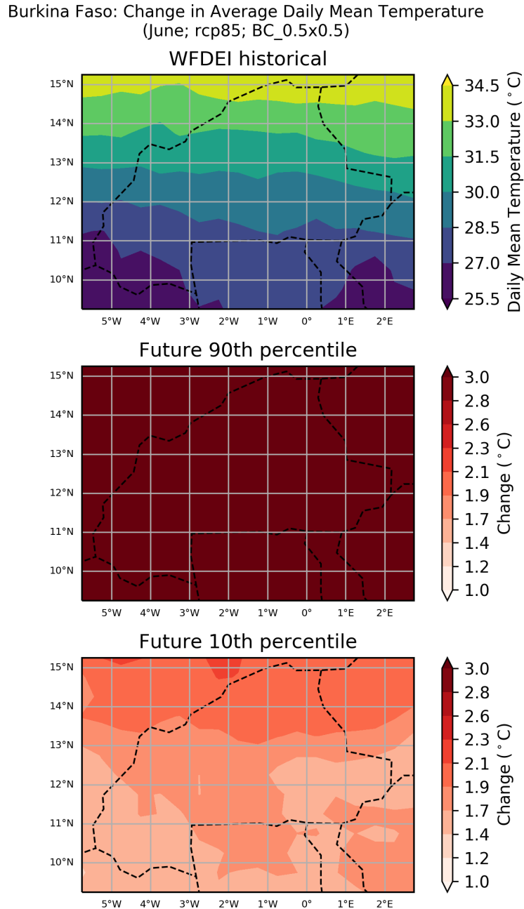
Figure 45: These maps show the ensemble spread in the absolute change in Average Daily Mean Temperature for the period 2040 to 2059 (compared to a baseline period of 1950 - 2000) for the June season. They show the 90th and 10th percentiles of the distribution across the model ensemble, computed separately at each grid point, for the Burkina Faso region. This particular plot shows the absolute change for the RCP8.5 scenario.
