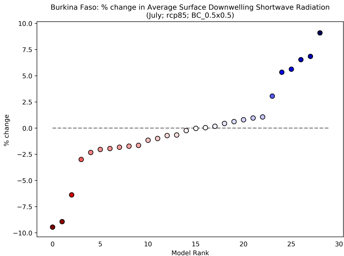
Figure 52: This scatterplot shows the percentage change in Average Surface Downwelling Shortwave Radiation for the period 2040 to 2059 (compared to a baseline period of 1950 - 2000) for the July season. Each data point shows an individual model averaged over Burkina Faso, and ranked according to the magnitude of the value on the y-axis. This particular plot shows the percentage change for the RCP8.5 scenario.
