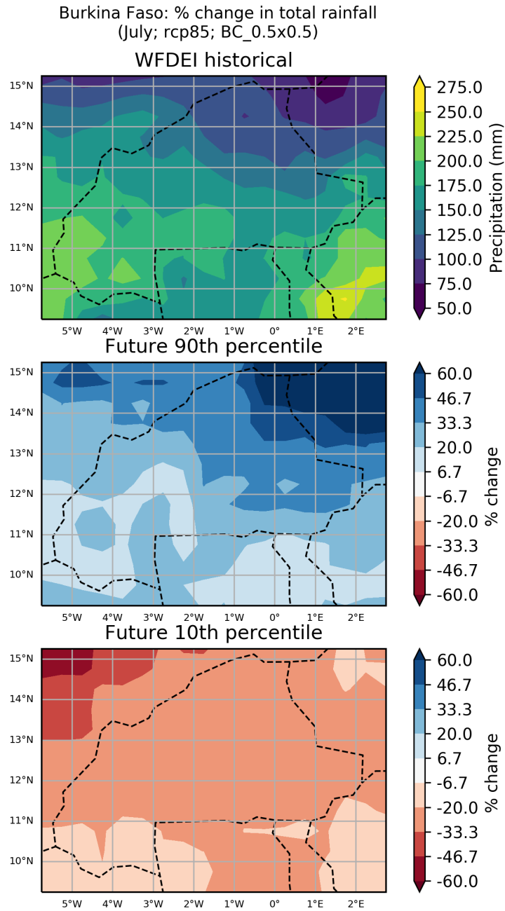
Figure 41: These maps show the ensemble spread in the percentage change in Total Rainfall for the period 2040 to 2059 (compared to a baseline period of 1950 - 2000) for the July season. They show the 90th and 10th percentiles of the distribution across the model ensemble, computed separately at each grid point, for the Burkina Faso region. This particular plot shows the percentage change for the RCP8.5 scenario.
