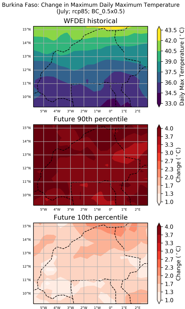
Figure 29: These maps show the ensemble spread in the absolute change in Maximum Daily Maximum Temperature for the period 2040 to 2059 (compared to a baseline period of 1950 - 2000) for the July season. They show the 90th and 10th percentiles of the distribution across the model ensemble, computed separately at each grid point, for the Burkina Faso region. This particular plot shows the absolute change for the RCP8.5 scenario.
