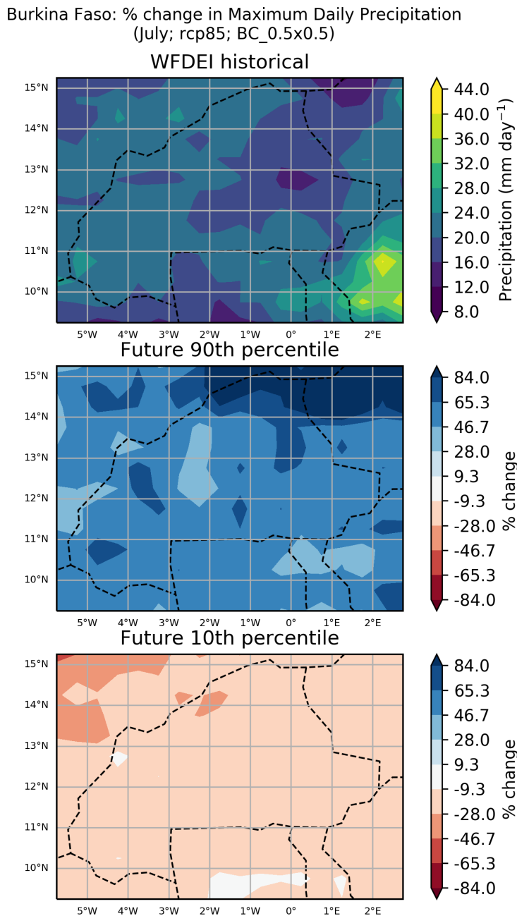
Figure 25: These maps show the ensemble spread in the percentage change in Maximum Daily Precipitation for the period 2040 to 2059 (compared to a baseline period of 1950 - 2000) for the July season. They show the 90th and 10th percentiles of the distribution across the model ensemble, computed separately at each grid point, for the Burkina Faso region. This particular plot shows the percentage change for the RCP8.5 scenario.
