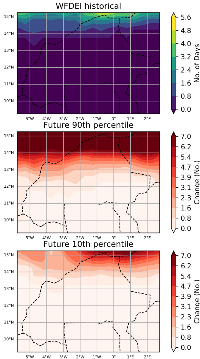
Figure 68: These maps show the ensemble spread in the absolute change in Number of Days with a Maximum Temperature > 40^{\circ}\text{C} for the period 2040 to 2059 (compared to a baseline period of 1950 - 2000) for the July season. They show the 90th and 10th percentiles of the distribution across the model ensemble, computed separately at each grid point, for the Burkina Faso region. This particular plot shows the absolute change for the RCP8.5 scenario.
