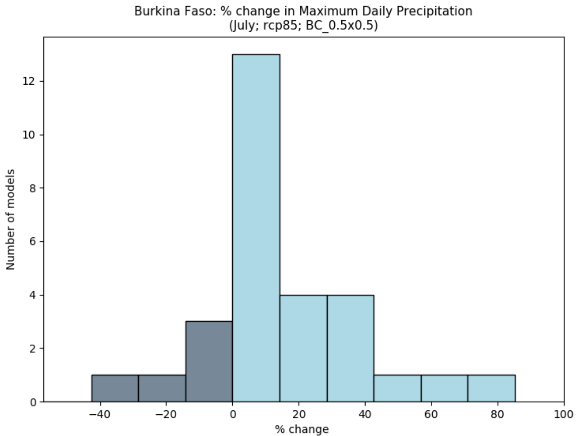
Figure 26: This histogram shows the number of models that agree on the percentage change in Maximum Daily Precipitation for the period 2040 to 2059 (compared to a baseline period of 1950 - 2000) for the July season. Each vertical bar shows the number of models that agree on the range of values shown on the x-axis for the Burkina Faso region. This particular plot shows the percentage change for the RCP8.5 scenario.
