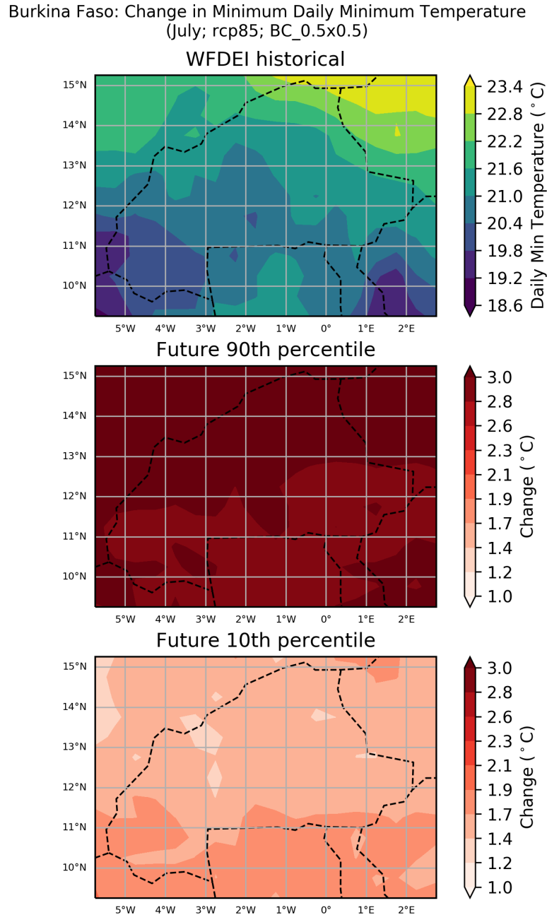
Figure 37: These maps show the ensemble spread in the absolute change in Minimum Daily Minimum Temperature for the period 2040 to 2059 (compared to a baseline period of 1950 - 2000) for the July season. They show the 90th and 10th percentiles of the distribution across the model ensemble, computed separately at each grid point, for the Burkina Faso region. This particular plot shows the absolute change for the RCP8.5 scenario.
