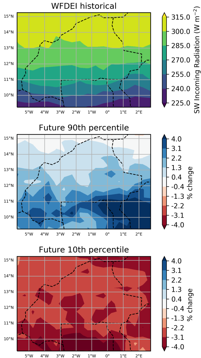
Burkina Faso: % change in Maximum Surface Downwelling Shortwave Radiation (July; rcp85; BC_0.5x0.5)
