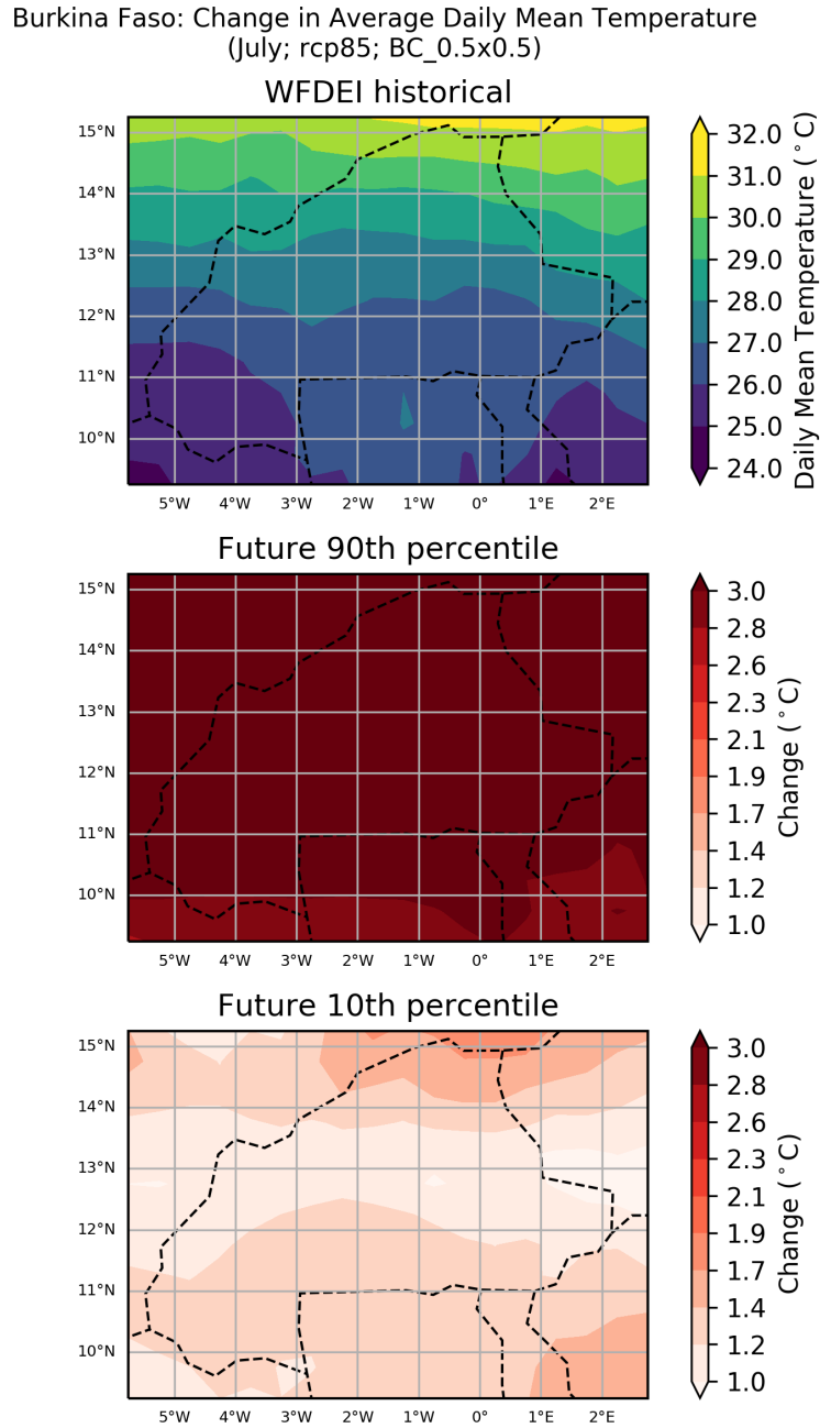
Figure 45: These maps show the ensemble spread in the absolute change in Average Daily Mean Temperature for the period 2040 to 2059 (compared to a baseline period of 1950 - 2000) for the July season. They show the 90th and 10th percentiles of the distribution across the model ensemble, computed separately at each grid point, for the Burkina Faso region. This particular plot shows the absolute change for the RCP8.5 scenario.
