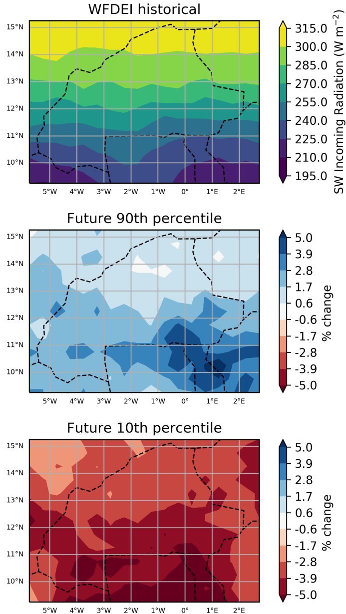
Burkina Faso: % change in Maximum Surface Downwelling Shortwave Radiation (August; rcp85; BC_0.5x0.5)
