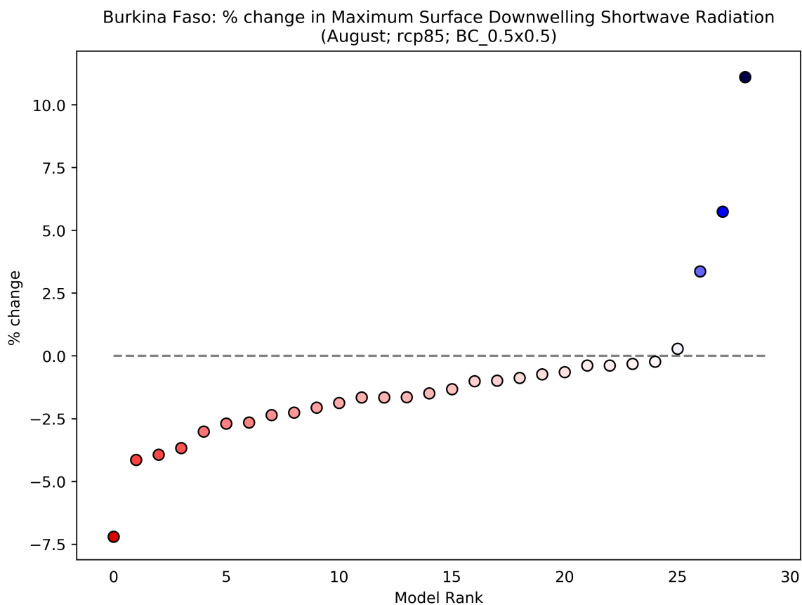
Figure 36: This scatterplot shows the percentage change in Maximum Surface Downwelling Shortwave Radiation for the period 2040 to 2059 (compared to a baseline period of 1950 - 2000) for the August season. Each data point shows an individual model averaged over Burkina Faso, and ranked according to the magnitude of the value on the y-axis. This particular plot shows the percentage change for the RCP8.5 scenario.
