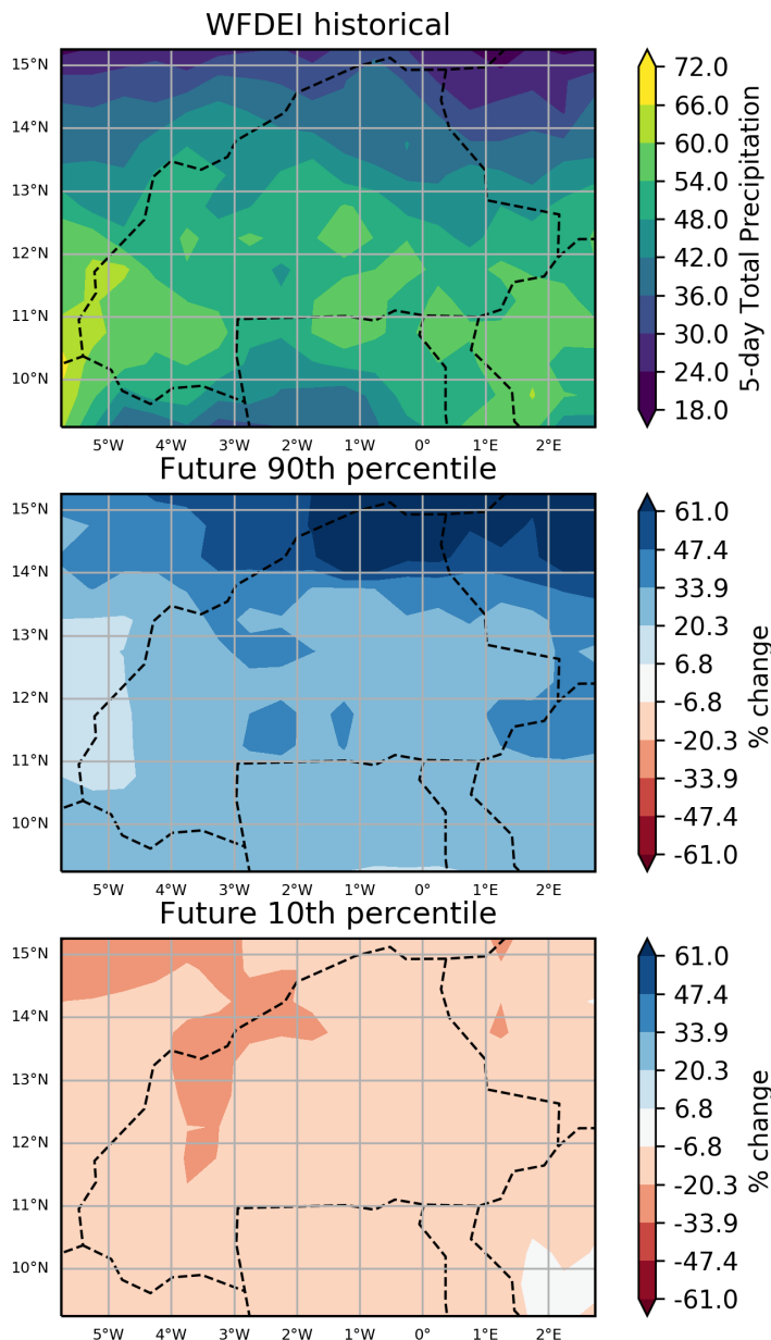
Figure 80: These maps show the ensemble spread in the percentage change in Maximum Rainfall Total in a 5-day Period for the period 2040 to 2059 (compared to a baseline period of 1950 - 2000) for the August season. They show the 90th and 10th percentiles of the distribution across the model ensemble, computed separately at each grid point, for the Burkina Faso region. This particular plot shows the percentage change for the RCP8.5 scenario.
