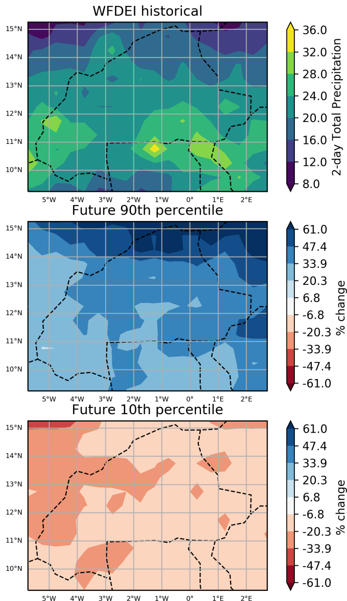
Figure 88: These maps show the ensemble spread in the percentage change in Maximum Rainfall Total in a 2-day Period for the period 2040 to 2059 (compared to a baseline period of 1950 - 2000) for the August season. They show the 90th and 10th percentiles of the distribution across the model ensemble, computed separately at each grid point, for the Burkina Faso region. This particular plot shows the percentage change for the RCP8.5 scenario.
