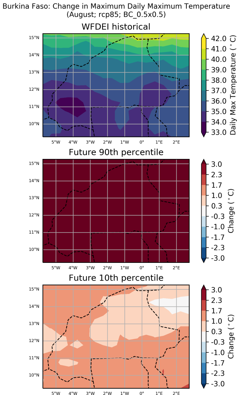
Figure 29: These maps show the ensemble spread in the absolute change in Maximum Daily Maximum Temperature for the period 2040 to 2059 (compared to a baseline period of 1950 - 2000) for the August season. They show the 90th and 10th percentiles of the distribution across the model ensemble, computed separately at each grid point, for the Burkina Faso region. This particular plot shows the absolute change for the RCP8.5 scenario.
