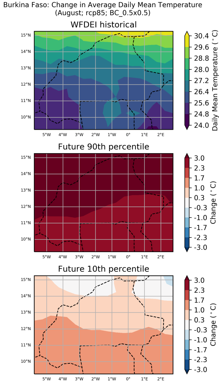
Figure 45: These maps show the ensemble spread in the absolute change in Average Daily Mean Temperature for the period 2040 to 2059 (compared to a baseline period of 1950 - 2000) for the August season. They show the 90th and 10th percentiles of the distribution across the model ensemble, computed separately at each grid point, for the Burkina Faso region. This particular plot shows the absolute change for the RCP8.5 scenario.
