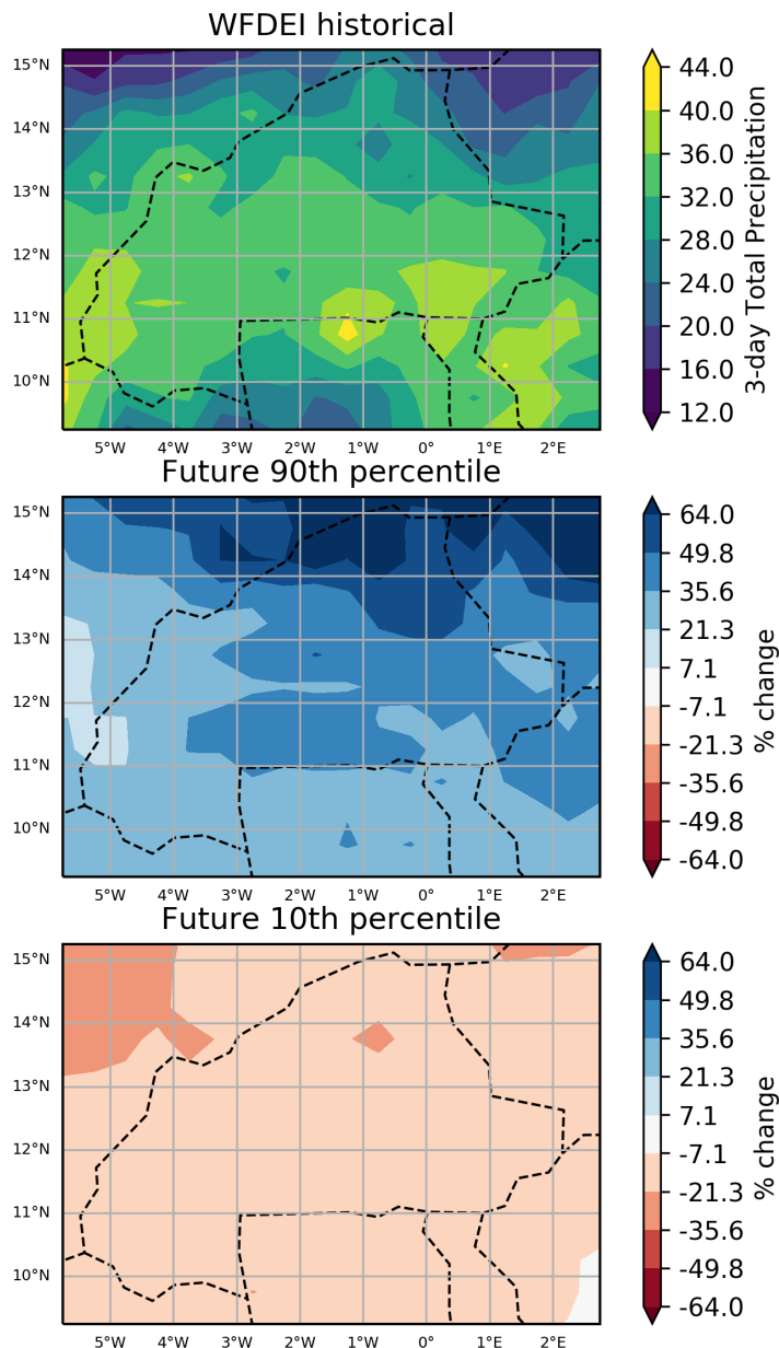
Figure 84: These maps show the ensemble spread in the percentage change in Maximum Rainfall Total in a 3-day Period for the period 2040 to 2059 (compared to a baseline period of 1950 - 2000) for the August season. They show the 90th and 10th percentiles of the distribution across the model ensemble, computed separately at each grid point, for the Burkina Faso region. This particular plot shows the percentage change for the RCP8.5 scenario.
