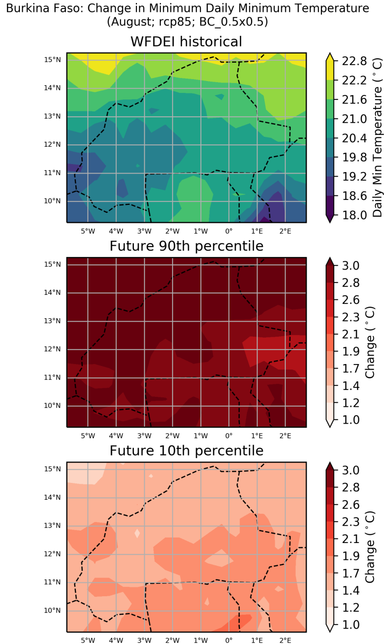
Figure 37: These maps show the ensemble spread in the absolute change in Minimum Daily Minimum Temperature for the period 2040 to 2059 (compared to a baseline period of 1950 - 2000) for the August season. They show the 90th and 10th percentiles of the distribution across the model ensemble, computed separately at each grid point, for the Burkina Faso region. This particular plot shows the absolute change for the RCP8.5 scenario.
