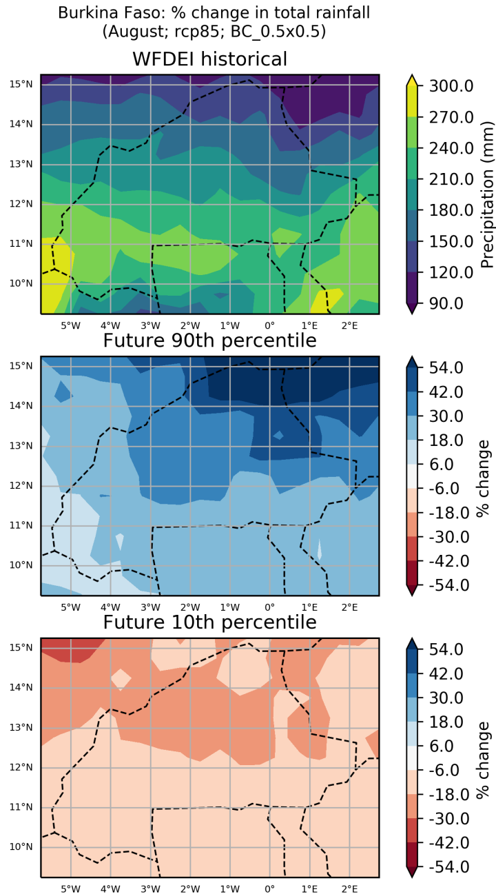
Figure 41: These maps show the ensemble spread in the percentage change in Total Rainfall for the period 2040 to 2059 (compared to a baseline period of 1950 - 2000) for the August season. They show the 90th and 10th percentiles of the distribution across the model ensemble, computed separately at each grid point, for the Burkina Faso region. This particular plot shows the percentage change for the RCP8.5 scenario.
