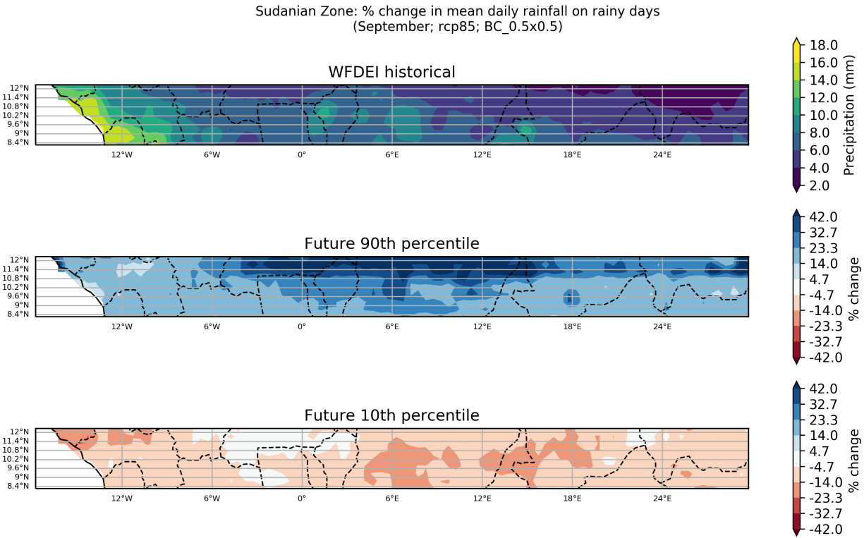
Figure 53: These maps show the ensemble spread in the percentage change in Mean Daily Rainfall on Rainy Days for the period 2040 to 2059 (compared to a baseline period of 1950 - 2000) for the September season. They show the 90th and 10th percentiles of the distribution across the model ensemble, computed separately at each grid point, for the Sudanian Zone region. This particular plot shows the percentage change for the RCP8.5 scenario.
