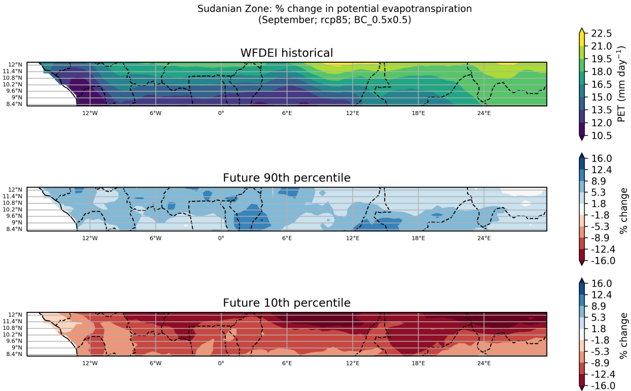
Figure 1: These maps show the ensemble spread in the percentage change in Potential Evapotranspiration for the period 2040 to 2059 (compared to a baseline period of 1950 - 2000) for the September season. They show the 90th and 10th percentiles of the distribution across the model ensemble, computed separately at each grid point, for the Sudanian Zone region. This particular plot shows the percentage change for the RCP8.5 scenario.
