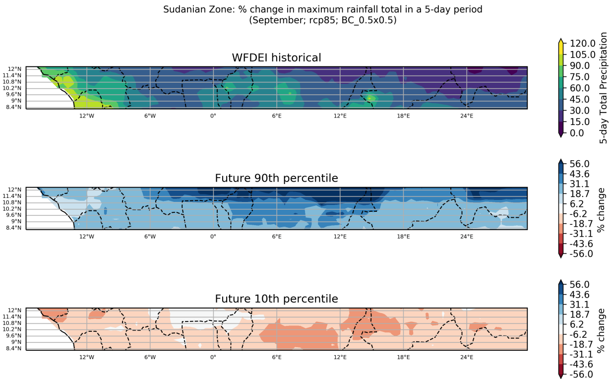
Figure 80: These maps show the ensemble spread in the percentage change in Maximum Rainfall Total in a 5-day Period for the period 2040 to 2059 (compared to a baseline period of 1950 - 2000) for the September season. They show the 90th and 10th percentiles of the distribution across the model ensemble, computed separately at each grid point, for the Sudanian Zone region. This particular plot shows the percentage change for the RCP8.5 scenario.
