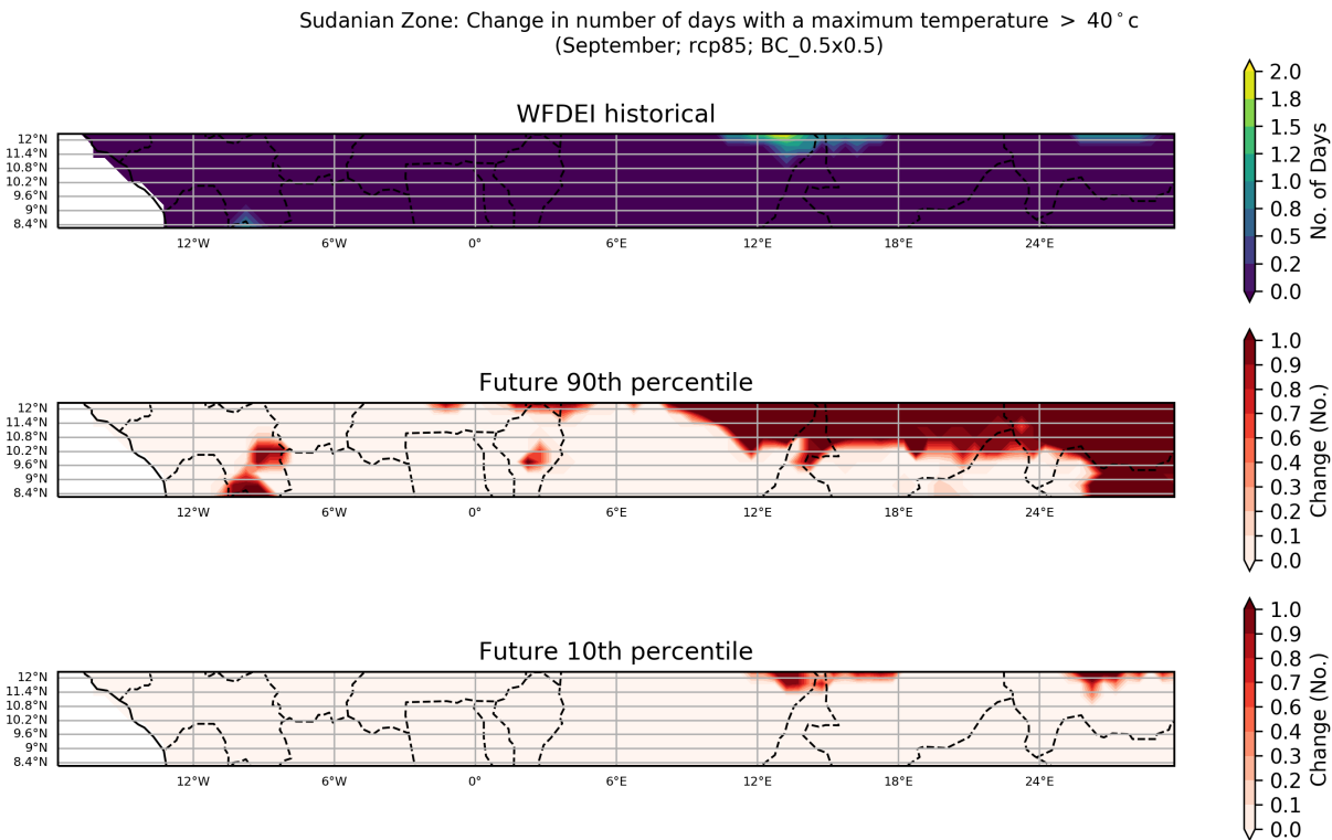
Figure 68: These maps show the ensemble spread in the absolute change in Number of Days with a Maximum Temperature > 40°C for the period 2040 to 2059 (compared to a baseline period of 1950 - 2000) for the September season. They show the 90th and 10th percentiles of the distribution across the model ensemble, computed separately at each grid point, for the Sudanian Zone region. This particular plot shows the absolute change for the RCP8.5 scenario.
