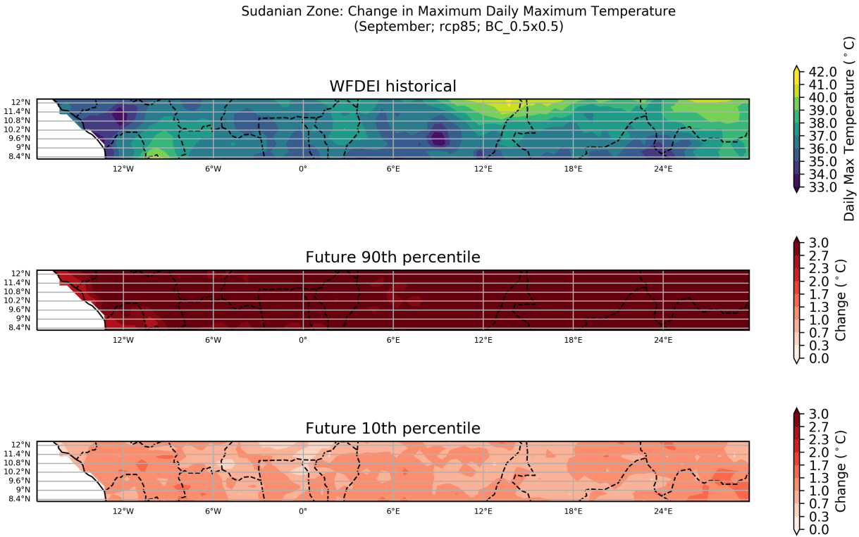
Figure 29: These maps show the ensemble spread in the absolute change in Maximum Daily Maximum Temperature for the period 2040 to 2059 (compared to a baseline period of 1950 - 2000) for the September season. They show the 90th and 10th percentiles of the distribution across the model ensemble, computed separately at each grid point, for the Sudanian Zone region. This particular plot shows the absolute change for the RCP8.5 scenario.
