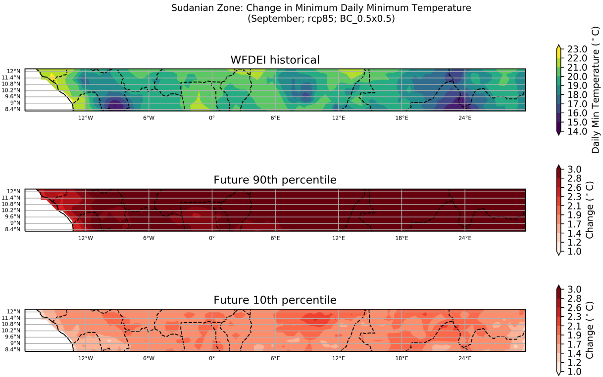
Figure 37: These maps show the ensemble spread in the absolute change in Minimum Daily Minimum Temperature for the period 2040 to 2059 (compared to a baseline period of 1950 - 2000) for the September season. They show the 90th and 10th percentiles of the distribution across the model ensemble, computed separately at each grid point, for the Sudanian Zone region. This particular plot shows the absolute change for the RCP8.5 scenario.
