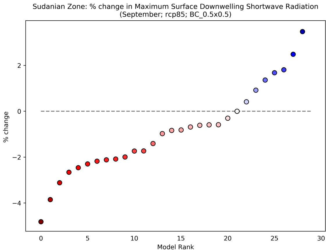
Figure 36: This scatterplot shows the percentage change in Maximum Surface Downwelling Shortwave Radiation for the period 2040 to 2059 (compared to a baseline period of 1950 - 2000) for the September season. Each data point shows an individual model averaged over Sudanian Zone, and ranked according to the magnitude of the value on the y-axis. This particular plot shows the percentage change for the RCP8.5 scenario.
