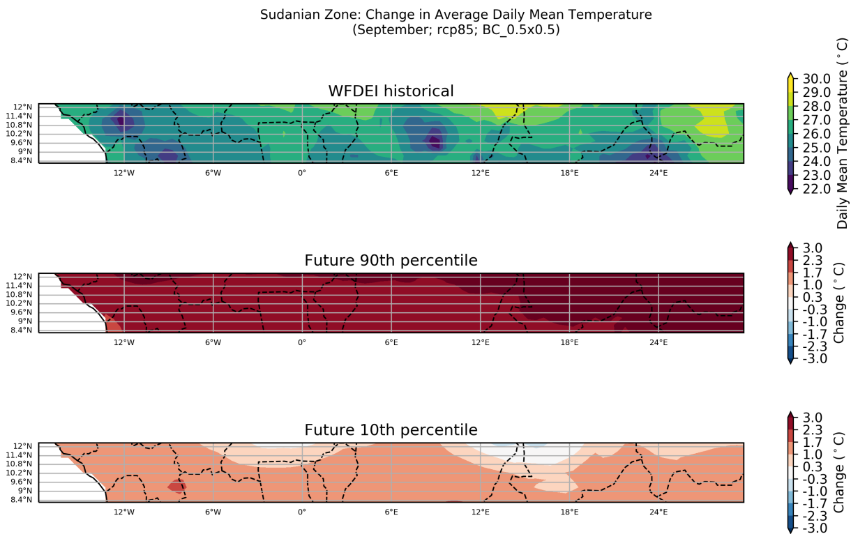
Figure 45: These maps show the ensemble spread in the absolute change in Average Daily Mean Temperature for the period 2040 to 2059 (compared to a baseline period of 1950 - 2000) for the September season. They show the 90th and 10th percentiles of the distribution across the model ensemble, computed separately at each grid point, for the Sudanian Zone region. This particular plot shows the absolute change for the RCP8.5 scenario.
