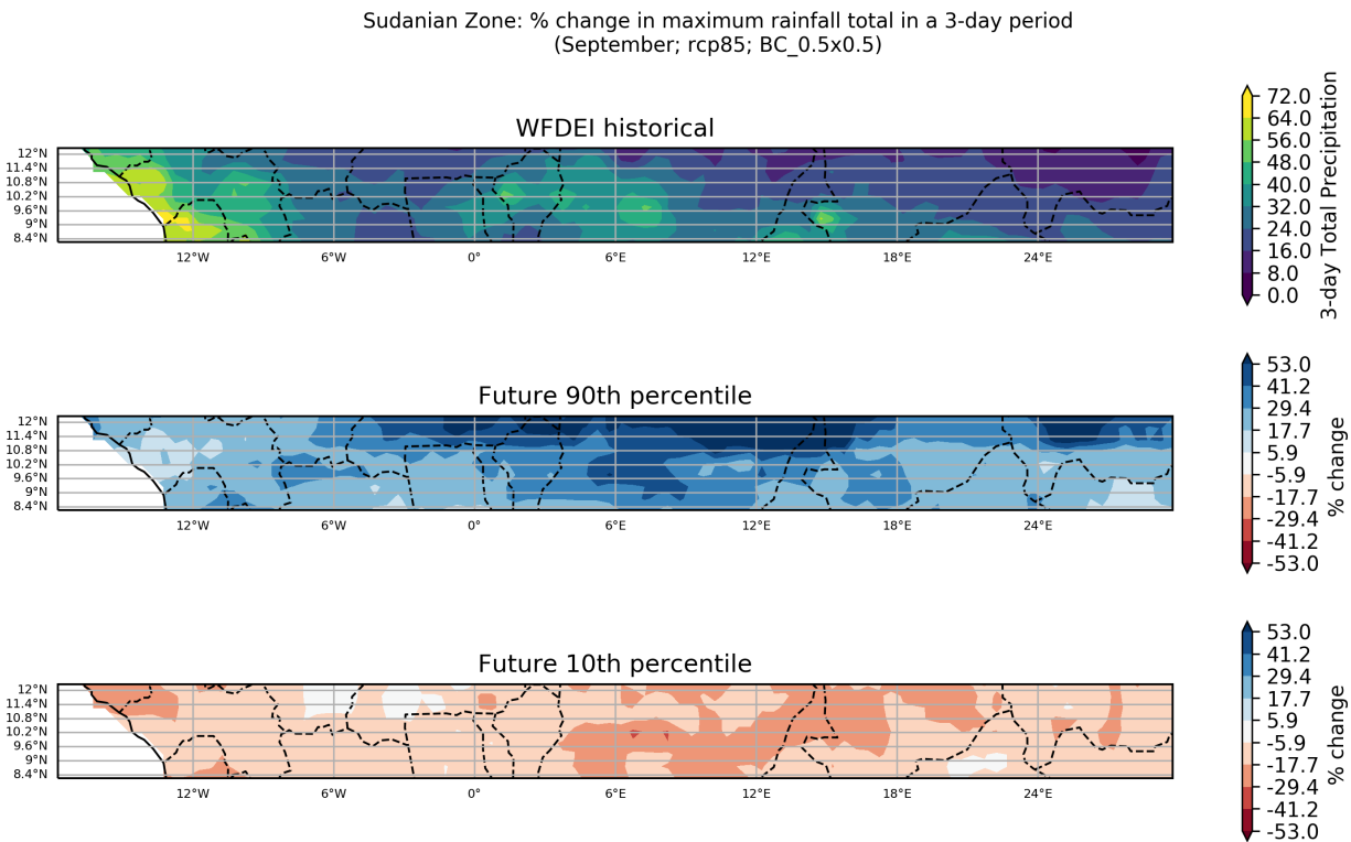
Figure 84: These maps show the ensemble spread in the percentage change in Maximum Rainfall Total in a 3-day Period for the period 2040 to 2059 (compared to a baseline period of 1950 - 2000) for the September season. They show the 90th and 10th percentiles of the distribution across the model ensemble, computed separately at each grid point, for the Sudanian Zone region. This particular plot shows the percentage change for the RCP8.5 scenario.
