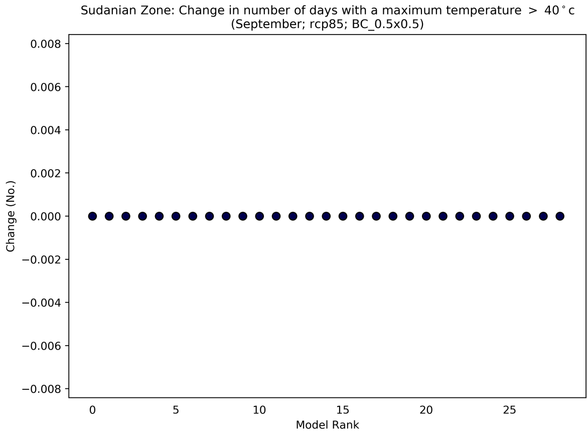
Figure 71: This scatterplot shows the absolute change in Number of Days with a Maximum Temperature > 40°C for the period 2040 to 2059 (compared to a baseline period of 1950 - 2000) for the September season. Each data point shows an individual model averaged over Sudanian Zone, and ranked according to the magnitude of the value on the y-axis. This particular plot shows the absolute change for the RCP8.5 scenario.
