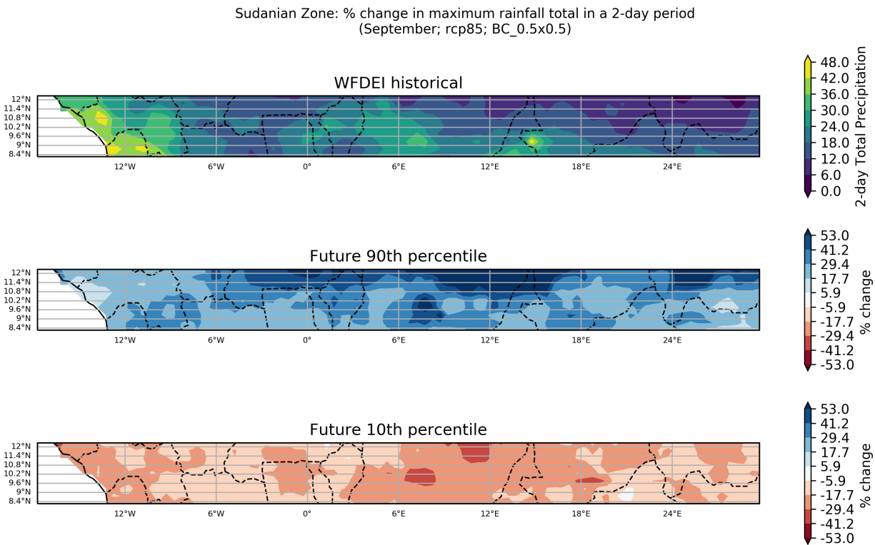
Figure 88: These maps show the ensemble spread in the percentage change in Maximum Rainfall Total in a 2-day Period for the period 2040 to 2059 (compared to a baseline period of 1950 - 2000) for the September season. They show the 90th and 10th percentiles of the distribution across the model ensemble, computed separately at each grid point, for the Sudanian Zone region. This particular plot shows the percentage change for the RCP8.5 scenario.
