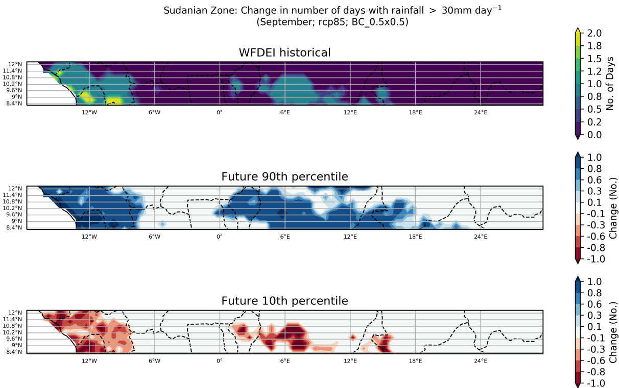
Figure 72: These maps show the ensemble spread in the absolute change in Number of Days with Rainfall > 30mm day -1 for the period 2040 to 2059 (compared to a baseline period of 1950 - 2000) for the September season. They show the 90th and 10th percentiles of the distribution across the model ensemble, computed separately at each grid point, for the Sudanian Zone region. This particular plot shows the absolute change for the RCP8.5 scenario.
