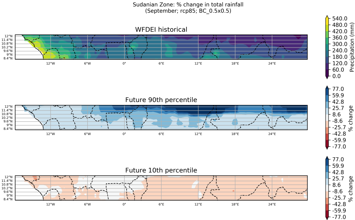
Figure 41: These maps show the ensemble spread in the percentage change in Total Rainfall for the period 2040 to 2059 (compared to a baseline period of 1950 - 2000) for the September season. They show the 90th and 10th percentiles of the distribution across the model ensemble, computed separately at each grid point, for the Sudanian Zone region. This particular plot shows the percentage change for the RCP8.5 scenario.
