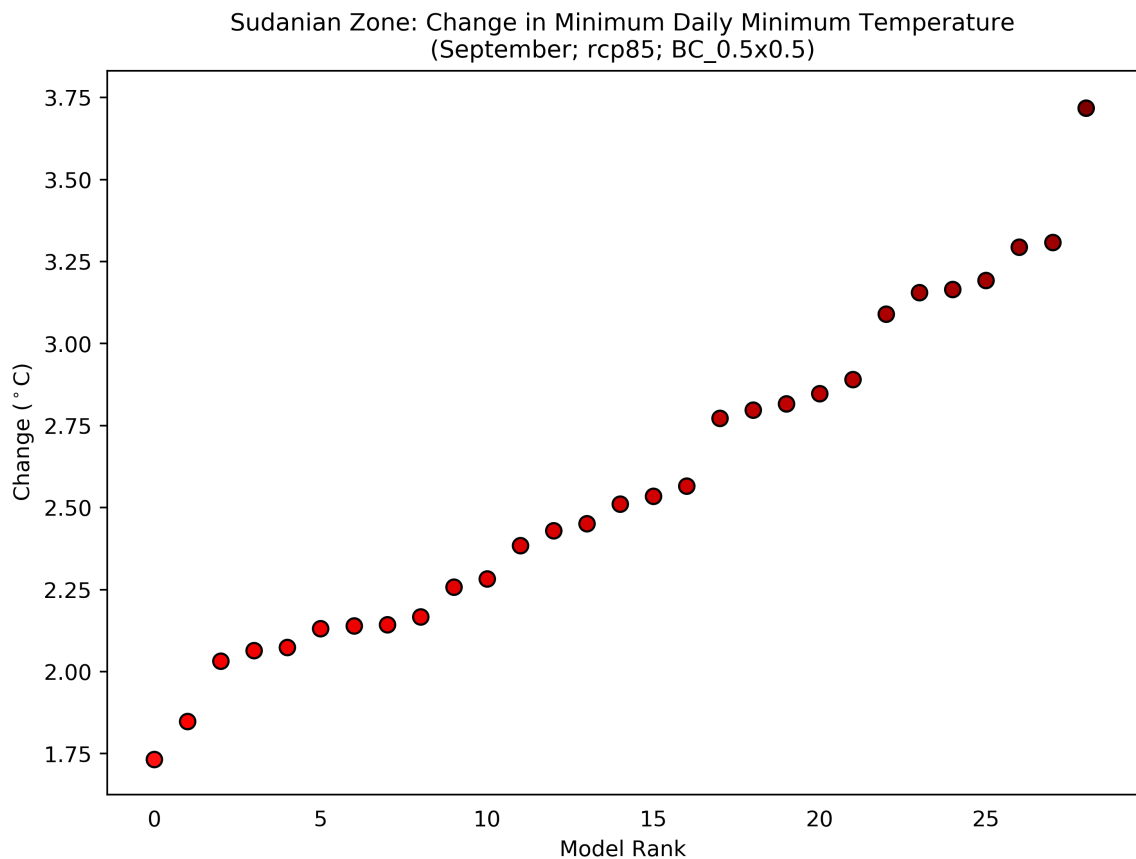
Figure 40: This scatterplot shows the absolute change in Minimum Daily Minimum Temperature for the period 2040 to 2059 (compared to a baseline period of 1950 - 2000) for the September season. Each data point shows an individual model averaged over Sudanian Zone, and ranked according to the magnitude of the value on the y-axis. This particular plot shows the absolute change for the RCP8.5 scenario.
