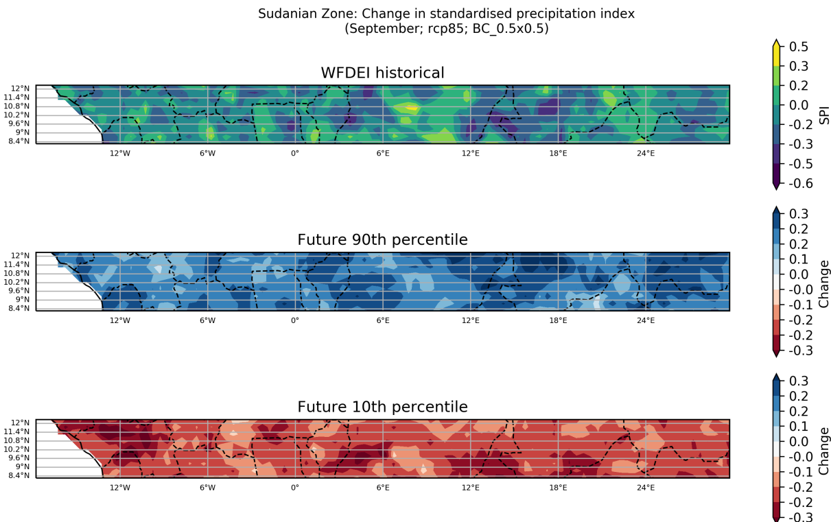
Figure 9: These maps show the ensemble spread in the absolute change in Standardised Precipitation Index for the period 2040 to 2059 (compared to a baseline period of 1950 - 2000) for the September season. They show the 90th and 10th percentiles of the distribution across the model ensemble, computed separately at each grid point, for the Sudanian Zone region. This particular plot shows the absolute change for the RCP8.5 scenario.
