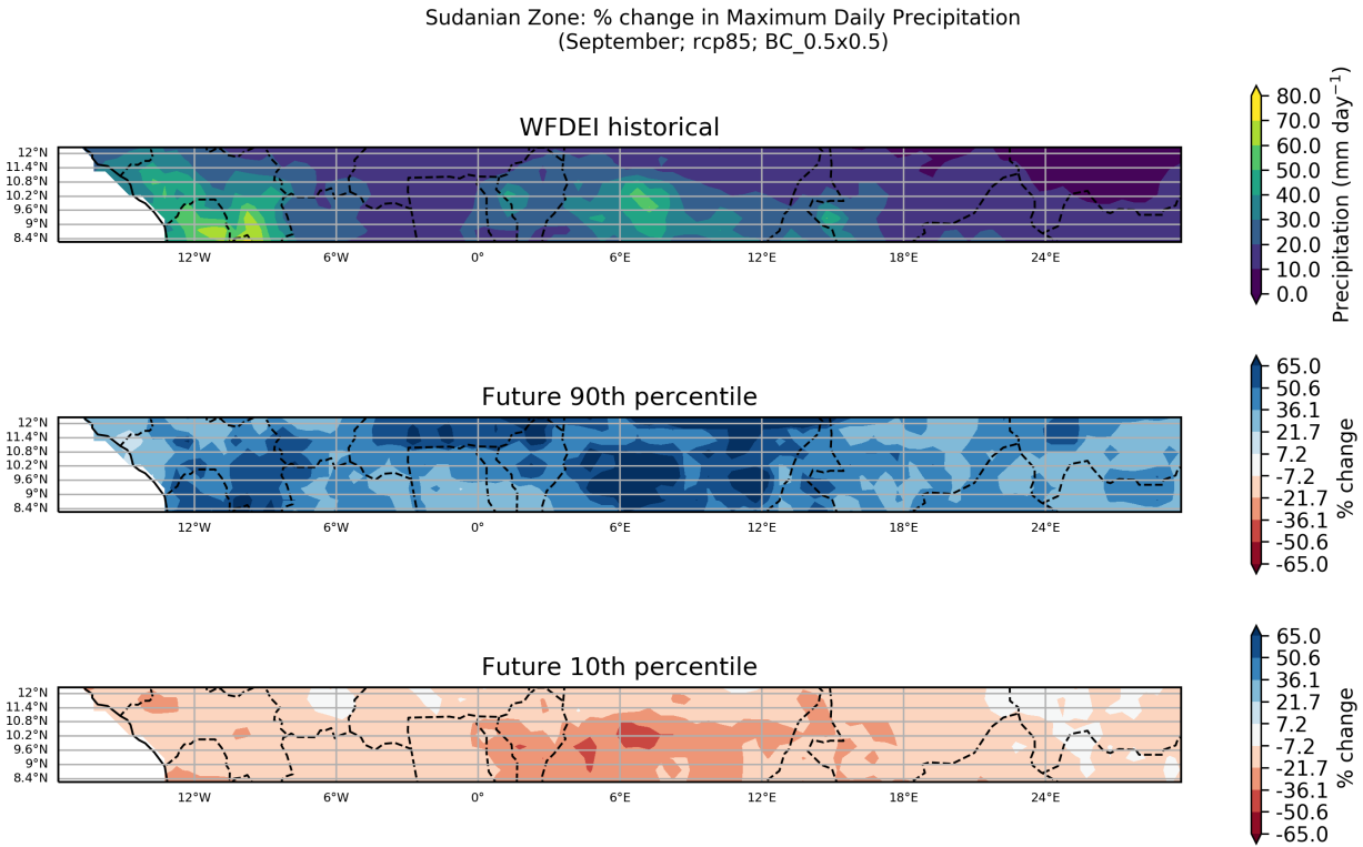
Figure 25: These maps show the ensemble spread in the percentage change in Maximum Daily Precipitation for the period 2040 to 2059 (compared to a baseline period of 1950 - 2000) for the September season. They show the 90th and 10th percentiles of the distribution across the model ensemble, computed separately at each grid point, for the Sudanian Zone region. This particular plot shows the percentage change for the RCP8.5 scenario.
