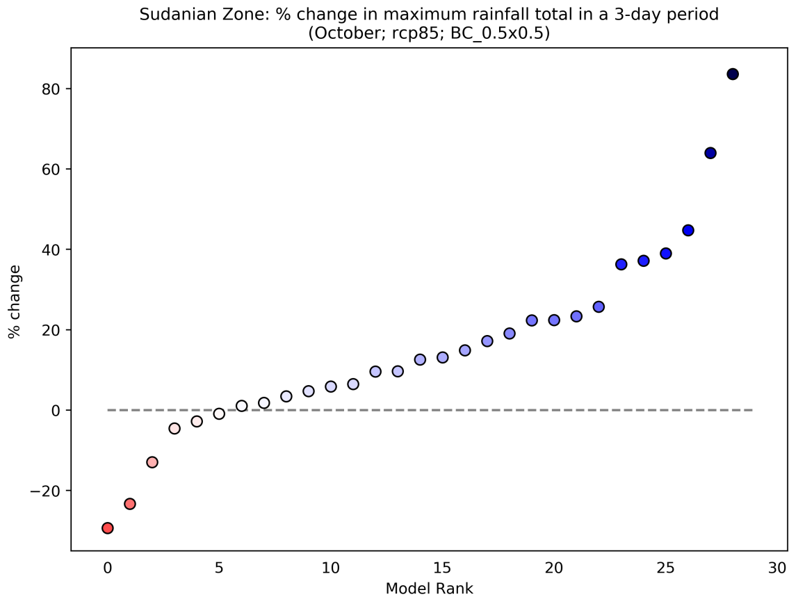
Figure 87: This scatterplot shows the percentage change in Maximum Rainfall Total in a 3-day Period for the period 2040 to 2059 (compared to a baseline period of 1950 - 2000) for the October season. Each data point shows an individual model averaged over Sudanian Zone, and ranked according to the magnitude of the value on the y-axis. This particular plot shows the percentage change for the RCP8.5 scenario.
