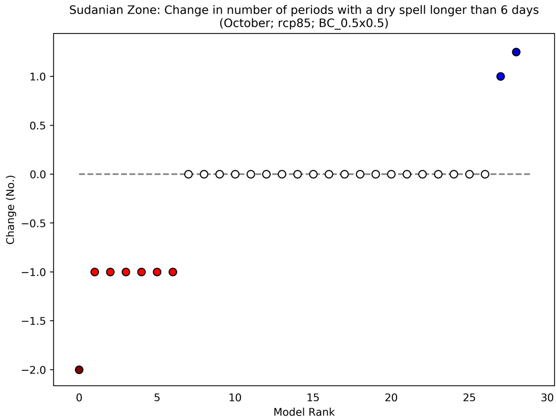
Figure 24: This scatterplot shows the absolute change in Number of Periods with a Dry Spell Longer Than 6 Days for the period 2040 to 2059 (compared to a baseline period of 1950 - 2000) for the October season. Each data point shows an individual model averaged over Sudanian Zone, and ranked according to the magnitude of the value on the y-axis. This particular plot shows the absolute change for the RCP8.5 scenario.
