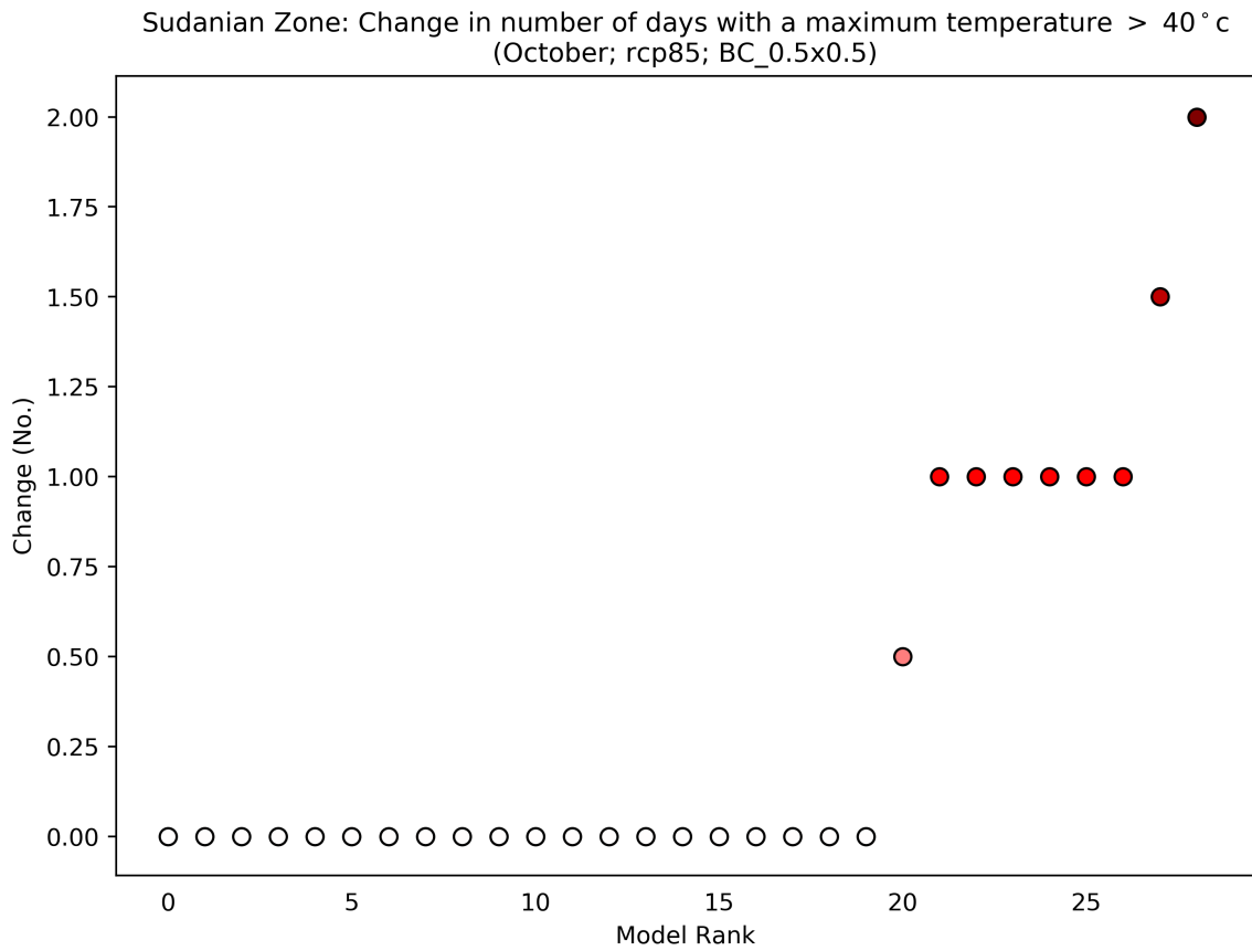
Figure 71: This scatterplot shows the absolute change in Number of Days with a Maximum Temperature > 40°C for the period 2040 to 2059 (compared to a baseline period of 1950 - 2000) for the October season. Each data point shows an individual model averaged over Sudanian Zone, and ranked according to the magnitude of the value on the y-axis. This particular plot shows the absolute change for the RCP8.5 scenario.
