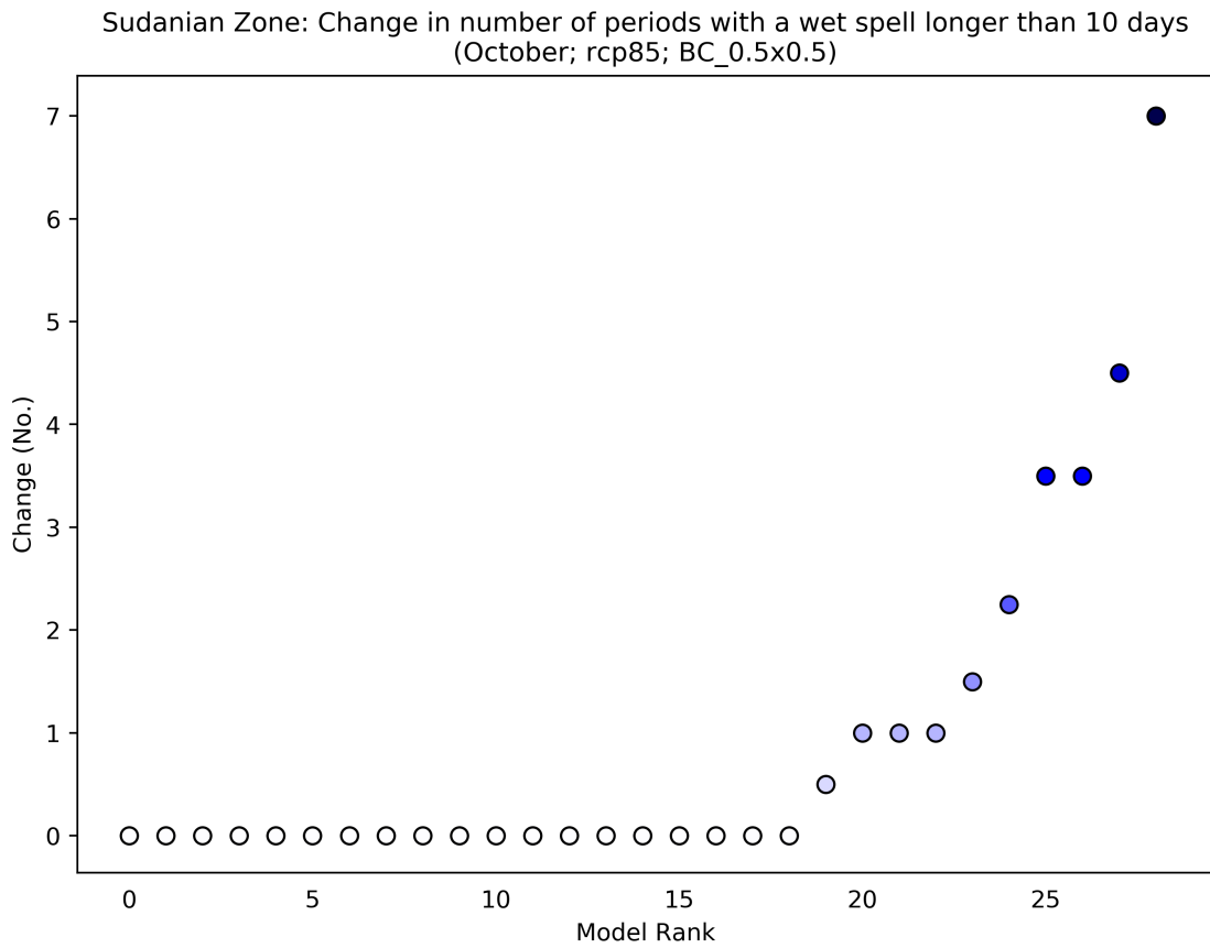
Figure 20: This scatterplot shows the absolute change in Number of Periods with a Wet Spell Longer Than 10 Days for the period 2040 to 2059 (compared to a baseline period of 1950 - 2000) for the October season. Each data point shows an individual model averaged over Sudanian Zone, and ranked according to the magnitude of the value on the y-axis. This particular plot shows the absolute change for the RCP8.5 scenario.
