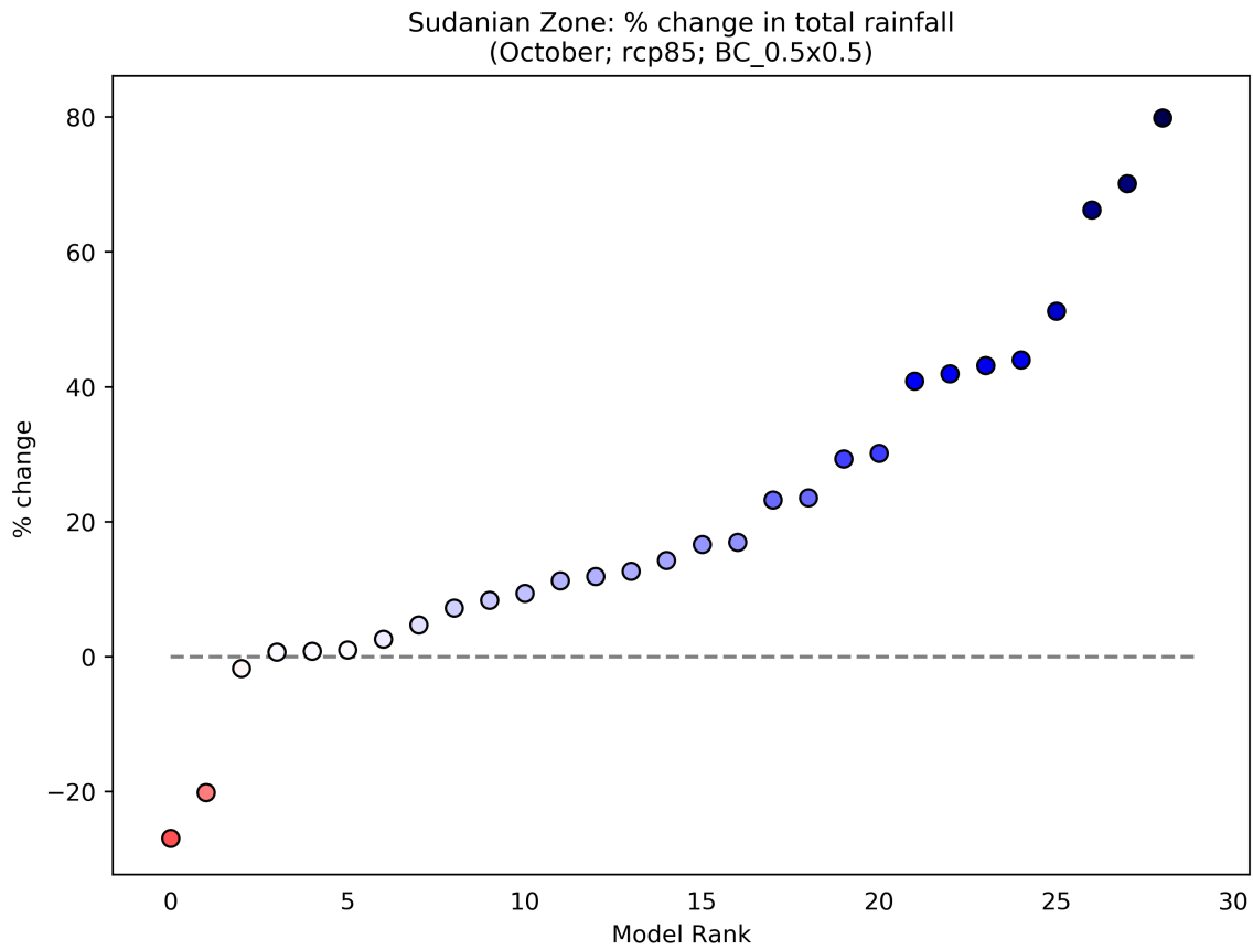
Figure 44: This scatterplot shows the percentage change in Total Rainfall for the period 2040 to 2059 (compared to a baseline period of 1950 - 2000) for the October season. Each data point shows an individual model averaged over Sudanian Zone, and ranked according to the magnitude of the value on the y-axis. This particular plot shows the percentage change for the RCP8.5 scenario.
