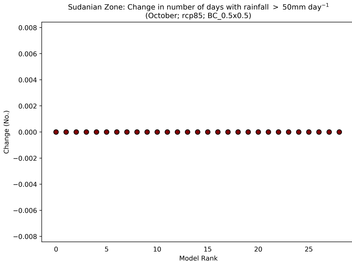
Figure 79: This scatterplot shows the absolute change in Number of Days with Rainfall > 50mm day -1 for the period 2040 to 2059 (compared to a baseline period of 1950 - 2000) for the October season. Each data point shows an individual model averaged over Sudanian Zone, and ranked according to the magnitude of the value on the y-axis. This particular plot shows the absolute change for the RCP8.5 scenario.
