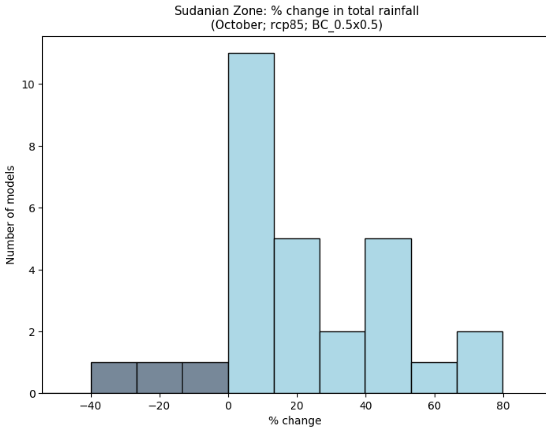
Figure 42: This histogram shows the number of models that agree on the percentage change in Total Rainfall for the period 2040 to 2059 (compared to a baseline period of 1950 - 2000) for the October season. Each vertical bar shows the number of models that agree on the range of values shown on the x-axis for the Sudanian Zone region. This particular plot shows the percentage change for the RCP8.5 scenario.
