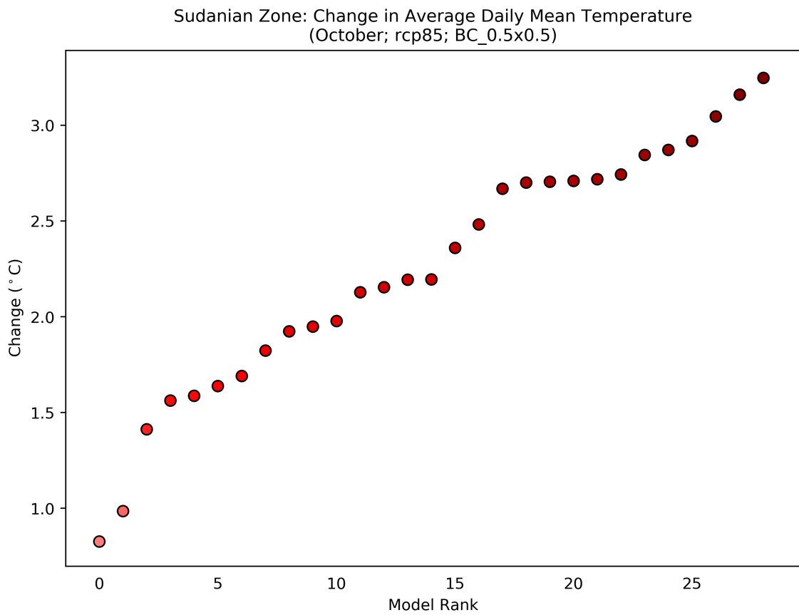
Figure 48: This scatterplot shows the absolute change in Average Daily Mean Temperature for the period 2040 to 2059 (compared to a baseline period of 1950 - 2000) for the October season. Each data point shows an individual model averaged over Sudanian Zone, and ranked according to the magnitude of the value on the y-axis. This particular plot shows the absolute change for the RCP8.5 scenario.
