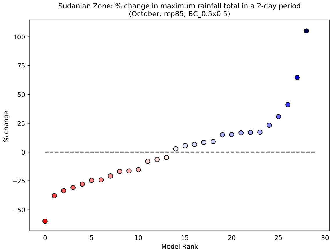
Figure 91: This scatterplot shows the percentage change in Maximum Rainfall Total in a 2-day Period for the period 2040 to 2059 (compared to a baseline period of 1950 - 2000) for the October season. Each data point shows an individual model averaged over Sudanian Zone, and ranked according to the magnitude of the value on the y-axis. This particular plot shows the percentage change for the RCP8.5 scenario.
