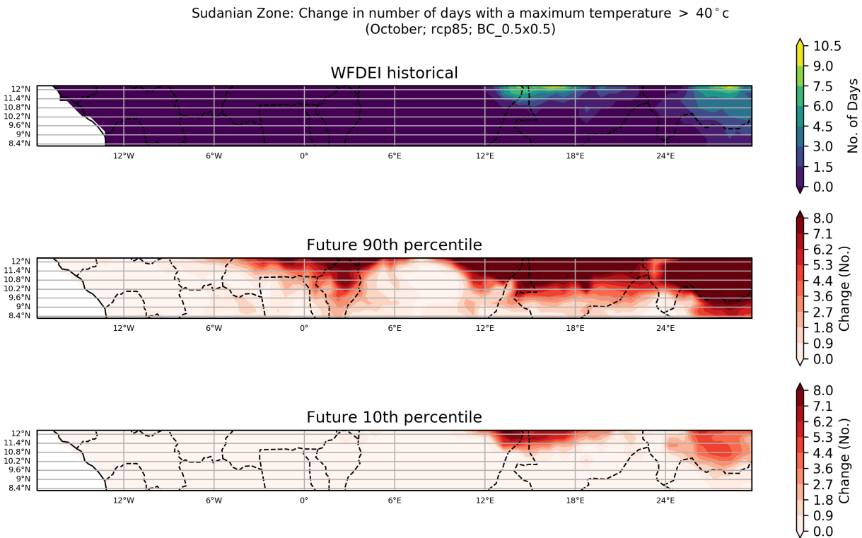
Figure 68: These maps show the ensemble spread in the absolute change in Number of Days with a Maximum Temperature > 40^{\circ}\text{C} for the period 2040 to 2059 (compared to a baseline period of 1950 - 2000) for the October season. They show the 90th and 10th percentiles of the distribution across the model ensemble, computed separately at each grid point, for the Sudanian Zone region. This particular plot shows the absolute change for the RCP8.5 scenario.
