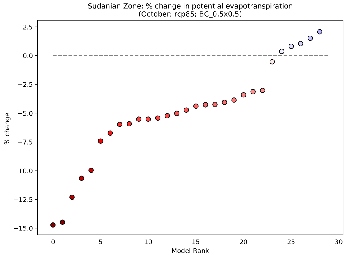
Figure 4: This scatterplot shows the percentage change in Potential Evapotranspiration for the period 2040 to 2059 (compared to a baseline period of 1950 - 2000) for the October season. Each data point shows an individual model averaged over Sudanian Zone, and ranked according to the magnitude of the value on the y-axis. This particular plot shows the percentage change for the RCP8.5 scenario.
