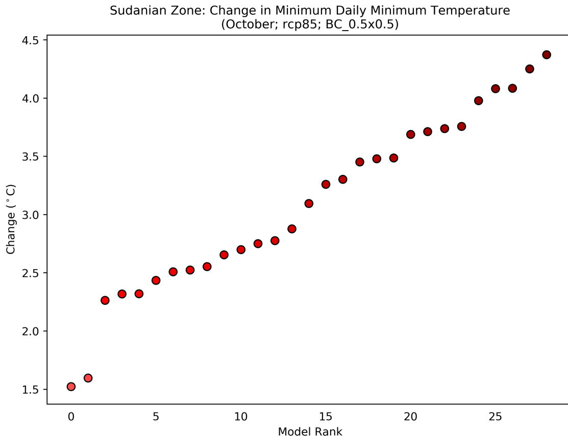
Figure 40: This scatterplot shows the absolute change in Minimum Daily Minimum Temperature for the period 2040 to 2059 (compared to a baseline period of 1950 - 2000) for the October season. Each data point shows an individual model averaged over Sudanian Zone, and ranked according to the magnitude of the value on the y-axis. This particular plot shows the absolute change for the RCP8.5 scenario.
