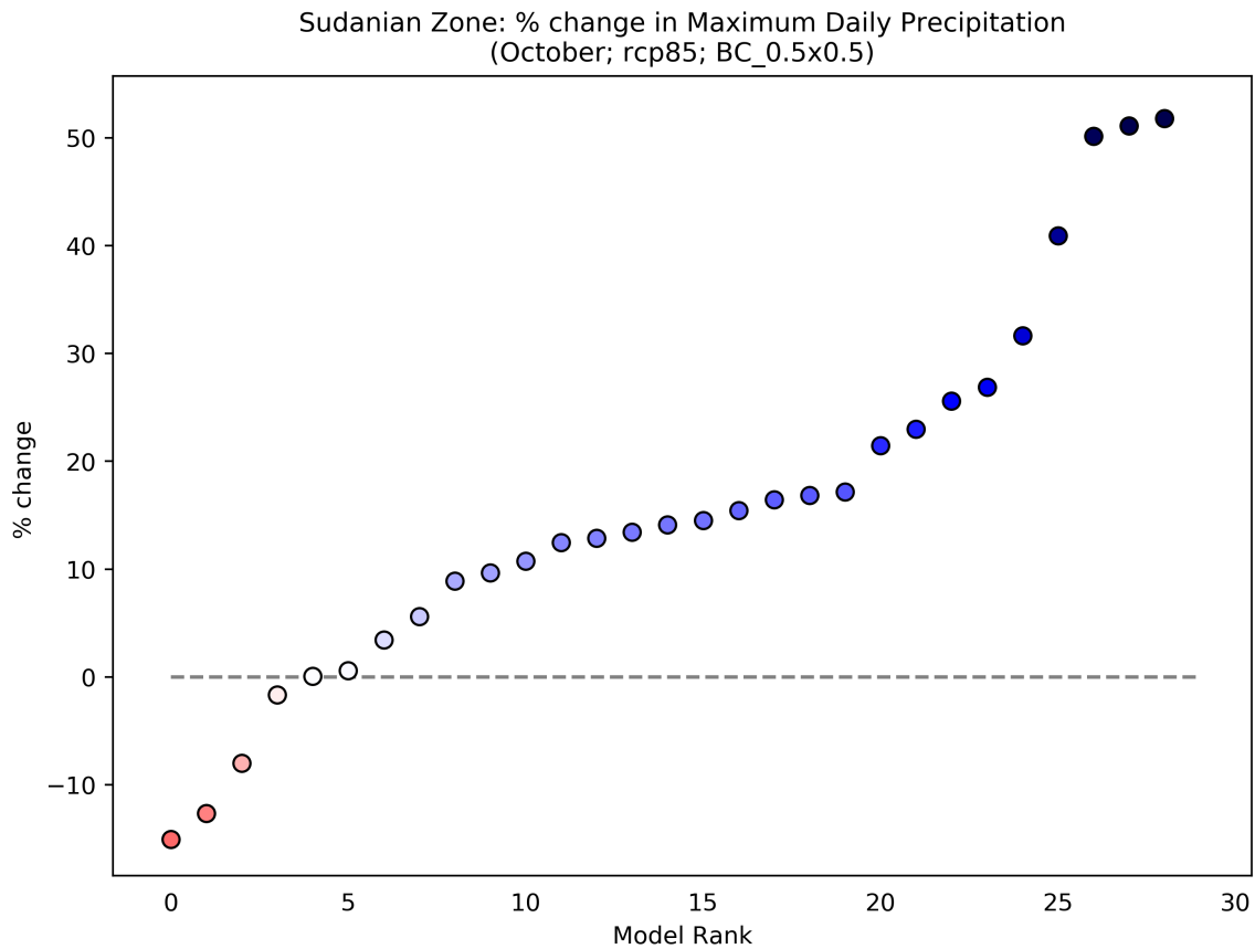
Figure 28: This scatterplot shows the percentage change in Maximum Daily Precipitation for the period 2040 to 2059 (compared to a baseline period of 1950 - 2000) for the October season. Each data point shows an individual model averaged over Sudanian Zone, and ranked according to the magnitude of the value on the y-axis. This particular plot shows the percentage change for the RCP8.5 scenario.
