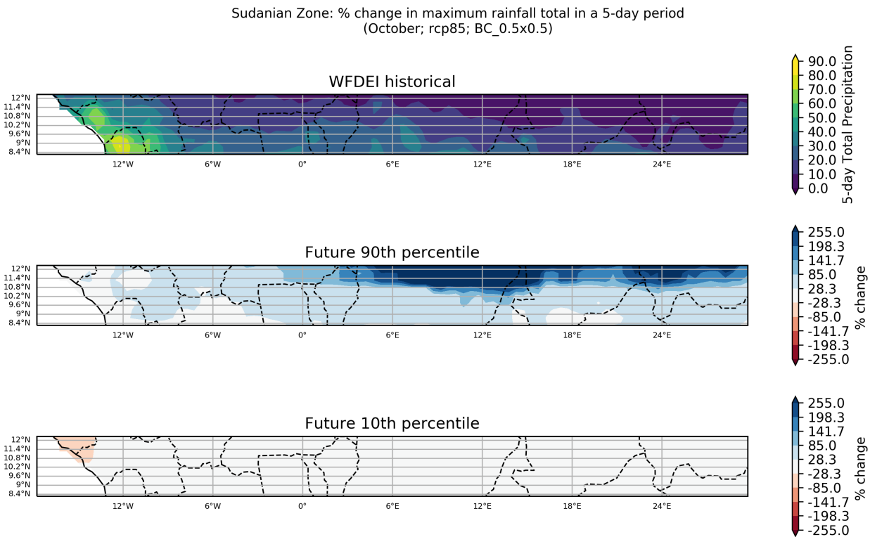
Figure 80: These maps show the ensemble spread in the percentage change in Maximum Rainfall Total in a 5-day Period for the period 2040 to 2059 (compared to a baseline period of 1950 - 2000) for the October season. They show the 90th and 10th percentiles of the distribution across the model ensemble, computed separately at each grid point, for the Sudanian Zone region. This particular plot shows the percentage change for the RCP8.5 scenario.
