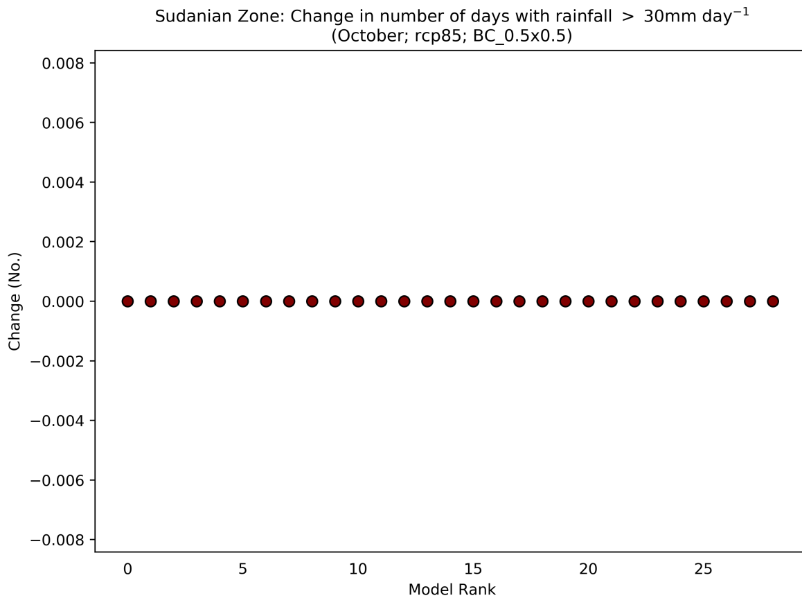
Figure 75: This scatterplot shows the absolute change in Number of Days with Rainfall > 30mm day -1 for the period 2040 to 2059 (compared to a baseline period of 1950 - 2000) for the October season. Each data point shows an individual model averaged over Sudanian Zone, and ranked according to the magnitude of the value on the y-axis. This particular plot shows the absolute change for the RCP8.5 scenario.
