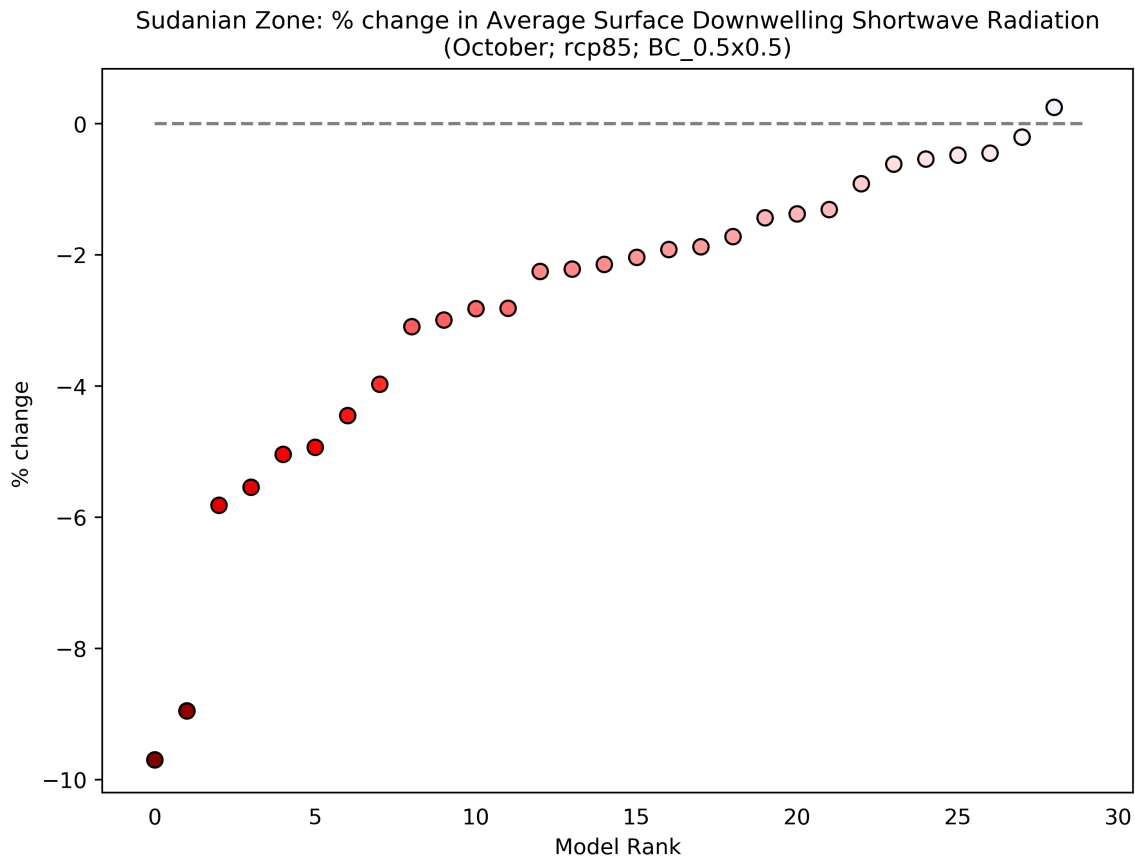
Figure 52: This scatterplot shows the percentage change in Average Surface Downwelling Shortwave Radiation for the period 2040 to 2059 (compared to a baseline period of 1950 - 2000) for the October season. Each data point shows an individual model averaged over Sudanian Zone, and ranked according to the magnitude of the value on the y-axis. This particular plot shows the percentage change for the RCP8.5 scenario.
