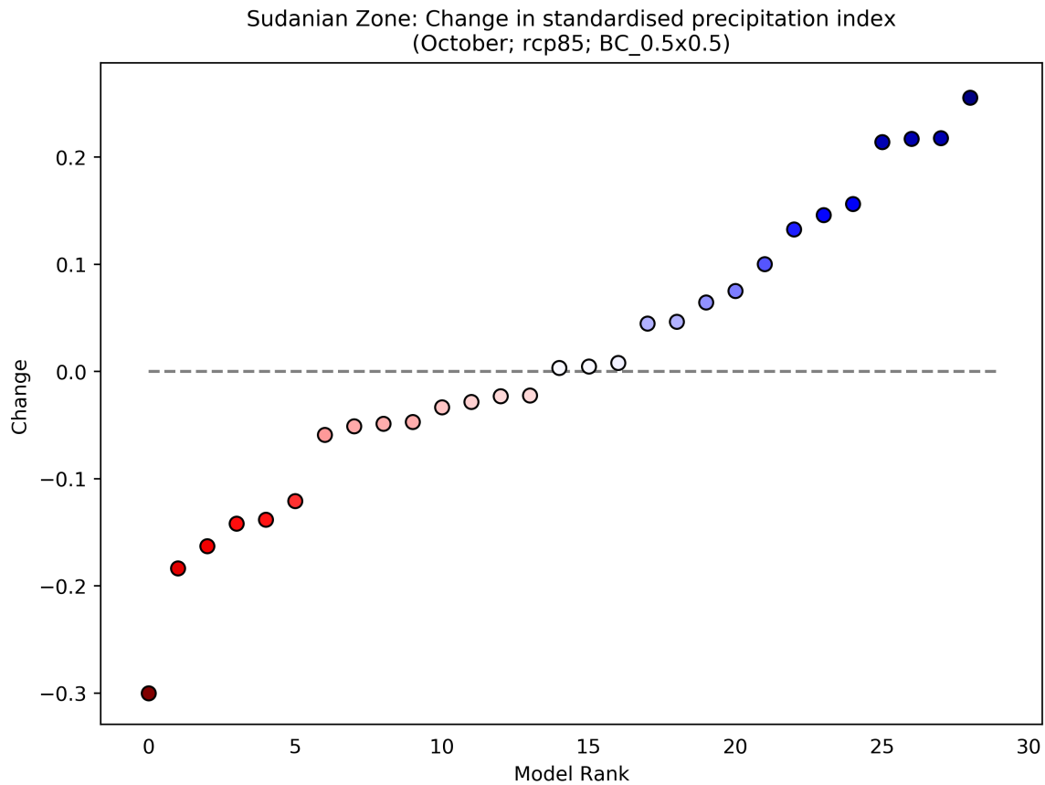
Figure 12: This scatterplot shows the absolute change in Standardised Precipitation Index for the period 2040 to 2059 (compared to a baseline period of 1950 - 2000) for the October season. Each data point shows an individual model averaged over Sudanian Zone, and ranked according to the magnitude of the value on the y-axis. This particular plot shows the absolute change for the RCP8.5 scenario.
