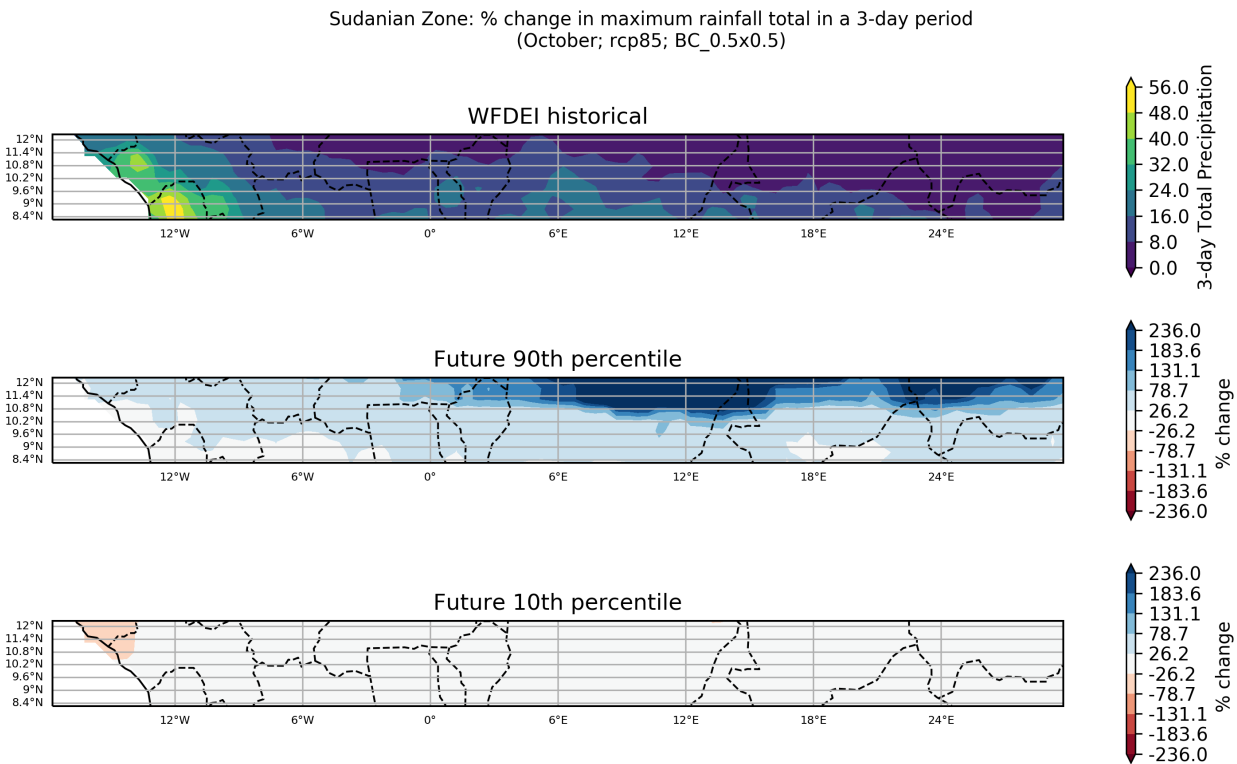
Figure 84: These maps show the ensemble spread in the percentage change in Maximum Rainfall Total in a 3-day Period for the period 2040 to 2059 (compared to a baseline period of 1950 - 2000) for the October season. They show the 90th and 10th percentiles of the distribution across the model ensemble, computed separately at each grid point, for the Sudanian Zone region. This particular plot shows the percentage change for the RCP8.5 scenario.
