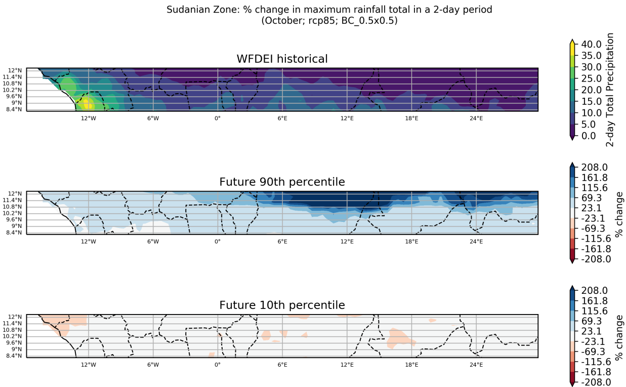
Figure 88: These maps show the ensemble spread in the percentage change in Maximum Rainfall Total in a 2-day Period for the period 2040 to 2059 (compared to a baseline period of 1950 - 2000) for the October season. They show the 90th and 10th percentiles of the distribution across the model ensemble, computed separately at each grid point, for the Sudanian Zone region. This particular plot shows the percentage change for the RCP8.5 scenario.
