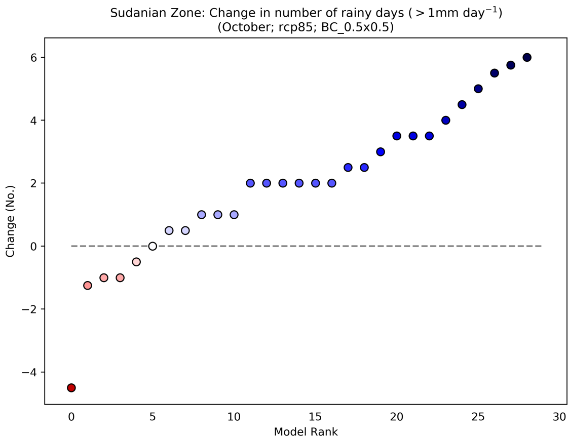
Figure 67: This scatterplot shows the absolute change in Number of Rainy Days ( >1\text{mm day}^{-1} ) for the period 2040 to 2059 (compared to a baseline period of 1950 - 2000) for the October season. Each data point shows an individual model averaged over Sudanian Zone, and ranked according to the magnitude of the value on the y-axis. This particular plot shows the absolute change for the RCP8.5 scenario.
