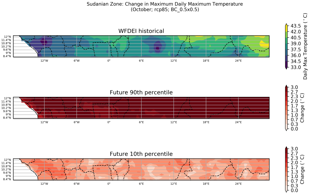
Figure 29: These maps show the ensemble spread in the absolute change in Maximum Daily Maximum Temperature for the period 2040 to 2059 (compared to a baseline period of 1950 - 2000) for the October season. They show the 90th and 10th percentiles of the distribution across the model ensemble, computed separately at each grid point, for the Sudanian Zone region. This particular plot shows the absolute change for the RCP8.5 scenario.
