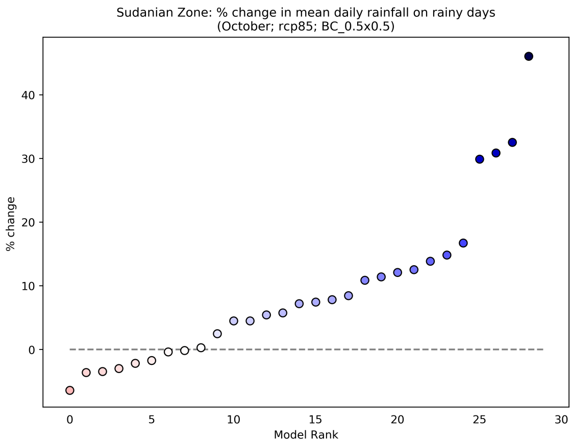
Figure 56: This scatterplot shows the percentage change in Mean Daily Rainfall on Rainy Days for the period 2040 to 2059 (compared to a baseline period of 1950 - 2000) for the October season. Each data point shows an individual model averaged over Sudanian Zone, and ranked according to the magnitude of the value on the y-axis. This particular plot shows the percentage change for the RCP8.5 scenario.
