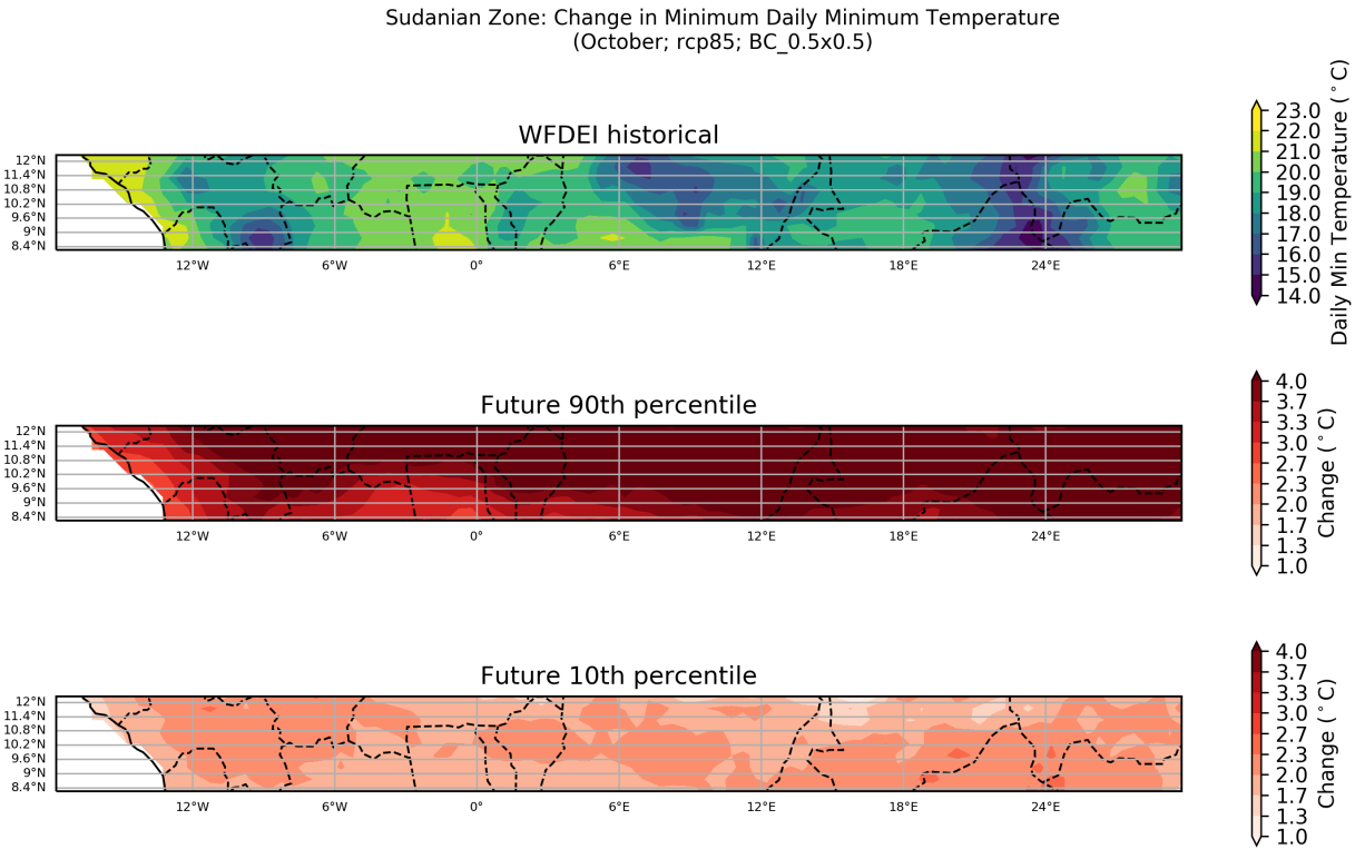
Figure 37: These maps show the ensemble spread in the absolute change in Minimum Daily Minimum Temperature for the period 2040 to 2059 (compared to a baseline period of 1950 - 2000) for the October season. They show the 90th and 10th percentiles of the distribution across the model ensemble, computed separately at each grid point, for the Sudanian Zone region. This particular plot shows the absolute change for the RCP8.5 scenario.
