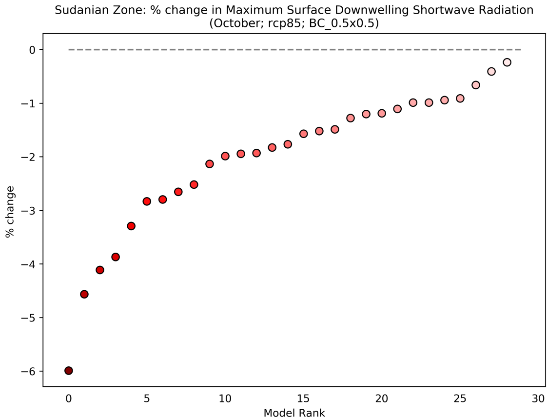
Figure 36: This scatterplot shows the percentage change in Maximum Surface Downwelling Shortwave Radiation for the period 2040 to 2059 (compared to a baseline period of 1950 - 2000) for the October season. Each data point shows an individual model averaged over Sudanian Zone, and ranked according to the magnitude of the value on the y-axis. This particular plot shows the percentage change for the RCP8.5 scenario.
