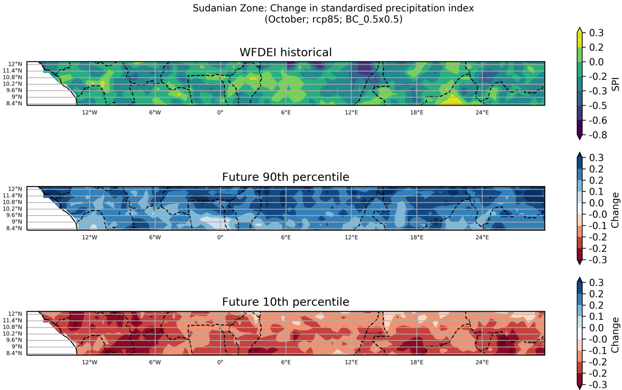
Figure 9: These maps show the ensemble spread in the absolute change in Standardised Precipitation Index for the period 2040 to 2059 (compared to a baseline period of 1950 - 2000) for the October season. They show the 90th and 10th percentiles of the distribution across the model ensemble, computed separately at each grid point, for the Sudanian Zone region. This particular plot shows the absolute change for the RCP8.5 scenario.
