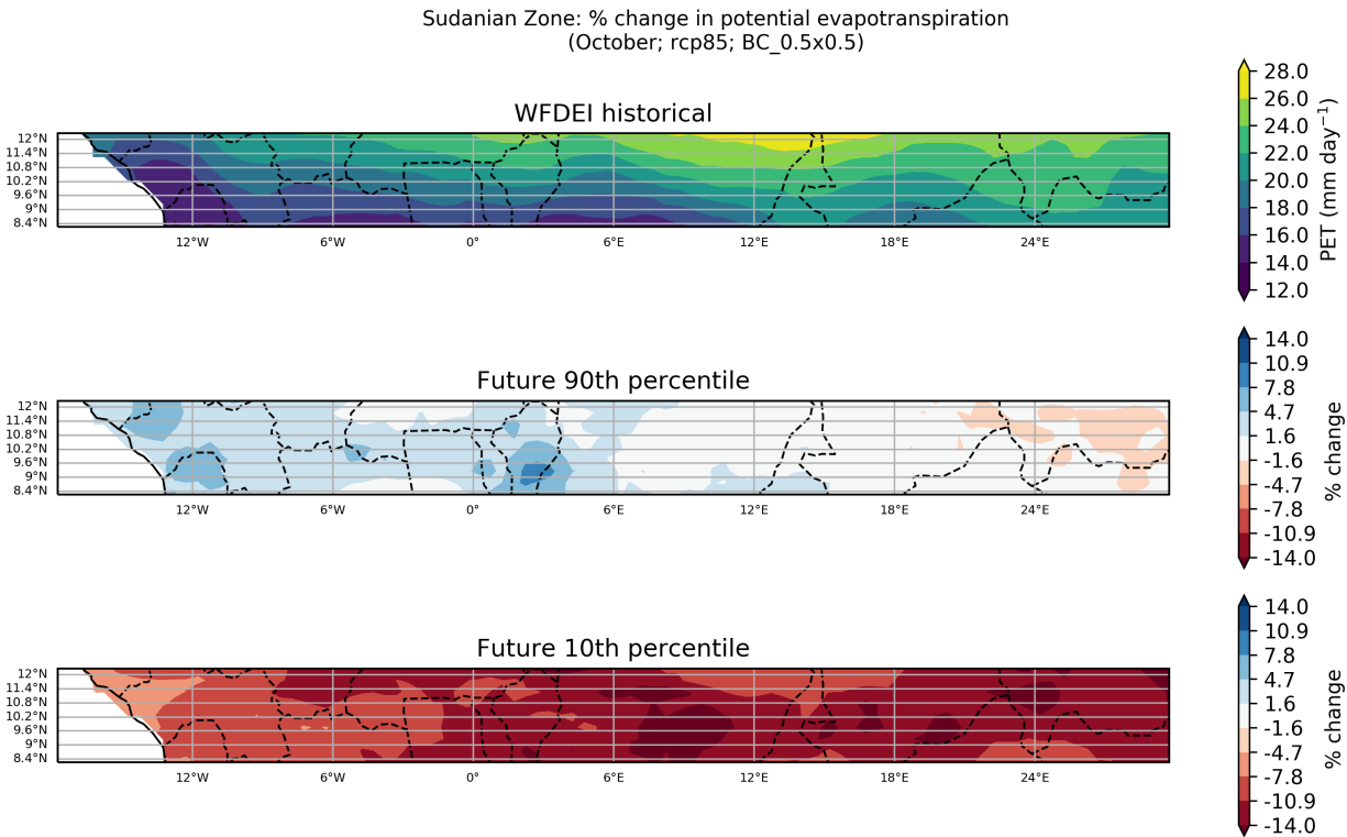
Figure 1: These maps show the ensemble spread in the percentage change in Potential Evapotranspiration for the period 2040 to 2059 (compared to a baseline period of 1950 - 2000) for the October season. They show the 90th and 10th percentiles of the distribution across the model ensemble, computed separately at each grid point, for the Sudanian Zone region. This particular plot shows the percentage change for the RCP8.5 scenario.
