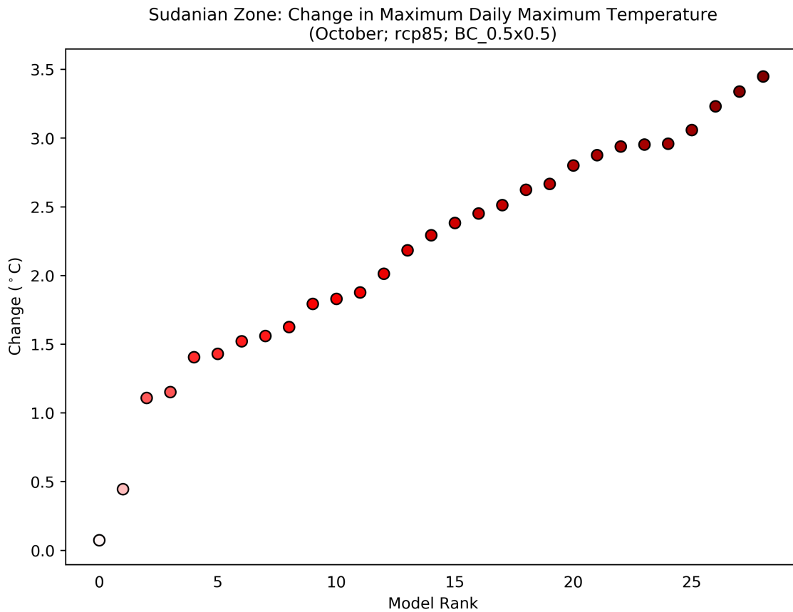
Figure 32: This scatterplot shows the absolute change in Maximum Daily Maximum Temperature for the period 2040 to 2059 (compared to a baseline period of 1950 - 2000) for the October season. Each data point shows an individual model averaged over Sudanian Zone, and ranked according to the magnitude of the value on the y-axis. This particular plot shows the absolute change for the RCP8.5 scenario.
