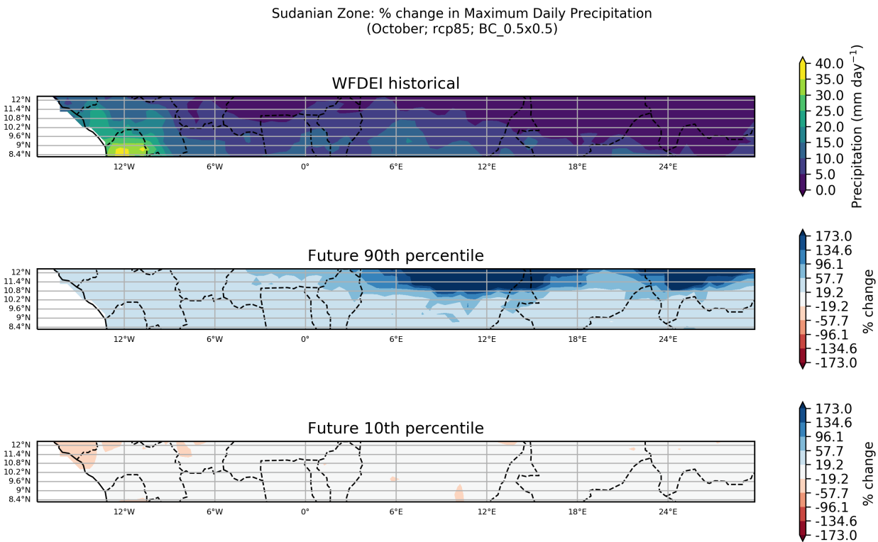
Figure 25: These maps show the ensemble spread in the percentage change in Maximum Daily Precipitation for the period 2040 to 2059 (compared to a baseline period of 1950 - 2000) for the October season. They show the 90th and 10th percentiles of the distribution across the model ensemble, computed separately at each grid point, for the Sudanian Zone region. This particular plot shows the percentage change for the RCP8.5 scenario.
