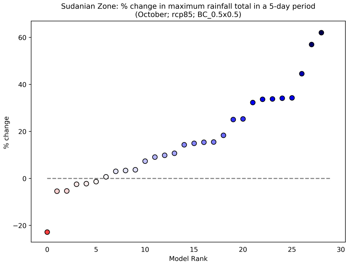
Figure 83: This scatterplot shows the percentage change in Maximum Rainfall Total in a 5-day Period for the period 2040 to 2059 (compared to a baseline period of 1950 - 2000) for the October season. Each data point shows an individual model averaged over Sudanian Zone, and ranked according to the magnitude of the value on the y-axis. This particular plot shows the percentage change for the RCP8.5 scenario.
