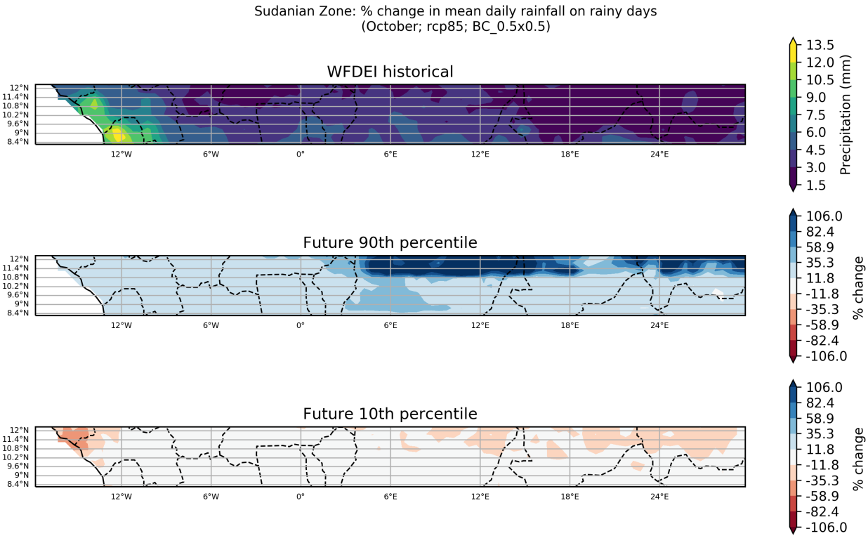
Figure 53: These maps show the ensemble spread in the percentage change in Mean Daily Rainfall on Rainy Days for the period 2040 to 2059 (compared to a baseline period of 1950 - 2000) for the October season. They show the 90th and 10th percentiles of the distribution across the model ensemble, computed separately at each grid point, for the Sudanian Zone region. This particular plot shows the percentage change for the RCP8.5 scenario.
