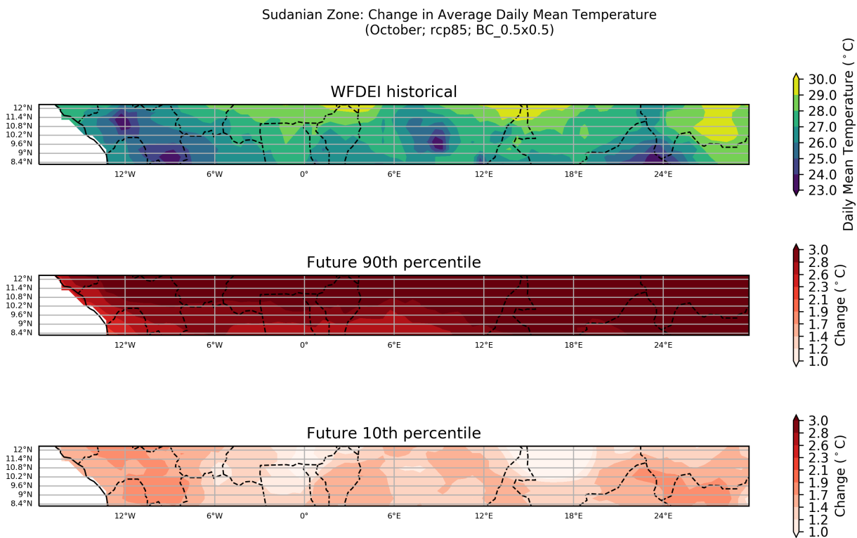
Figure 45: These maps show the ensemble spread in the absolute change in Average Daily Mean Temperature for the period 2040 to 2059 (compared to a baseline period of 1950 - 2000) for the October season. They show the 90th and 10th percentiles of the distribution across the model ensemble, computed separately at each grid point, for the Sudanian Zone region. This particular plot shows the absolute change for the RCP8.5 scenario.
