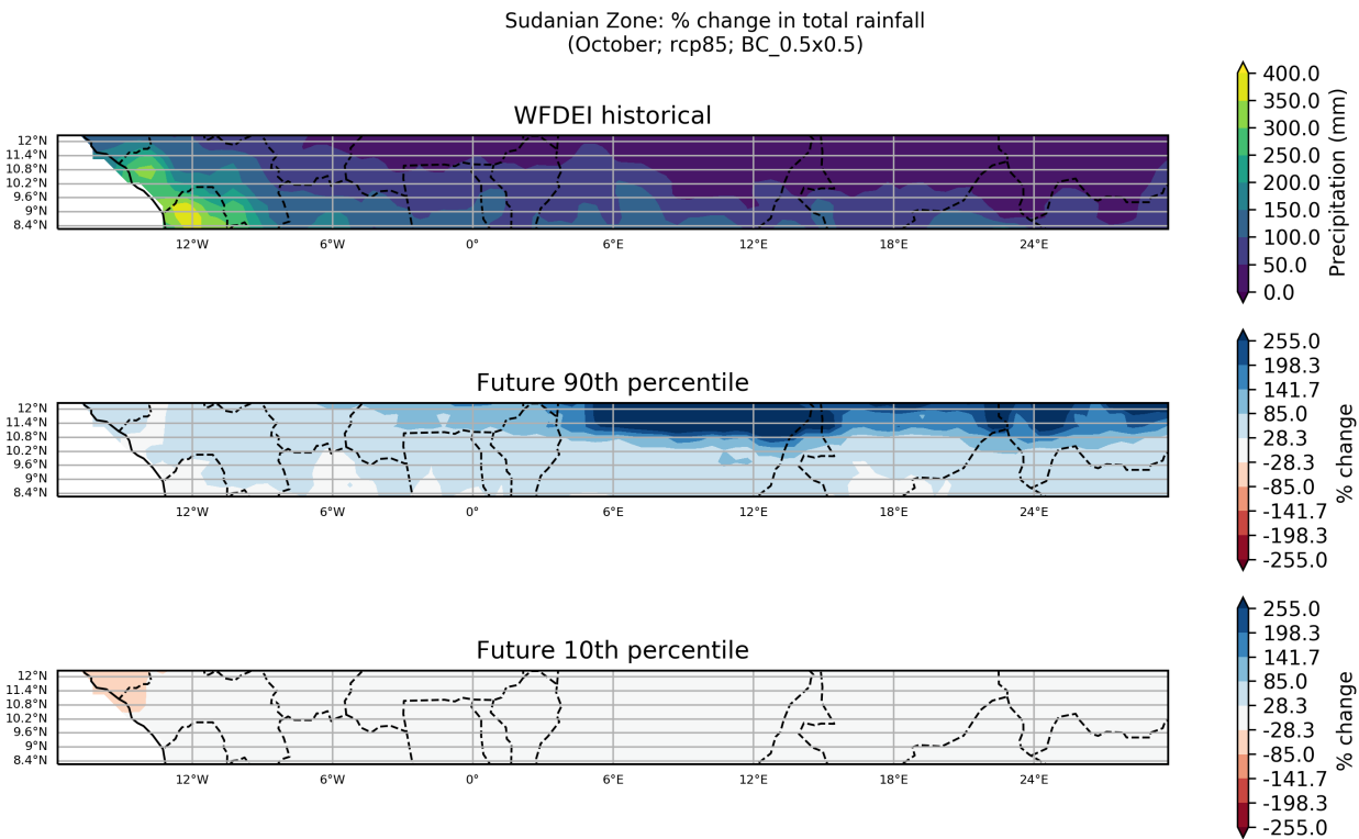
Figure 41: These maps show the ensemble spread in the percentage change in Total Rainfall for the period 2040 to 2059 (compared to a baseline period of 1950 - 2000) for the October season. They show the 90th and 10th percentiles of the distribution across the model ensemble, computed separately at each grid point, for the Sudanian Zone region. This particular plot shows the percentage change for the RCP8.5 scenario.
