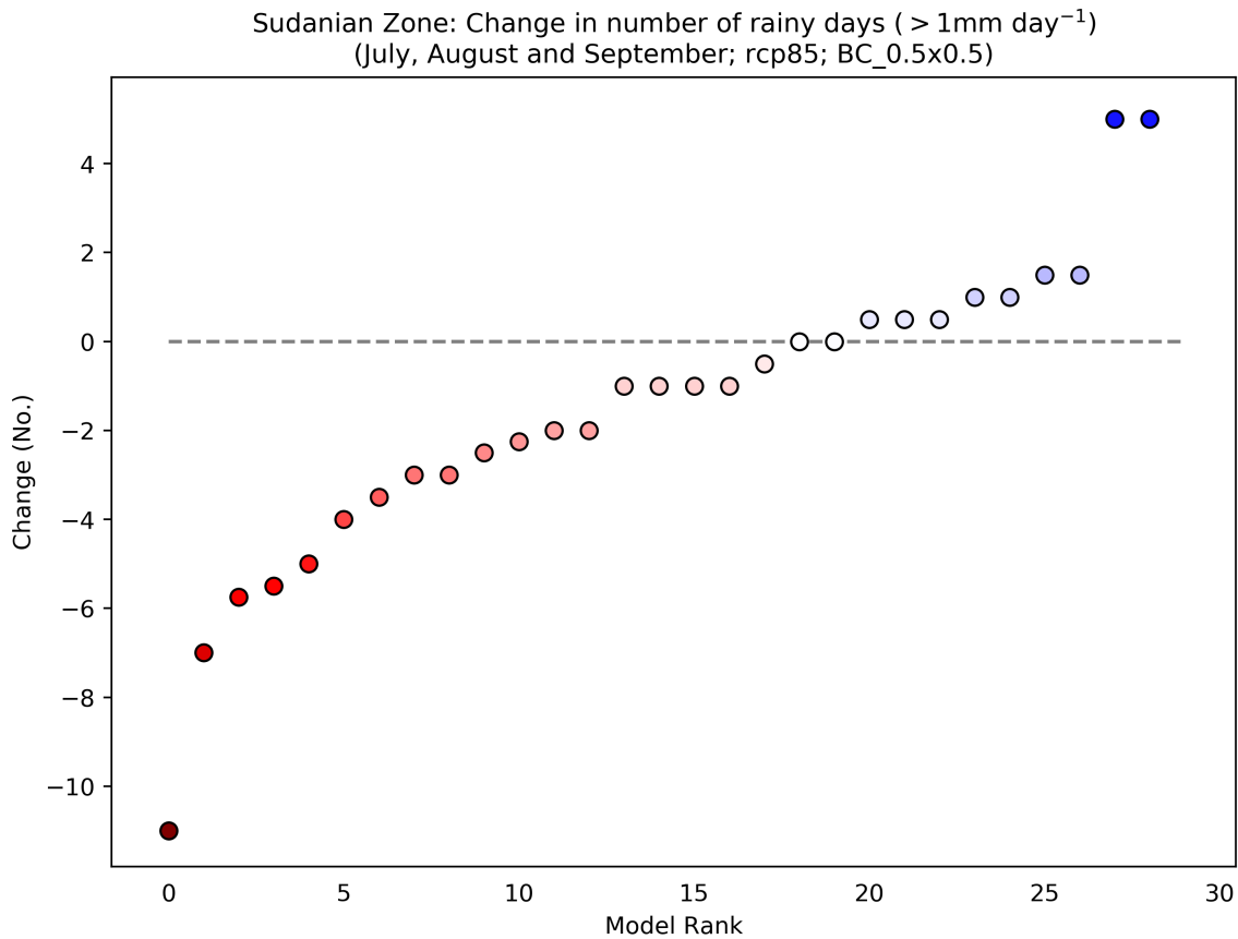
Figure 67: This scatterplot shows the absolute change in Number of Rainy Days ( > 1\text{mm day}^{-1} ) for the period 2040 to 2059 (compared to a baseline period of 1950 - 2000) for the July, August and September season. Each data point shows an individual model averaged over Sudanian Zone, and ranked according to the magnitude of the value on the y-axis. This particular plot shows the absolute change for the RCP8.5 scenario.
