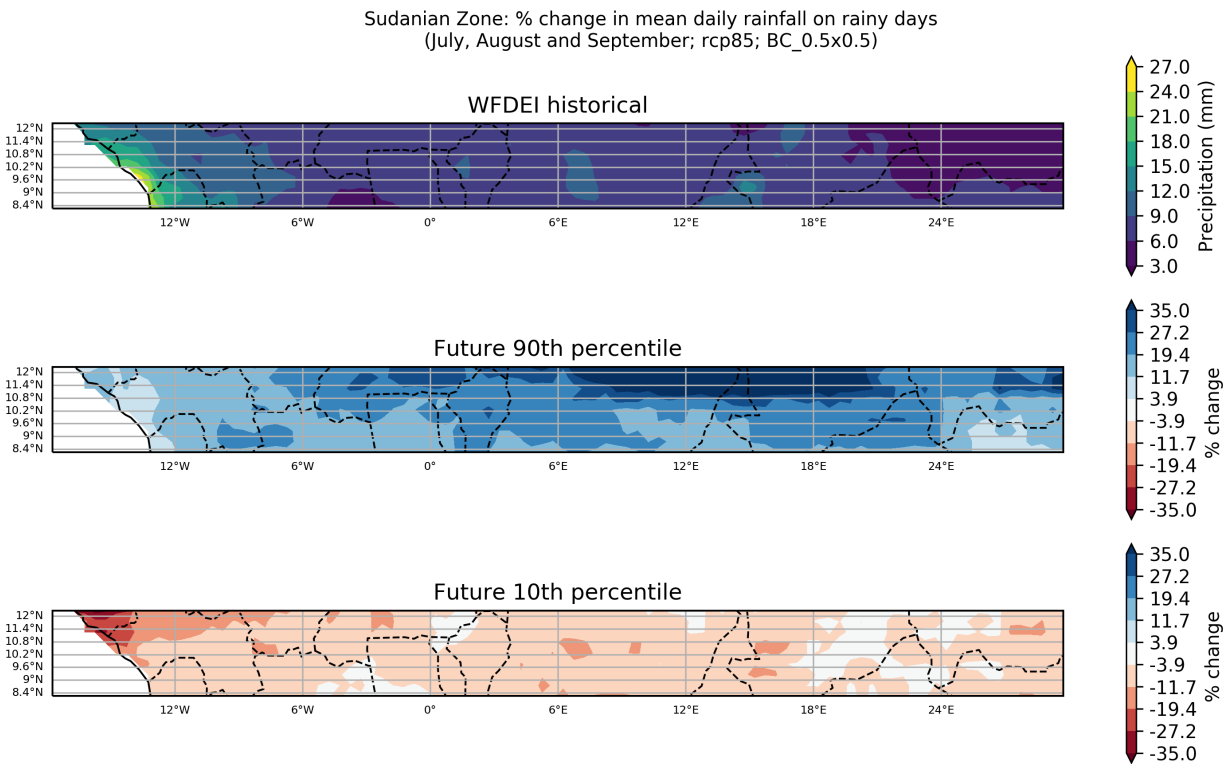
Figure 53: These maps show the ensemble spread in the percentage change in Mean Daily Rainfall on Rainy Days for the period 2040 to 2059 (compared to a baseline period of 1950 - 2000) for the July, August and September season. They show the 90th and 10th percentiles of the distribution across the model ensemble, computed separately at each grid point, for the Sudanian Zone region. This particular plot shows the percentage change for the RCP8.5 scenario.
