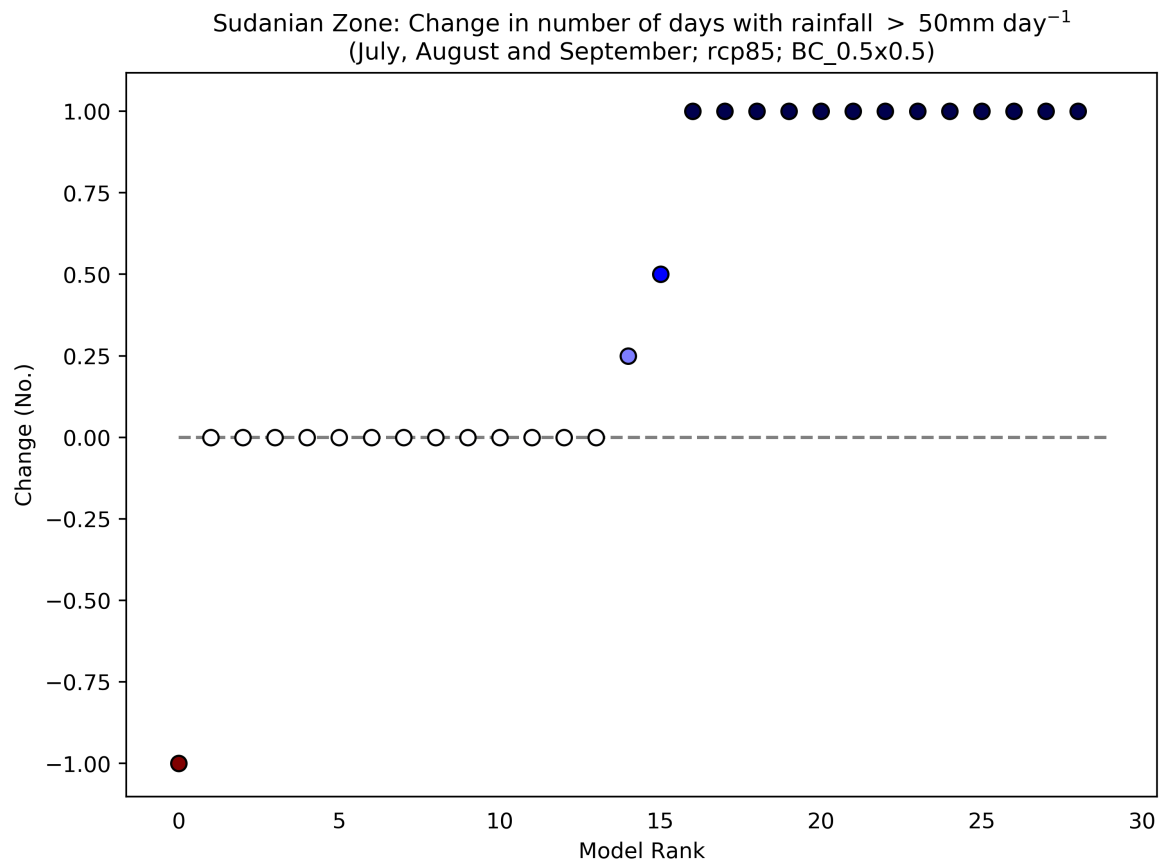
Figure 79: This scatterplot shows the absolute change in Number of Days with Rainfall > 50mm day -1 for the period 2040 to 2059 (compared to a baseline period of 1950 - 2000) for the July, August and September season. Each data point shows an individual model averaged over Sudanian Zone, and ranked according to the magnitude of the value on the y-axis. This particular plot shows the absolute change for the RCP8.5 scenario.
